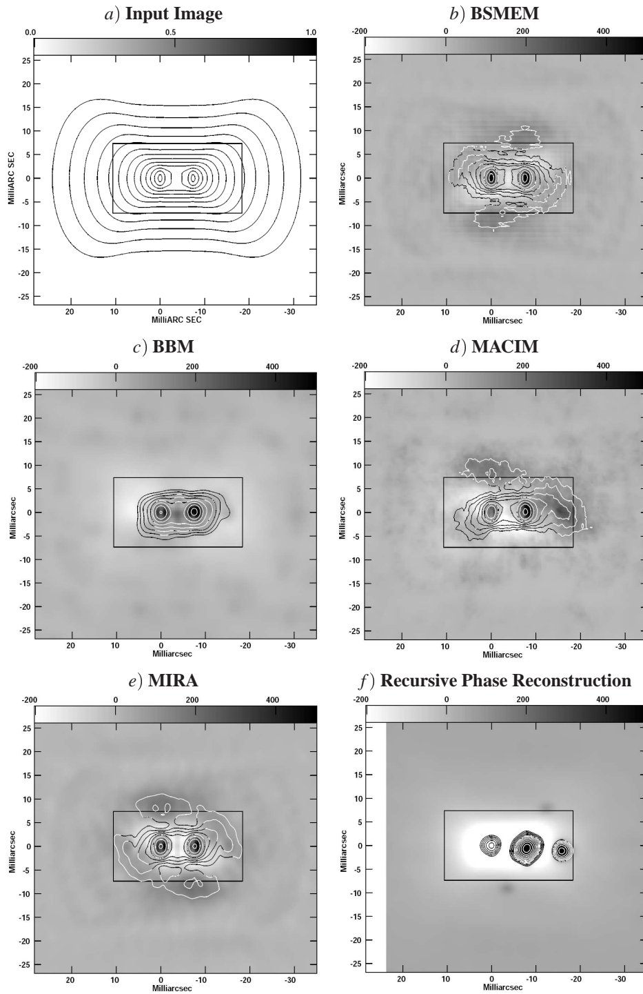
Figure 5.6: For the IAU imaging beauty contest 2006, a image of a optically thin disk had to be reconstructed (Figure a). Figures b to f depict the entry images by the contestants. Whereas the contours show the brightness distribution, the greyscale shows the residuals relative to the original image (Image Credit: Lawson et al. 2006 ).
