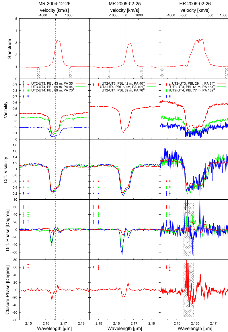
Figure 9.3: AMBER observables derived from our \eta Car data around the Bry line for three independent measurements ( Left : MR, 2004 December 26, Middle : MR, 2005 February 25, Right : HR, 2005 February 26). The first row shows the continuum-normalized spectra as extracted from the interferometric channels, followed by the derived calibrated visibilities and the differential visibilities. In the fourth and fifth row, the differential phase and the closure phase are presented. In the spectra we mark the wavelength regimes, which we defined as continuum for our analysis (shaded regions). The vertical grey line marks the rest-wavelength of Bry ( \lambda_{\text{vac}} = 2.1661 \mu\text{m} ; the small correction due to the system velocity of -8 \text{ km/s} (Smith 2004) has been neglected). We show different error bars within each panel: The left error bars correspond to the total (including statistical and systematic) error estimated for the continuum wavelength range, and the error bar towards the right visualizes the total error for the wavelength range within the line. For the HR 2005-02-26 measurement, data splitting showed that for a small wavelength range (hatched areas in the two lower right panels), the differential phase for the longest and middle baseline as well as the closure phase become very noisy and are therefore not reliable. Furthermore, the HR differential phase of the longest baseline is noisy at all wavelengths. See Sect. 9.3 for further details.
