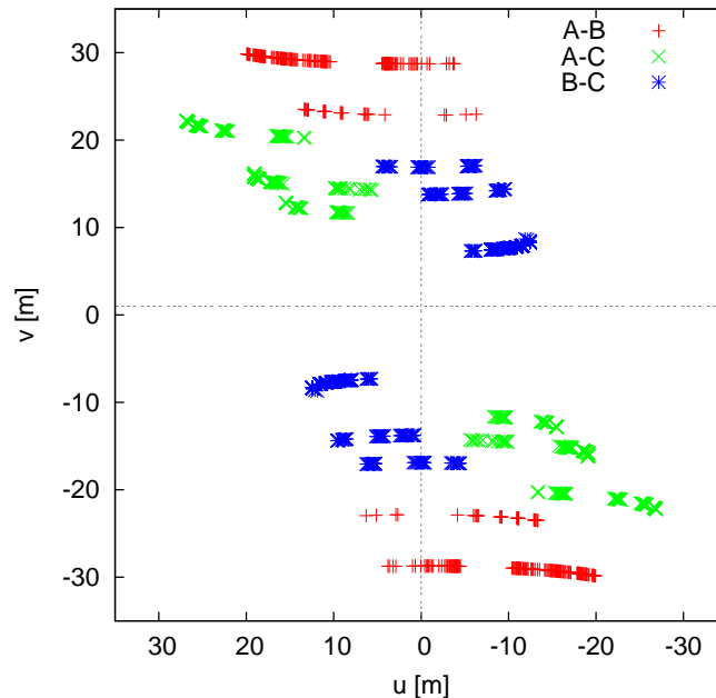
Figure 8.2: uv -plane coverage obtained on \theta^1 Ori C with the four IOTA array configurations used. The relatively strong asymmetry in the uv -plane coverage mainly results from the position of \theta^1 Ori C relatively close to the celestial equator.
