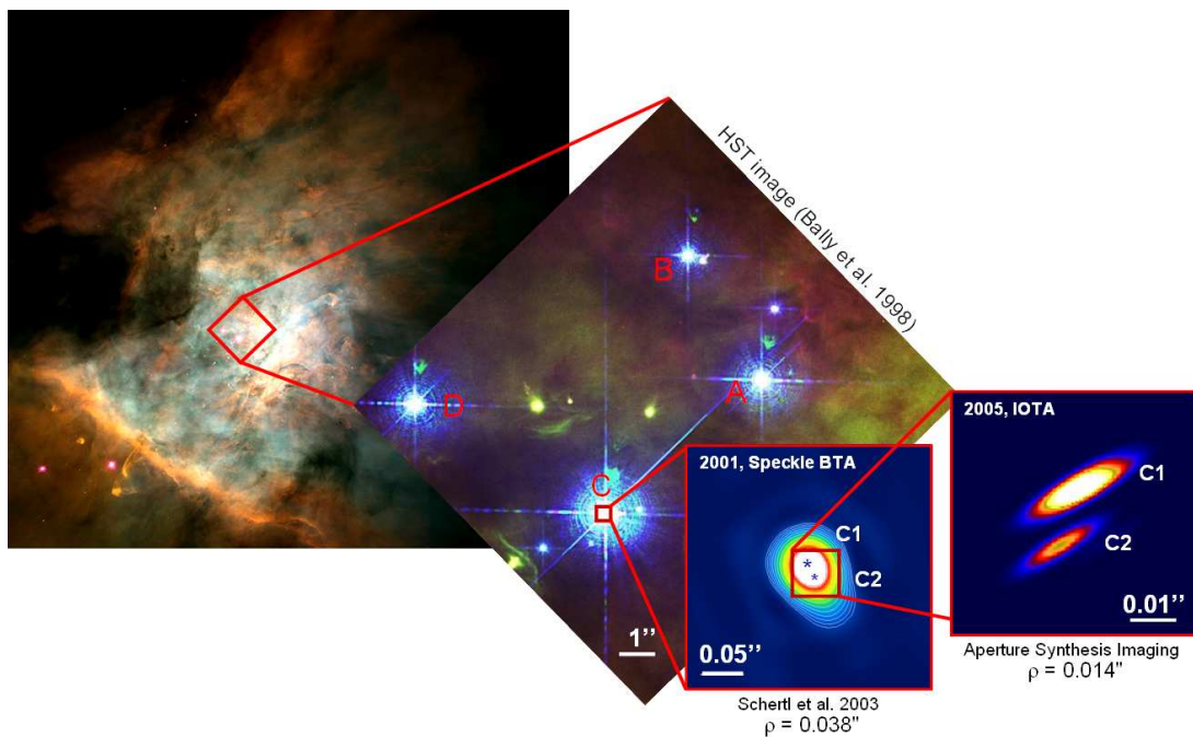
Figure 8.1: Mosaic zooming in from an HST image of the M42 H II region into the Trapezium cluster and the \theta^1 Ori C system, as seen with our speckle and IOTA imaging.
