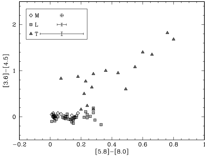
FIG. 4.—Similar to Fig. 3, except in this case we show the [3.6] - [4.5] vs. [5.8] - [8.0] color-color diagram for the same objects. [See the electronic edition of the Journal for a color version of this figure.]
