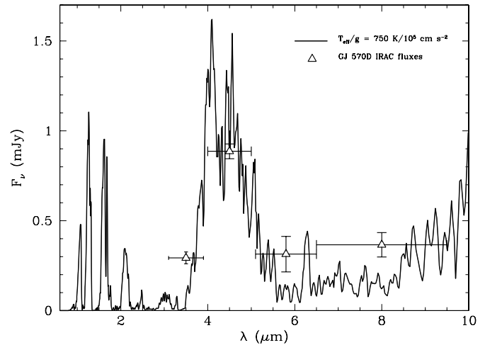
FIG. 14.—Comparison between a theoretical T dwarf spectral model with T_{\text{eff}}/g = 750 \text{ K}/10^5 \text{ cm s}^{-2} and the IRAC fluxes measured for the T7.5 dwarf GJ 570D. A distance of 5.89 pc has been assumed (Dahn et al. 2002). The triangles depict the fluxes (with their uncertainties) derived from the IRAC photometry; the horizontal lines indicate the widths of the IRAC bands. This model was generated for GJ 570D in 2002 to fit its optical spectrum shortward of 1.0 \mu\text{m} (Burrows et al. 2002). No further attempt was made to improve the fit. A slight ( \sim 40\% ) discrepancy in the 4.5 \mu\text{m} bandpass, attributable to a CO abundance excess in the atmosphere, is manifest. Despite this, this plot and Fig. 7 in Burrows et al. (2002) represent a good fit (that can nevertheless be improved) from 0.6 \mu\text{m} to \sim 8.0 \mu\text{m} and indicate that the IRAC data were successfully anticipated. [See the electronic edition of the Journal for a color version of this figure.]
