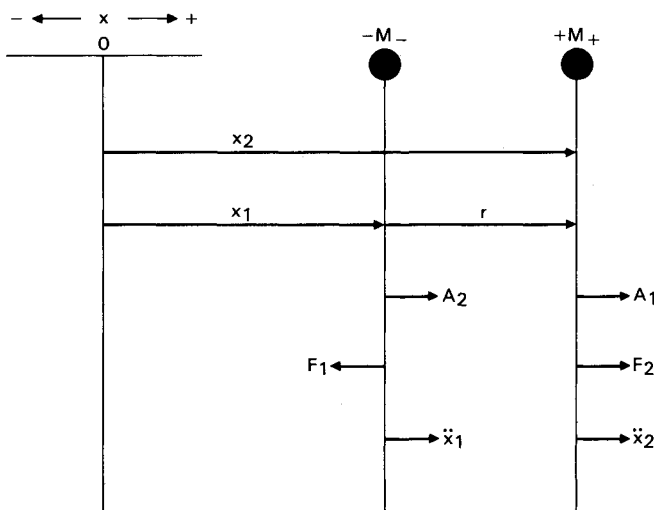
Fig. 4 Gravitational coupling of two opposite masses.
