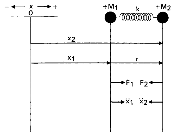
a) Two positive mass particles
