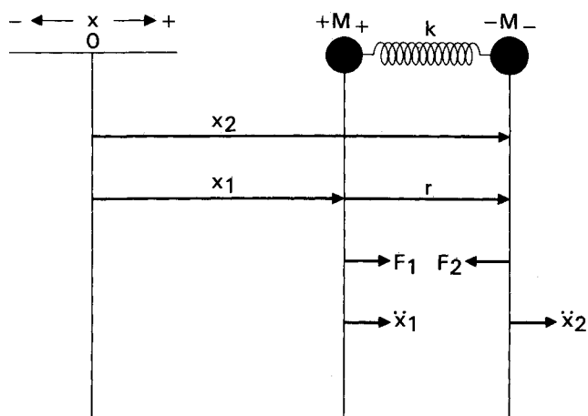
b) Two opposite mass particles
