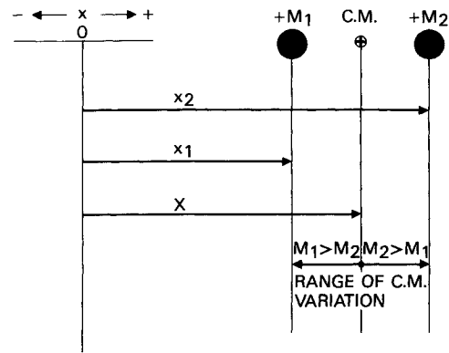
a) Two positive mass particles
