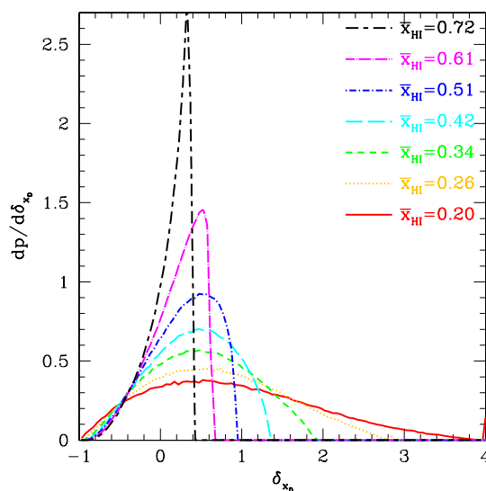
Figure 11.7 Probability distributions of the fractional bias in a simple damping wing estimator of the ionized bubble filling factor, \delta_{x_D} \equiv \bar{x}_D / (1 - Q_{\text{HII}}) - 1 . The different curves show different stages in reionization; all are computed with a semi-numerical simulation of reionization. Note that the mean is always non-zero, and the distribution becomes both wider and more biased as reionization progresses. Figure credit: Mesinger, A. & Furlanetto, S.R., Mon. Not. R. Astron. Soc. , 385 , 1348 (2008). Copyright 2008 by the Royal Astronomical Society.
