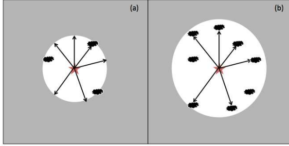
Figure 9.6 Illustration of the role of optically-thick regions (or LLSs) in reionization. These always exist due to the clumpiness of the IGM, but they only become important in the late phases of the process. (a) Early in reionization, when the ionized regions are small, most lines of sight intersect the edge of the ionized bubble rather than an LLS. Most ionizing photons therefore contribute to increasing the filling factor of ionized gas, and LLSs play only a minor role in slowing the process during its early phases. (b) However, once the bubble size grows larger than the mean separation of LLSs, most ionizing photons are absorbed by these objects rather than growing the ionized bubbles. The embedded sources therefore no longer contribute to reionization – and, so far as they are concerned the process is over locally , even if other regions remain largely neutral.
