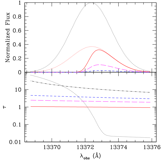
Figure 11.13 Top : Example line profiles for a galaxy at z = 10 . The upper dotted curve shows the intrinsic line profile, assumed to be a Gaussian with standard deviation 27 \text{ km s}^{-1} . The solid, long-dashed, and short-dashed curves show the observed line after reprocessing through the IGM; they place the galaxy in ionized bubbles with radii R_b = 10 , 5, and 3 comoving Mpc, respectively. The lower dotted curve shows the line if we neglect resonant absorption within the ionized bubble, assuming R_b = 10 Mpc. Bottom : The dotted line shows the resonant absorption from the ionized bubble. The solid, long-dashed, short-dashed, and dot-dashed curves show the damping wing optical depth for R_b = 10 , 5, 3, and 1 Mpc, respectively. Figure credit: Furlanetto, S.R. et al., Mon. Not. R. Astron. Soc. , 354 , 695 (2004). Copyright 2004 by the Royal Astronomical Society.
