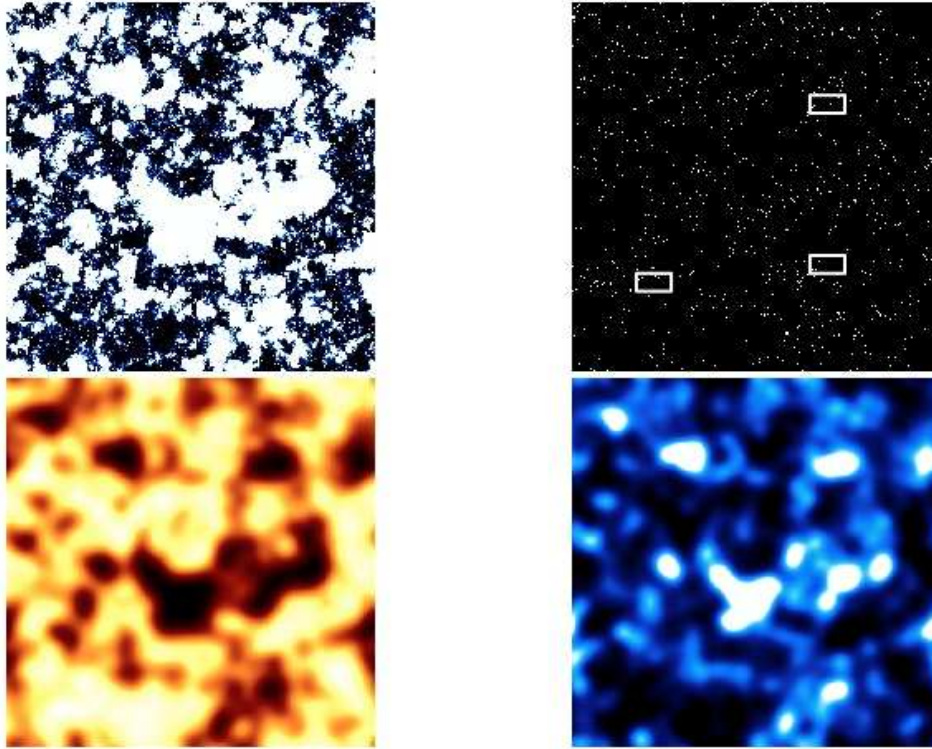
Figure 13.11 Schematic illustration of the cross-correlation between the spin-flip background and galaxy probes (see Color Plate 32 for a color version of this figure). Each panel shows a slice from a numerical simulation \sim 185 Mpc across. Upper left : Map of the ionized fraction midway through reionization (ionized regions are shown in white). Upper right : Map of the galaxy field. White squares show regions \sim 4 \times 8 arcmin across; these are each equivalent to four adjacent pointings of the James Webb Space Telescope. Lower left : Spin-flip background from this slice. Lower right : Galaxy map smoothed over 6 arcmin beam, as might be observed in an intensity mapping measurement. Note the strong large-scale anti-correlation between the bottom two figures. Figure credit: A. Lidz.
