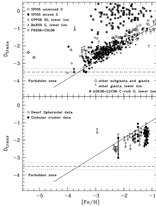
Figure 13.12 Measure of the carbon and oxygen abundance for metal-poor stars, D_{\text{trans}} \equiv \log_{10} (10^{[C/H]} + 0.3 \times 10^{[O/H]}) , as a function of the iron abundance relative to hydrogen, [Fe/H] . Top panel : Galactic halo stars. Bottom panel : Stars in dwarf spheroidal galaxies and globular clusters. G and SG indicate giants and subgiants. The critical limit marked with a dashed line was predicted theoretically by comparing the cooling rate for carbon and oxygen lines to H_2 cooling (which controls the formation of massive Population III stars). Without metal line cooling, no low mass stars should be found below this line. The dotted lines define the uncertainty in the theoretical prediction without dust cooling. If dust cooling is added, the dashed line is lowered by \sim 2 orders of magnitude. Interestingly, all data points are well above the theoretical lines for metal and dust cooling so far. Figure credit: Frebel, A., Johnson, J. L., & Bromm, V., Mon. Not. R. Astron. Soc. 380 , L49 (2007). Copyright 2007 by the Royal Astronomical Society.
