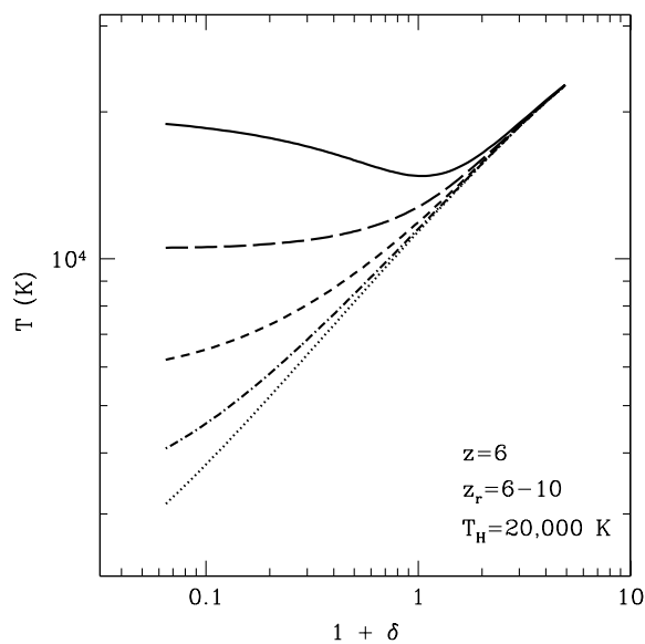
Figure 9.13 IGM temperature-density relation following H I reionization. All curves assume z = 6 and take a post-reionization temperature of T_H = 20,000 \text{ K} . The solid, long-dashed, short-dashed, dot-dashed, and dotted curves set the reionization redshift at z_r = 6, 7, 8, 9, and 10 , respectively. Figure credit: Furlanetto, S. R., & Oh, S. P., Astrophys. J. 701 , 94 (2009). Reproduced with permission of the American Astronomical Society.
