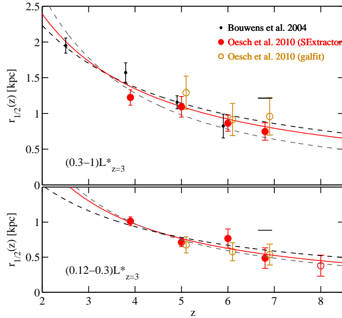
Figure 8.3 Observed evolution of the mean half-light radius of galaxies across the redshift range 2 < z < 8 in two bins of fixed intrinsic luminosity: (0.3-1)L_*(z = 3) (top) and (0.12-0.3)L_*(z = 3) (bottom), where L_*(z = 3) is the characteristic luminosity of a galaxy at z = 3 (equation 10.3). Different point types correspond to different methods of analysing the data. The dashed lines indicate the scaling expected for a fixed halo mass ( \propto (1+z)^{-1} ; black) or at fixed halo circular velocity ( \propto (1+z)^{-3/2} ; gray). The central solid lines correspond to the best-fit to the observed evolution described by \propto (1+z)^{-m} , with m = 1.12 \pm 0.17 for the brighter luminosity bin, and m = 1.32 \pm 0.52 at fainter luminosities. Figure credit: Oesch, P. A., et al., Astrophys. J. 709 , L21 (2010). Reproduced with permission of the American Astronomical Society.
