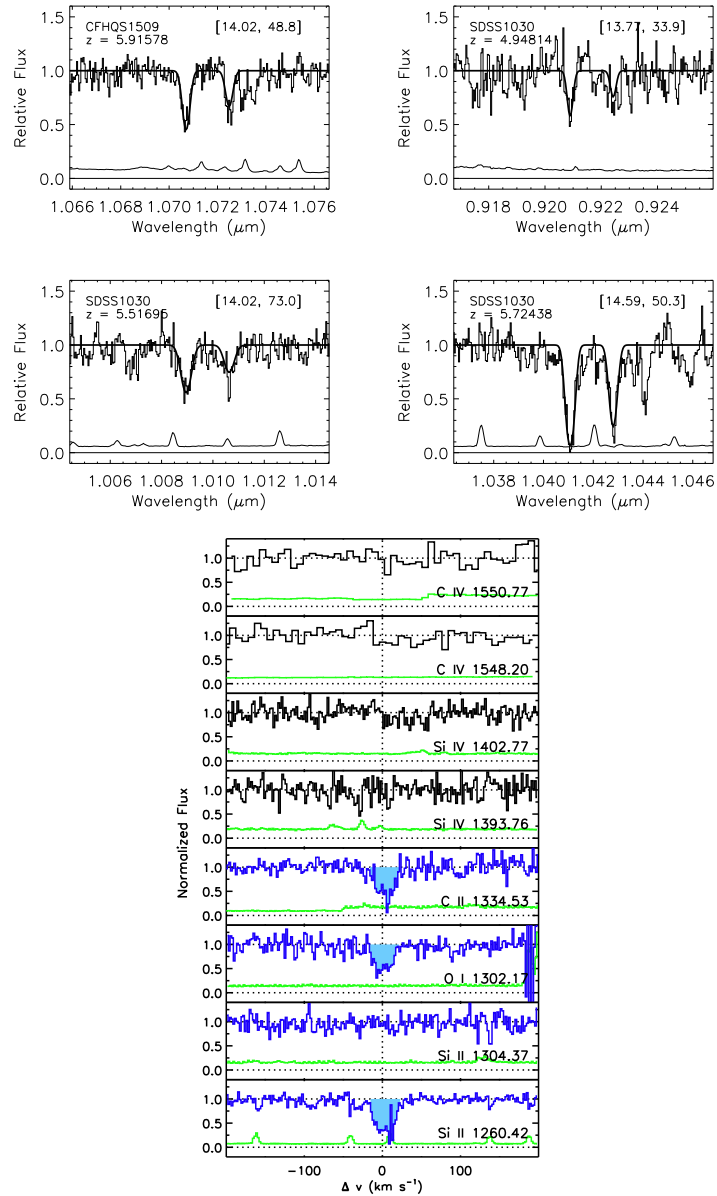
Figure 4.14 Examples of high- z metal absorption systems. Top : Several C IV doublets discovered with the Magellan Baade telescope. The upper histograms show the data; the lower histograms shows the errors. The solid curve in each panel is a Voigt profile fit to the two components of the doublet; the column density N_{\text{CIV}} and Doppler width b are listed in brackets in each panel. Bottom : An example low-ionization absorber at z = 5.8765 toward the quasar SDSS J0818+1722 discovered with the Keck telescope. The solid dark lines are the data; the errors are shown as the lower lines in each panel. Shaded regions represent detected transitions. The H I lines are completely saturated in both absorbers. Figure credit: Simcoe, R. A., Astrophys. J. 743 , 21 (2011, top panels); Becker, G. D., Astrophys. J. , submitted (2011), astro-ph/1101.4399 (bottom panels). Reproduced with permission of the American Astronomical Society.
