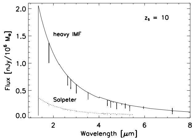
Figure 5.14 Comparison of the observed flux per unit frequency from a cluster of Population III stars at a redshift z_s = 10 for a Salpeter IMF ( dotted line ) and an IMF composed purely of very massive stars ( solid line ). The flux in units of nJy per 10^6 M_\odot of stars is plotted as a function of observed wavelength in \mu\text{m} . The cutoff below an observed wavelength of 1216 \text{ \AA} (1 + z_s) = 1.34 \mu\text{m} is due to hydrogen Lyman- \alpha absorption in the IGM (the so-called Gunn-Peterson effect; see §4.3). Figure credit: Bromm, V. Kudritzki, R. P. & Loeb, A. Astrophys. J. 552 , 464 (2001); Salpeter curve from Tumlinson, J., & Shull, M. J. Astrophys. J. 528 , L65 (2000). Reproduced with permission of the American Astronomical Society.
