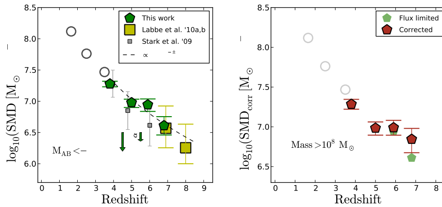
Figure 10.12 Stellar mass density (SMD) evolution over redshift in galaxies brighter than M_{AB} = -18 at a rest-frame wavelength of 1500 \text{ \AA} ( left ) and with stellar mass M_{*} > 10^8 M_{\odot} ( right ) from several different measurements. All panels assume a Salpeter IMF and Z = 0.2 Z_{\odot} ; the line labeled “Chabrier” shows the effect of assuming a different IMF. The other line (labeled “ H\alpha ”) shows the effect of systematic contamination from line emission. A minimum stellar density \sim 1.7 \times 10^6 f_{\text{esc}}^{-1} M_{\odot} \text{ Mpc}^{-3} of Population III stars (corresponding to \Omega_{*} \sim 1.25 \times 10^{-5} f_{\text{esc}}^{-1} ) is required to produce one ionizing photon per hydrogen atom. Figure credit: Gonzalez, V. et al. Astrophys. J. 735 , L34 (2011). Reproduced with permission of the American Astronomical Society.
