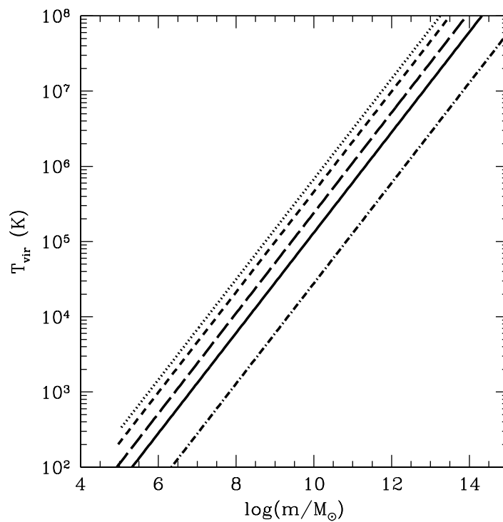
Figure 3.7 Virial temperature over a wide range of halo masses and redshifts (equation 3.30). The dotted, short-dashed, long-dashed, solid, and dot-dashed curves take z = 30, 20, 10, 5, and 0 , respectively. For simplicity we assume fully-ionized gas in all these halos, though the low-mass objects may actually accrete neutral gas.
