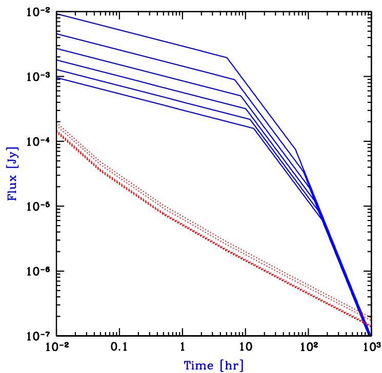
Figure 10.8 Detectability of high-redshift GRB afterglows as a function of time since the GRB explosion as measured by the observer. The GRB afterglow flux (in Jy) is shown at the redshifted Lyman- \alpha wavelength (solid curves). Also shown (dotted curves) is a crude estimate for the spectroscopic detection threshold of JWST , assuming an exposure time equal to 20% of the time since the GRB explosion. Each set of curves spans a sequence of redshifts: z = 5, 7, 9, 11, 13, 15 , respectively (from top to bottom). Figure credit: Barkana, R., & Loeb, A. Astrophys. J. 601 , 64 (2004). Reproduced with permission of the American Astronomical Society.
