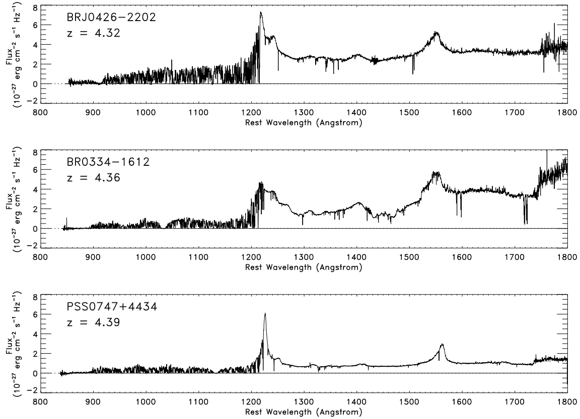
Figure 4.5 Example Lyman- \alpha forest spectra taken with the ESI spectrograph on the Keck Telescope. The highly variable absorption blueward of the Lyman- \alpha rest wavelength (at 1216 \text{\AA} ) is the Lyman- \alpha forest, not noise. Redward of this transition, the quasar continuum is visible, with only a few absorption features due to metal line absorbers in the IGM. Figure credit: Songaila, A. & Cowie, L., Astrophys. J. , 721 , 1448 (2011). Reproduced with permission of the American Astronomical Society.
