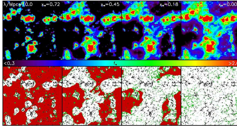
Figure 9.8 IGM absorbers in a “semi-numerical” simulation of reionization (see Color Plate 17 for a color version of this figure). In each panel, we set (by hand) the mean free path of ionizing photons to 10 comoving Mpc; the four columns show different H II fractions at a fixed redshift z = 10 . The upper panels show the ionizing flux (arbitrary normalization) inside ionized zones according to the colorscale. The lower panels show the locations of halos (dark points inside the white regions) and absorbers (green points). Figure credit: Crociani, D. et al., Mon. Not. R. Astron. Soc. , 411 , 289 (2011). Copyright 2011 by the Royal Astronomical Society.
