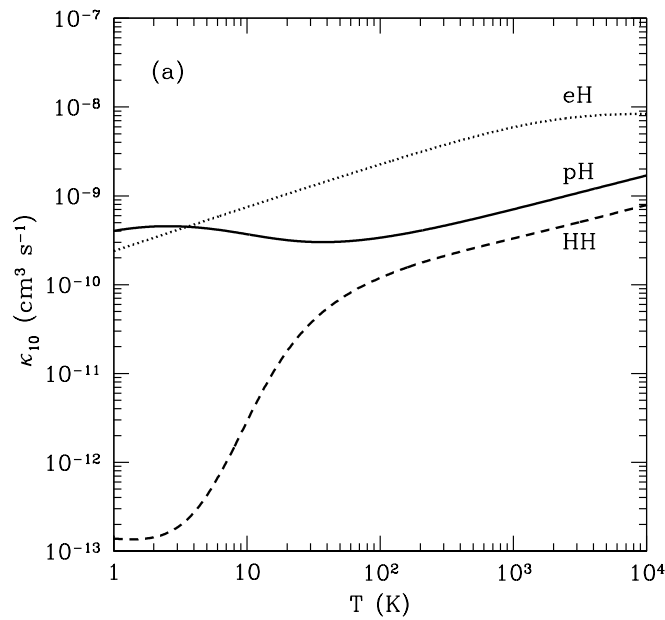
Figure 12.3 De-excitation rate coefficients for H-H collisions (dashed line), H-e - collisions (dotted line), and H-p collisions (solid line). Note that the net rates are also proportional to the densities of the individual species, so H-H collisions still dominate in a weakly-ionized medium. Figure credit: Furlanetto, S. R. & Furlanetto, M. R., Mon. Not. R. Astron. Soc. 379 , 130 (2007). Copyright 2007 by the Royal Astronomical Society.
