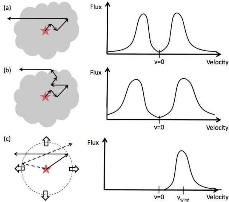
Figure 11.2 Schematic illustrations of the radiative transfer of Lyman- \alpha photons through a dust-free, homogeneous interstellar medium. (a) For a moderately optically thick cloud, a Lyman- \alpha photon undergoes a random walk until its frequency diffuses into the wings of the line, escaping once the optical depth \tau_\nu < 1 at the photon frequency \nu . This produces a double-peaked emission line and spatially compact emission. (b) For a very optically thick cloud, the photon may need to diffuse out of the cloud in space rather than frequency. In that case, the two peaks are substantially broader, and the emission is spatially extended. (c) If the scattering medium has a velocity gradient (here we imagine an expanding shell of gas), photons initially directed toward the observer are scattered away by the blueshifted near side of the shell. However, photons directed toward the far side of the shell that backscatter toward the observer pass through the near side of the shell far out of resonance and escape toward the observer. The result is a single emission line centered on the velocity of the far side of the shell.
