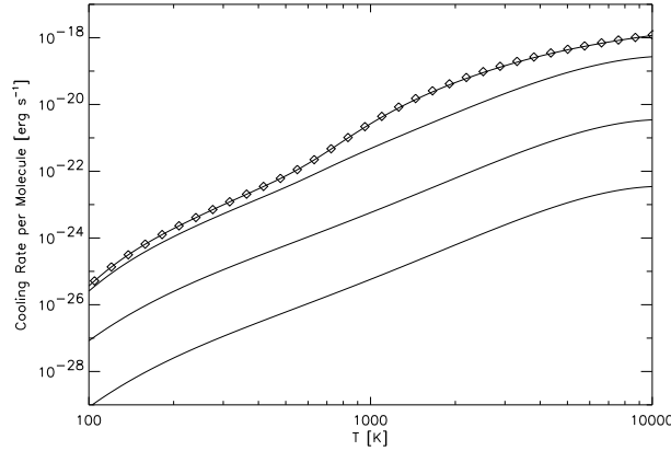
Figure 5.4 Cooling rate from \text{H}_2 per molecule. The solid lines show n = 10^{-1}, 10^1, 10^3, and 10^5 \text{ cm}^{-3} , from bottom to top. The diamonds show the cooling rate in LTE; note how the cooling function approaches this limit when n > n_{\text{cr}} due to the transition to LTE. Figure credit: Bromm V., et al., Astrophys. J. , 564 , 23 (2002). Reproduced with permission of the American Astronomical Society.
