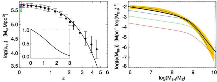
Figure 7.4 Left panel: the black hole mass density of quasars from the data (circles) and the best fit luminosity function (solid line). The inset shows the fraction of the mass density relative to today's value, \rho_{\text{BH}}(z)/\rho_{\text{BH}}(0) , on a linear scale. Right: the black hole mass function at z = 0 (thick black line) and z = 1, 2, 3 (from top to bottom). The shaded region shows the 1\sigma observational uncertainty. Figure credit: Hopkins, P. F., Richards, G. T., & Hernquist, L., Astrophys. J. 654 , 731 (2007). Reproduced with permission of the American Astronomical Society.
