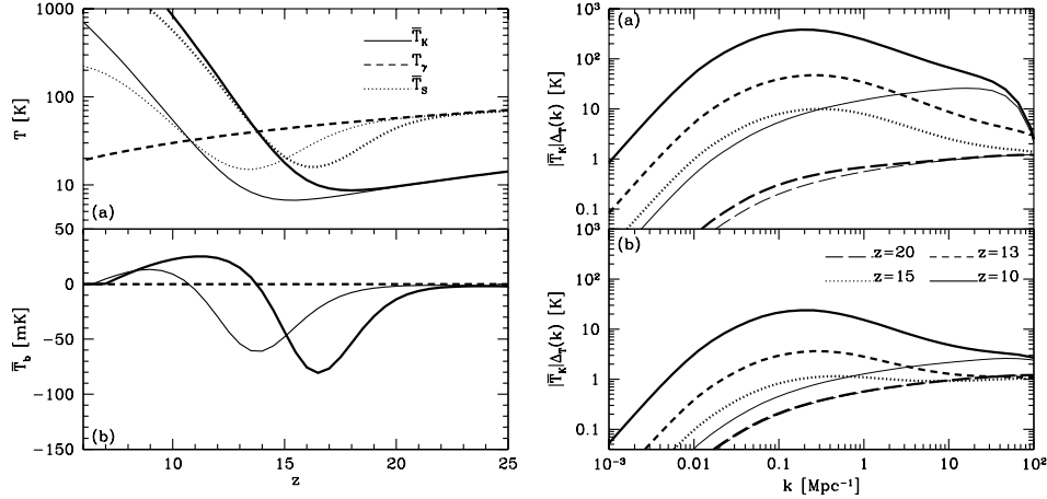
Figure 12.8 Left: Thermal history of two models of X-ray heating, Wouthuysen-Field coupling, and reionization. In the top panel, the solid, dashed, and dotted lines show T_K , T_\gamma , and T_S , respectively. The thick and thin lines take Population II and III star formation properties (see text for details). The bottom panel shows the mean spin-flip brightness temperature T_b in the same two models. Right: Power spectrum of temperature fluctuations in the same models, from z = 20 (where the mean temperature is nearly that of an adiabatically cooling IGM) to z = 10 (where T_K \gg T_\gamma ). The upper and lower panels are for the Population II and Population III models shown at left, respectively. The peak at late times corresponds to the typical mean free path of X-ray photons. The thin curves show the fluctuations for uniform heating (in this case the fluctuations arise from variations in the expansion cooling rate). Figure credit: Pritchard, J. R. & Furlanetto, S. R., Mon. Not. R. Astron. Soc. 376 , 1680 (2007). Copyright 2007 by the Royal Astronomical Society.
