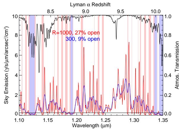
Figure 10.4 “Windows” in the J -band night-sky spectrum. The black line indicates the transmission of the night sky (scale on right). The two lines at the bottom show the night-sky spectrum at two resolutions ( R = 1000 and 300 ; intensity scale on left). The vertical shading shows regions where the emission is less than 1/3 of the mean value. Figure credit: Barton, E. J. et al., Astrophys. J. , 604 , L1 (2004). Reproduced with permission of the American Astronomical Society.
