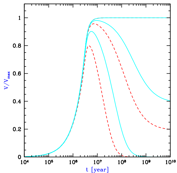
Figure 9.1 Evolution of the effective ionized volume for a stellar ionizing source, scaled to the maximum possible value V_{\text{max}} = 4\pi\bar{n}_H\gamma_{\text{max}}^3/3 (see eq. 9.3). The solid and dashed curves assume that the sources begin shining at z = 10 and 15 , respectively. Within each set, they take C = 0, 1 , and 10 , from top to bottom. The source has \zeta = 40 and is assumed to fade with time like t^{-4.5} after a period t_s = 3 \times 10^6 yr, characteristic of the massive star lifetime. Figure credit: Barkana, R. & Loeb, A., Phys. Rep. , 349 , 125 (2001). Copyright 2001 by Elsevier.
