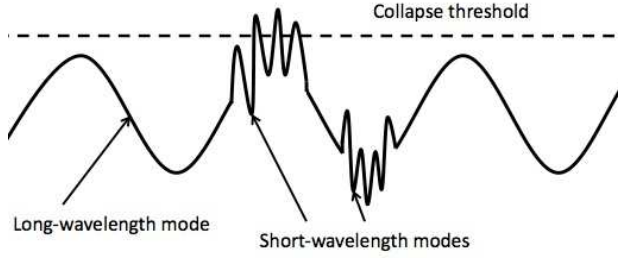
Figure 3.13 Modulation of dark matter halos by the underlying density field. Here, a single long-wavelength mode is shown for simplicity. The dashed horizontal line represents the density threshold for collapse (as in the Press-Schechter model); the large-scale mode does not reach the threshold anywhere. However, (to linear order) the superposed small-scale modes evolve independently of the amplitude of this large-scale field. Where the large-scale field has a high overdensity, it is much easier for the small-scale modes to pass the collapse threshold. We therefore expect dark matter halos to be highly clustered inside large-scale overdense regions.
