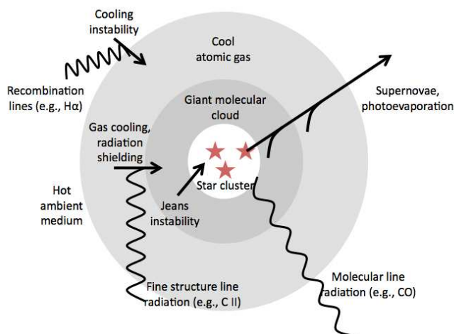
Figure 8.5 Cartoon of baryon flows in the ISM. The multiphase ISM is a hot, ambient medium surrounding cold gas clouds, which form when a thermal instability allows the hot gas to cool locally, producing recombination line radiation (such as H\alpha ). Inside these cool, neutral clouds, radiative cooling continues (largely through fine structure lines such as [C II] ), and the gas column eventually becomes sufficiently thick to shield H_2 from dissociating radiation, allowing a giant molecular cloud to form. Within the cloud, cooling continues via molecular transitions (such as CO ), until regions become gravitationally unstable and form stars. The radiation and eventual explosions of these stars return gas and energy into the hot ISM, so that the process is self-regulating.
