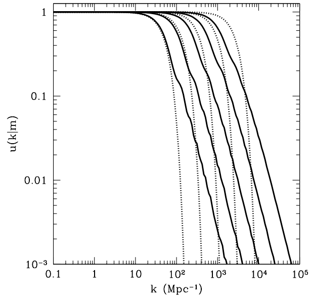
Figure 3.16 Fourier transforms of the normalized halo density profiles for a series of halos at z = 6 . The solid lines show the profiles for halos with NFW profiles and m = 10^6, 10^7, 10^8, 10^9, and 10^{10} M_{\odot} , from right to left (equation 3.56). The dotted lines show the Gaussian profiles of equation (3.59), with the same value of r_s .
