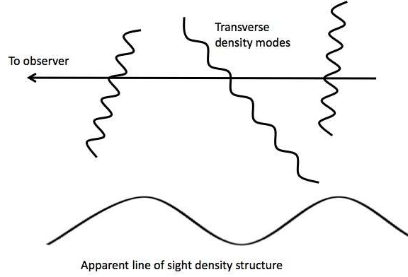
Figure 4.11 Illustration of aliasing in the Lyman- \alpha forest. The observer can only measure structure along the line of sight. However, density modes transverse to that skewer can still leave imprints in the one-dimensional field where they intersect it. The superposition of many such modes can mimic large-scale fluctuations along the line of sight, aliasing power from small to large scales.
