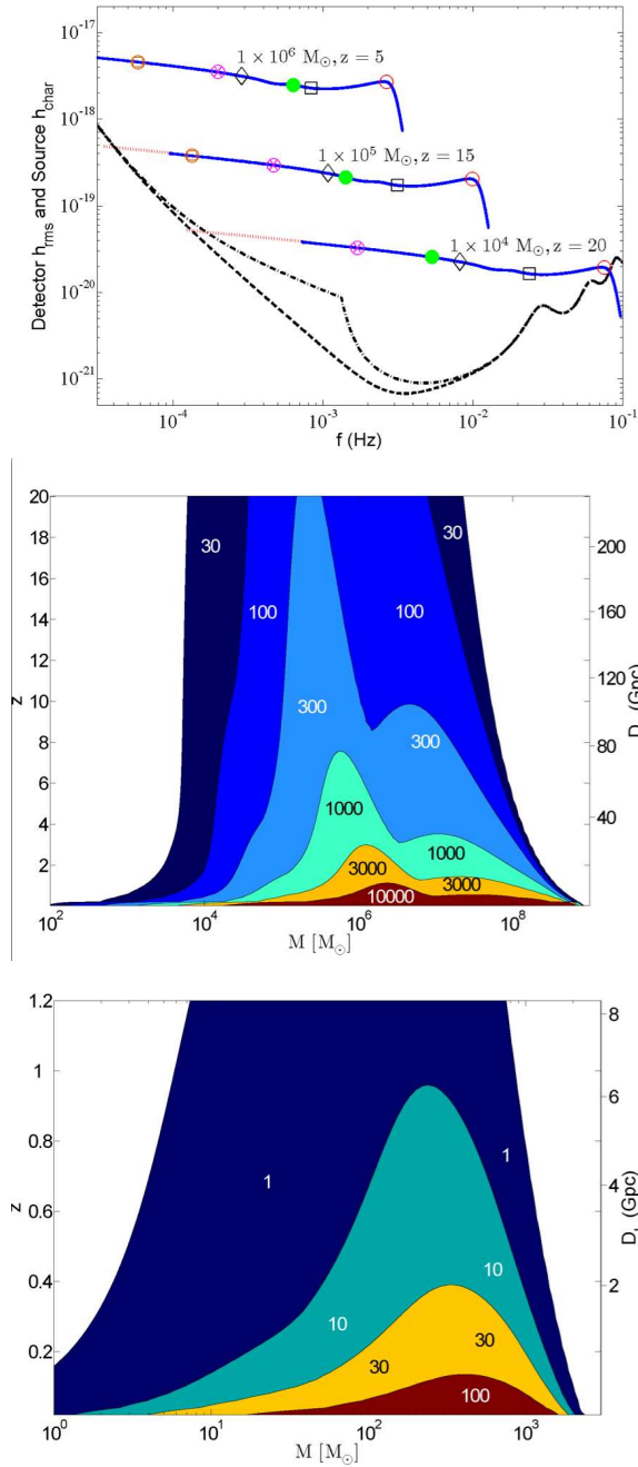
Figure 7.8 Sensitivity of the future gravitational wave observatories, LISA and Advanced-LIGO, to equal-mass ( M_1 = M_2 = M/2 ) binaries (see Color Plate 16 for a color version of this figure). Top panel : Root-mean-square noise amplitude of LISA h_{rms} from the detector only (dashed) and from the detector combined with the anticipated foreground confusion (dash-dotted), along with the characteristic amplitudes h_{char} of three binary masses M (solid). The locations on each h_{char} curve correspond to the peak amplitude (circle), 1 hour before the peak (filled circle), 1 day before the peak (circle with inscribed cross), and 1 month before the peak (circle with inscribed square) in the observer frame, as well as times of 25r_{Sch}/c (square) and 500r_{Sch}/c (diamond) before the peak in the source frame. Middle panel : Contour plot of the signal-to-noise ratio (SNR) with binary mass and redshift dependence for LISA. Bottom panel : SNR contour plot with mass and redshift dependence for Advanced-LIGO. Figure credit: Baker, J., et al. Phys. Rev. D75 , 4024 (2007). Copyright 2007 by the American Physical Society.
