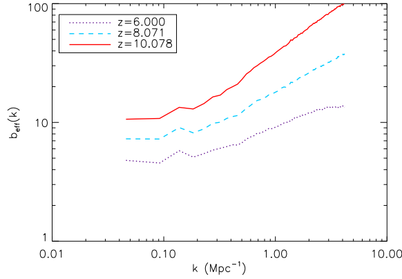
Figure 3.18 Average effective bias for halos with M > 2 \times 10^9 M_\odot as a function of spatial scale, estimated by comparing the nonlinear and linear power spectra via b_{\text{eff}}^2(k) = P(k)/P_{\text{lin}}(k) , where the “shot noise” term is already subtracted to obtain the clustering-driven component of the power spectrum P(k) . The three different curves vary the redshift of the bias measurement. Figure credit: Fernandez, E. et al., Astrophys. J. , 710 , 1089 (2010). Reproduced with permission of the American Astronomical Society.
