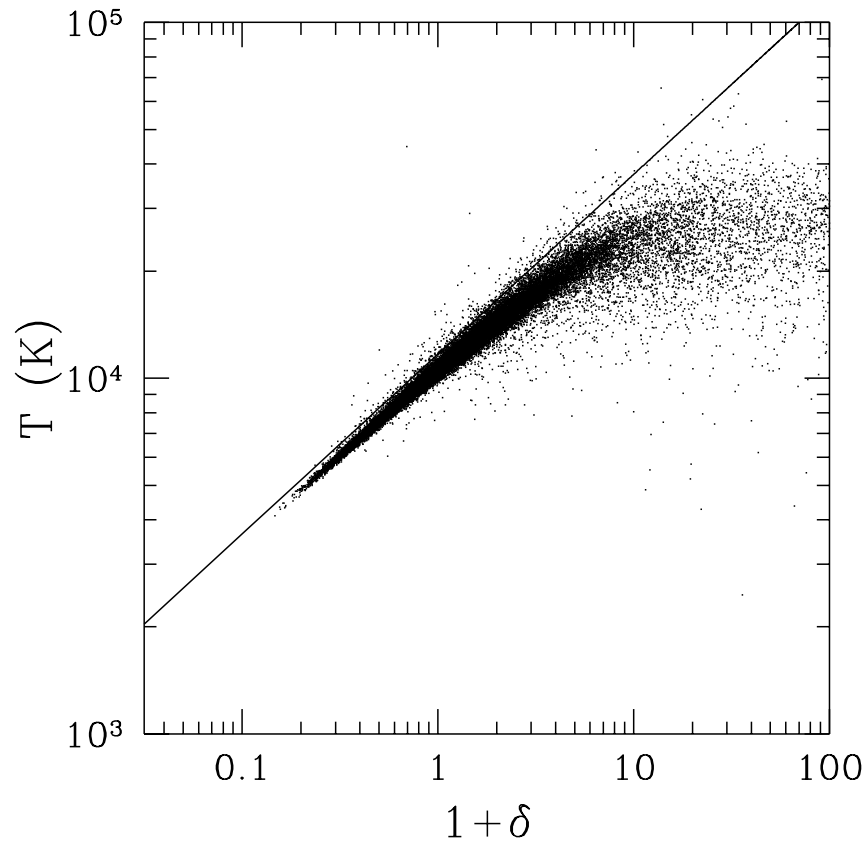
Figure 4.7 Temperature-density relation at z = 4 in a cosmological simulation (points), together with analytic prediction based on linear perturbation theory and equation (4.22). Note the near power-law relation, except at very high densities where the complex physics of nonlinear structure formation begin to matter. Figure credit: Hui, L. & Gnedin, N. Y. Mon. Not. R. Astron. Soc. 292 , 27 (1997). Copyright 1997 by the Royal Astronomical Society.
