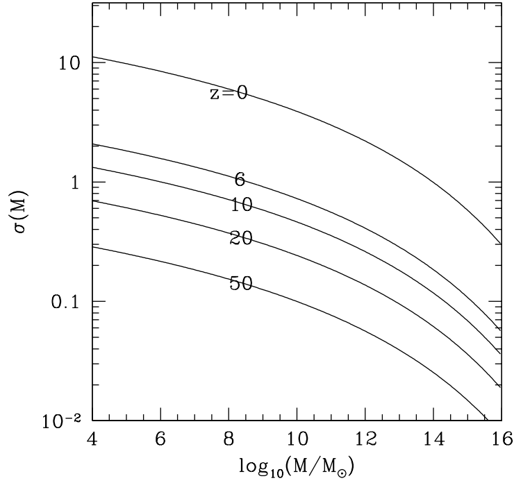
Figure 2.4 The root-mean-square amplitude of linearly-extrapolated density fluctuations \sigma as a function of mass M (in solar masses M_{\odot} , within a spherical top-hat filter) at different redshifts z . Halos form in regions that exceed the background density by a factor of order unity. This threshold is only surpassed by rare (many- \sigma ) peaks for high masses at high redshifts. When discussing the abundance of halos, we will factor out the linear growth of perturbations and use the function \sigma(M) at z = 0 . The comoving radius of an unperturbed sphere containing a mass M is R = 1.85(M/10^{12} M_{\odot})^{1/3} Mpc.
