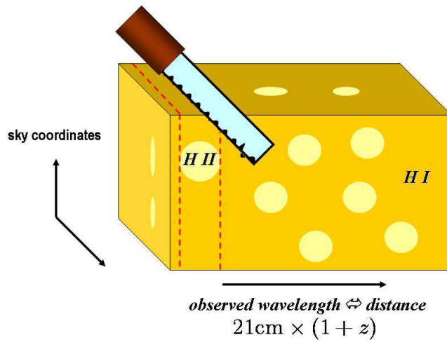
Figure 12.1 21-cm imaging of ionized bubbles during the epoch of reionization is analogous to slicing Swiss cheese (for a color version of this figure). The technique of slicing at intervals separated by the typical dimension of a bubble is optimal for revealing different patterns in each slice.
