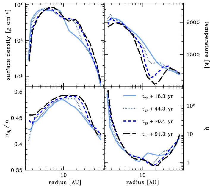
Figure 5.8 Radial profile of disk physical properties from the same simulation shown in Fig. 5.7, centered on the first protostellar core to form. Clockwise from upper left, the panels show the surface density, temperature, Toomre- Q parameter, and molecular fraction. Note how the disk parameters do not evolve strongly with time (shown with the different curves in each panel). The second core to form in the simulation forms within the region near r \sim 20 AU where Q < 1 . Figure credit: Clark, P. C. et al., Science 331 , 1040 (2011). Copyright 2008 by the American Association for the Advancement of Science.
