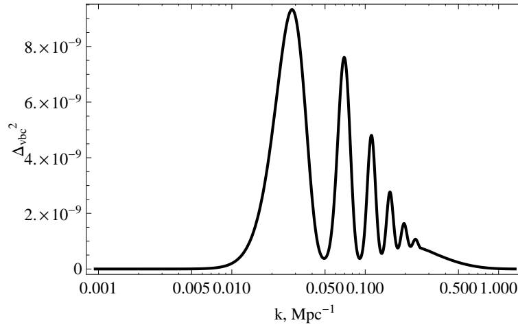
Figure 2.2 The variance of the velocity difference perturbations (in units of c ) between baryons and dark matter per \ln k as a function of comoving wavenumber k at z = 10^3 . Figure credit: Tseliakhovich, D. & Hirata, C., Phys. Rev. D82 , 3520 (2010). Copyright 2010 by the American Physical Society.
