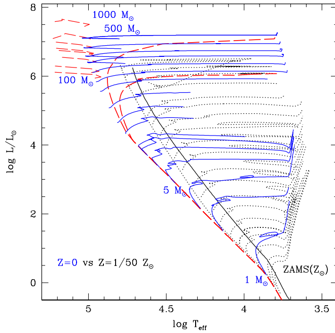
Figure 5.13 Main sequence evolutionary tracks for Population III stars (solid lines: without mass loss; short-dashed lines: with strong mass loss) and Z = 0.02 Z_\odot stars (dotted lines). Isochrones at 2 and 4 Myr for the Z = 0 stars are also shown with the long-dashed lines. The zero-age main sequence for solar-metallicity stars is shown by the vertical solid line; note that Population III stars are significantly hotter (bluer) than their higher-metallicity counterparts. Figure credit: Schaerer, D., Astron. & Astrophys. , 382 , 28 (2002).
