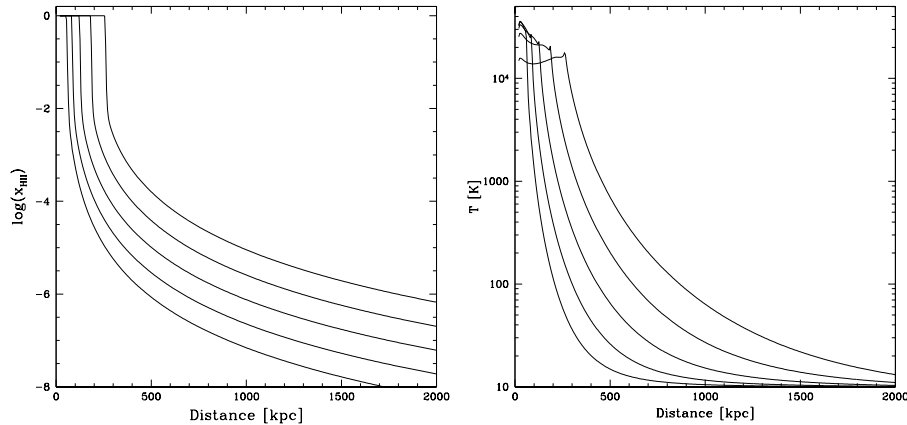
Figure 9.12 Example ionization and temperature profiles around a relatively bright quasar at z = 10 , with L_B = 10^9 L_\odot . The source is assumed to emit steadily after it turns on, and the different curves take t = 10^6, 10^{6.5}, 10^7, 10^{7.5}, and 10^8 yr after ignition. The calculation assumes an initial IGM temperature of T = 10 K and a uniform IGM at the mean density (including helium); note that distances are measured in proper (not comoving) units.
