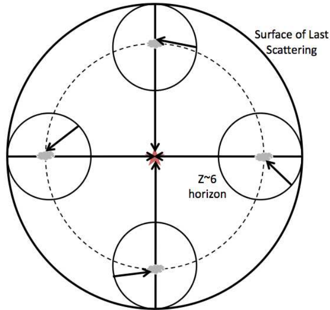
Figure 13.1 Cartoon of the damping of primordial CMB anisotropies after reionization (in comoving coordinates). The observer is represented by the star at the center; the thick outer circle represents the surface of last scattering of the observer. CMB photons (arrows) propagate through a screen of parcels of free electrons at z \sim 6 (located at the dashed circle for the observer). Each parcel sees the CMB out to its causal horizon, represented by the smaller circle surrounding it. The low optical depth of free electrons implies that most CMB photons propagate through without interaction (long arrows), but some photons are scattered into the line of sight from other directions. This partially washes out the primordial anisotropies on scales smaller than the horizon at the time of scattering.
