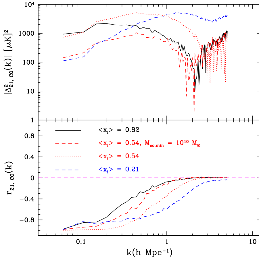
Figure 13.10 Cross-correlation between CO(2-1) emission and the spin-flip background in a numerical simulation of reionization (as in Figure 13.9). The dot-dashed, dotted, and solid curves take z = 9.8 , 7.3 , and 6.8 (or Q_{\text{HII}} = 0.21 , 0.54 , and 0.82 in this model), assuming that all galaxies emit CO(2-1). The long-dashed curve takes z = 7.3 but assumes that only massive galaxies emit CO. The top and bottom panels show the absolute value of the cross-power spectrum and the cross-correlation coefficient, respectively. Figure credit: Lidz, A. et al., Astrophys. J. 741 , 70 (2011). Reproduced with permission of the American Astronomical Society.
