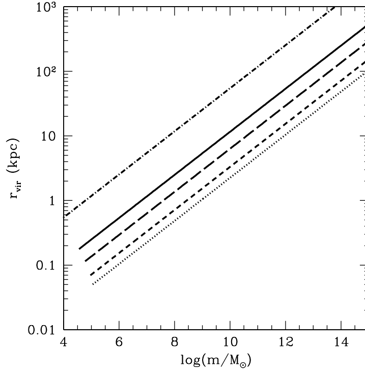
Figure 3.5 Virial radius over a wide range of halo masses and redshifts (equation 3.30). The dotted, short-dashed, long-dashed, solid, and dot-dashed curves take z = 30, 20, 10, 5, and 0 , respectively.
