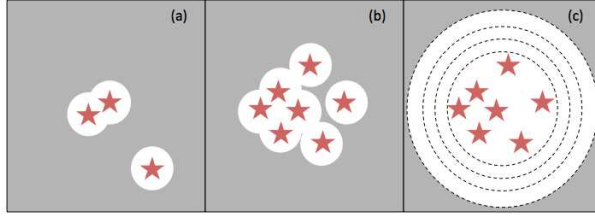
Figure 9.4 Cartoon of the excursion set model for generating the ionization morphology. (a) In the initial stages, where galaxies are nearly isolated, it is straightforward to compute the ionized volume (white circles) around each source (stars), given only its ionizing efficiency. However, if two such volumes overlap, the overlap region must be distributed over the remaining volume so that ionizing photons are conserved. (b) This problem becomes especially acute once a substantial fraction of the IGM is ionized: in that case, redistributing the overlap volume can link up previously separate ionizing bubbles, causing a cascading effect. (c) The solution is to work from the outside in, rather than trying to begin with each individual galaxy. Here, we compare the number of atoms contained inside the large circle with the number of ionizing photons generated by all the galaxies inside that region. If the latter is larger, the region is ionized; if not, we ask the same question for smaller regions (shown by the dashed circles), until the two quantities balance.
