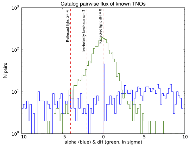
Figure 3: Example of pairwise measurements of H -magnitude for a sample of literature TNOs with d > 25 AU taken at different times, the broad distribution in standard deviations illustrating that there exist significant errors in the photometry presented in existing catalogs. The luminosity variation slope \alpha is also illustrated for the same pairwise observations, where 0 indicates no variation in distance between the observations.
