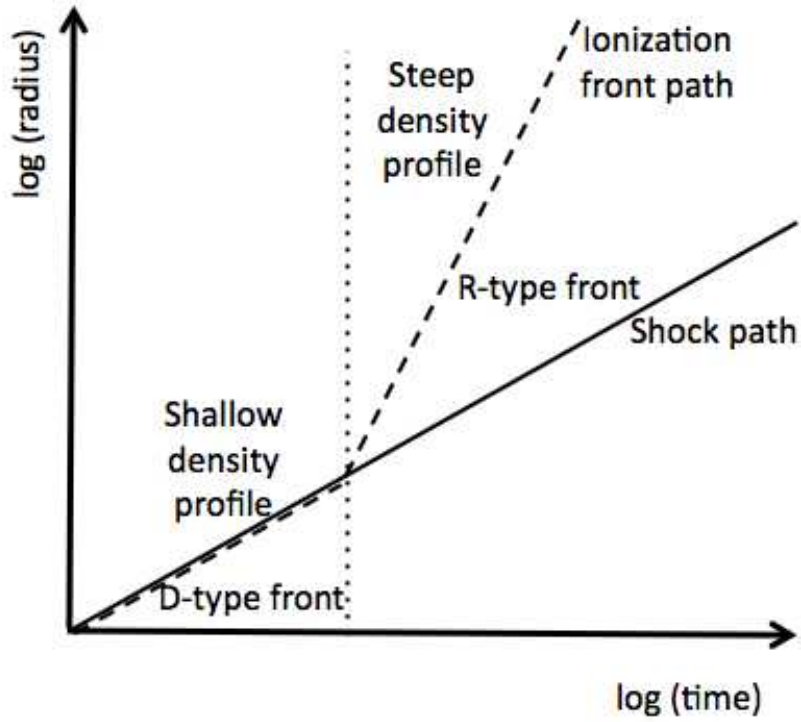
Figure 6.5 Cartoon of an ionization front propagating through a cosmological halo. The dashed and solid lines show the locations of the ionization front and shock, respectively. After an initial R-type phase (not shown), recombinations in the high-density core trap the front, making it D-type, in which a shock slightly leads the ionization front. As the density falls through the halo, the recombination rate also falls, eventually freeing the front to expand much faster than the sound speed. The shock is left behind and lags the front, often eventually transforming into a simple pressure wave.
