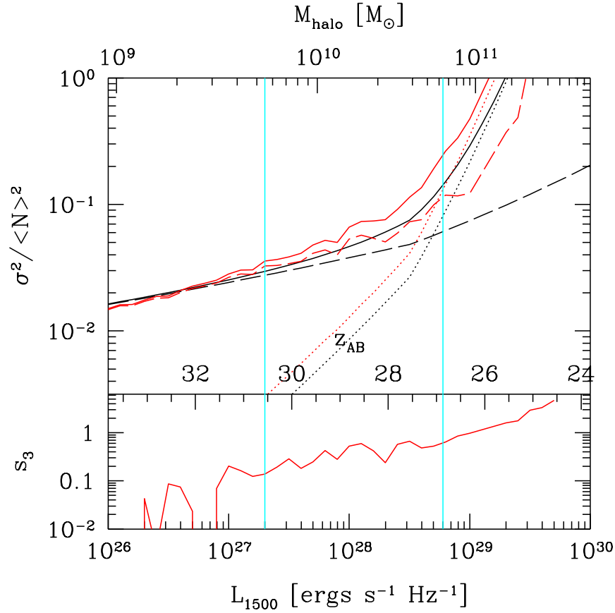
Figure 10.15 Upper panel: Predicted relative contributions to the fractional variance in the number counts of galaxies as a function of UV luminosity at an emission wavelength of 1500 \text{ \AA} within a Lyman-break dropout survey spanning the redshift interval z = 6\text{--}8 with a 3.4' \times 3.4' field-of-view (matching HUDF and approximately that of JWST). Solid lines show the total variance, while long-dashed and dotted lines show the contributions from cosmic variance and Poisson noise, respectively. The upper curves show the results from numerical simulations, while the lower curves were calculated analytically based on linear perturbation theory. Vertical lines bracket the region where the variance is higher than expected due to the skewness of the full count probability distribution but is not Poisson-dominated. The middle and top horizontal axes translate the monochromatic luminosity to z -band AB magnitude and host halo mass, respectively. Lower panel: Skewness of the full galaxy count probability distribution calculated from a numerical simulation based on equation (10.24). Figure credit: Munoz, J., Trac, H., & Loeb, A. Mon. Not. R. Astron. Soc. , 405 , 2001 (2010). Copyright 2010 by the Royal Astronomical Society.
