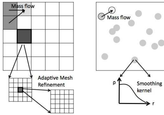
Figure 3.19 Numerical methods for solving hydrodynamics. At left, we show a grid-based algorithm, where the continuous fluid quantities are discretized on a grid, with the equations solved along the grid faces. Mass flows are described by exchanging material between the cells. Resolution is often increased through adaptive mesh refinement , where a new grid is spawned once certain criteria are reached (most commonly, a density or timestep criterion). At right, we illustrate smoothed-particle hydrodynamics, in which the matter field is discretized into a set of particles that can flow freely through the simulation volume. Each particle describes a fixed mass, distributed according to a smoothing kernel illustrated at bottom. Mass flows by moving the particles around.
