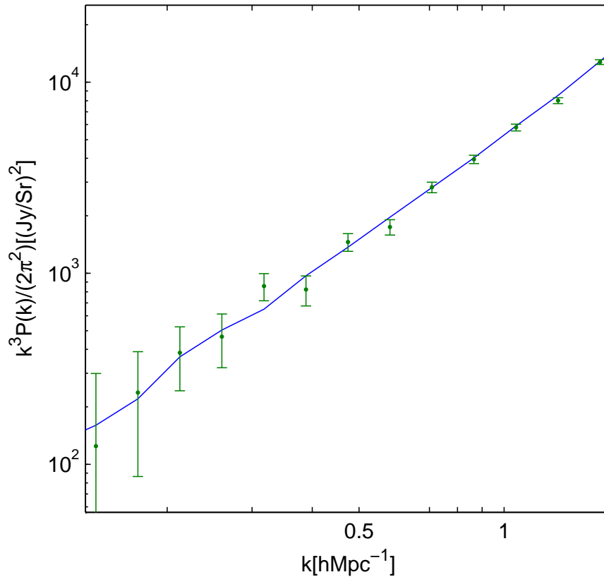
Figure 13.8 The cross power spectrum of O I( 63 \mu\text{m} ) and O III( 52 \mu\text{m} ) at z = 6 measured from mock simulation data for a hypothetical infrared space telescope (see text). The solid line is the cross power spectrum measured when only line emission from galaxies in the target lines is included. The points with error bars are the recovered power spectrum when detector noise, contaminating line emission, galaxy continuum emission, dust in our galaxy and the CMB are included (see equation 13.29). Figure credit: Visbal, E., Trac, H., & Loeb, A., J. Cosm. Astropart. Phys. 11 , 16 (2011). Copyright 2011 by the Institute of Physics.
