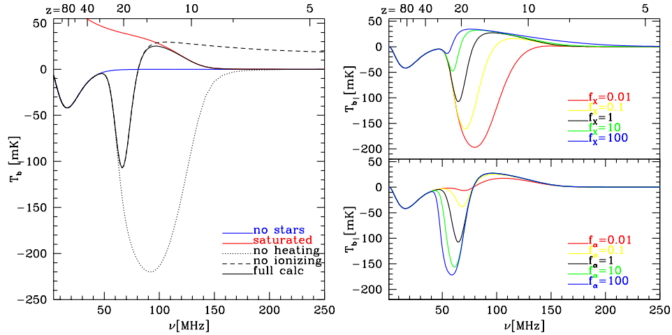
Figure 12.9 Monopole of the spin-flip brightness temperature (so-called the “global 21-cm signal”) in several models of early structure formation (see Color Plate 27 for a color version of this figure). Left : Major variations around our fiducial model (solid curve with several turning points), as indicated. Each curve either eliminates a physical process (like heating or ionization) or maximizes it. Right : Suites of models in which we vary the Lyman- \alpha (lower panel) and X-ray heating (upper panel) efficiencies by a factor of 10^4 . Figure credit: Pritchard, J. R. & Loeb, A., Phys. Rev. D 82 , 023006 (2010). Copyright 2010 by the American Physical Society.
