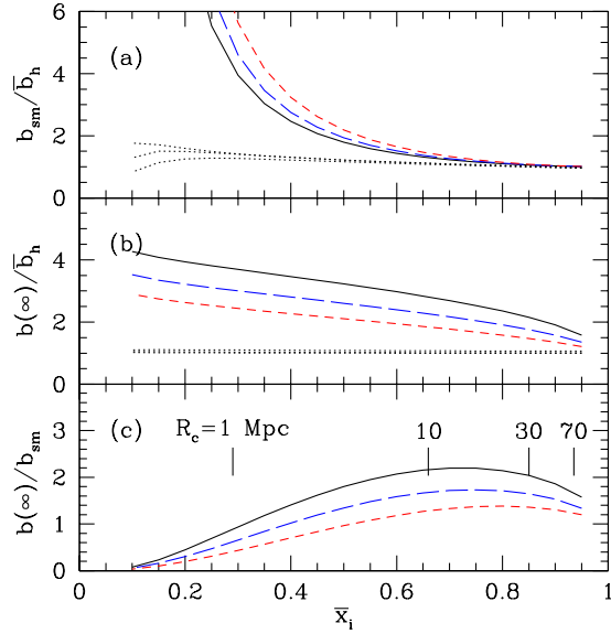
Figure 11.18 (a): Predicted small-scale bias of LAEs at z = 10 , relative to the bias expected if all galaxies above the mass threshold were visible. This applies to separations larger than the nonlinear scale but smaller than the characteristic bubble size R_c . The solid, long-dashed, and short-dashed curves take m_{\text{obs,min}} = 10^8 , 10^9 , and 10^{10} M_\odot , respectively. The dotted curves show the predicted galaxy bias, neglecting absorption, relative to its true value (the small errors at early times result from the approximations described in the text). (b): Predicted large-scale bias at z = 10 , relative to the bias expected if all galaxies above the mass threshold were visible. (c): Ratio of large to small scale bias; the transition between the two regimes will occur roughly at R_c , which is marked for a few different values of the bubble filling factor Q_{\text{H II}} = \bar{x}_i . Figure credit: Furlanetto, S.R. et al., Mon. Not. R. Astron. Soc. , 365 , 1012 (2006). Copyright 2006 by the Royal Astronomical Society.
