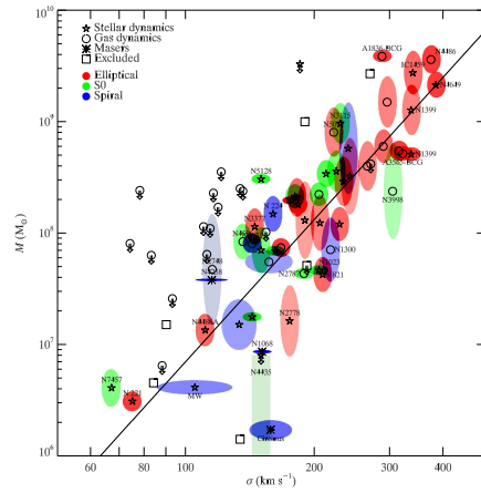
Figure 7.7 Dynamical measurements of the correlation between supermassive black hole mass, M_{\text{BH}} , and velocity dispersion of stars in the spheroid of its host galaxy, \sigma_* (see Color Plate 15 for a color version of this figure). The symbol indicates the method of black hole mass measurement: dynamics of stars ( pentagrams ), dynamics of gas ( circles ), dynamics of maser sites ( asterisks ). Arrows indicate 3\sigma upper limits to black hole mass. The shade of the error ellipse indicates the Hubble type of the host galaxy: elliptical, S0, or spiral. The line is the best fit relation to the full sample: M_{\text{BH}} = 10^{8.12} M_{\odot} (\sigma_*/200 \text{ km s}^{-1})^{4.24} . The mass uncertainty for NGC 4258 has been plotted much larger than its actual value so that it will show on this plot. Figure credit: Gültekin, K., et al. Astrophys. J. 698 , 198 (2009). Reproduced with permission of the American Astronomical Society.
