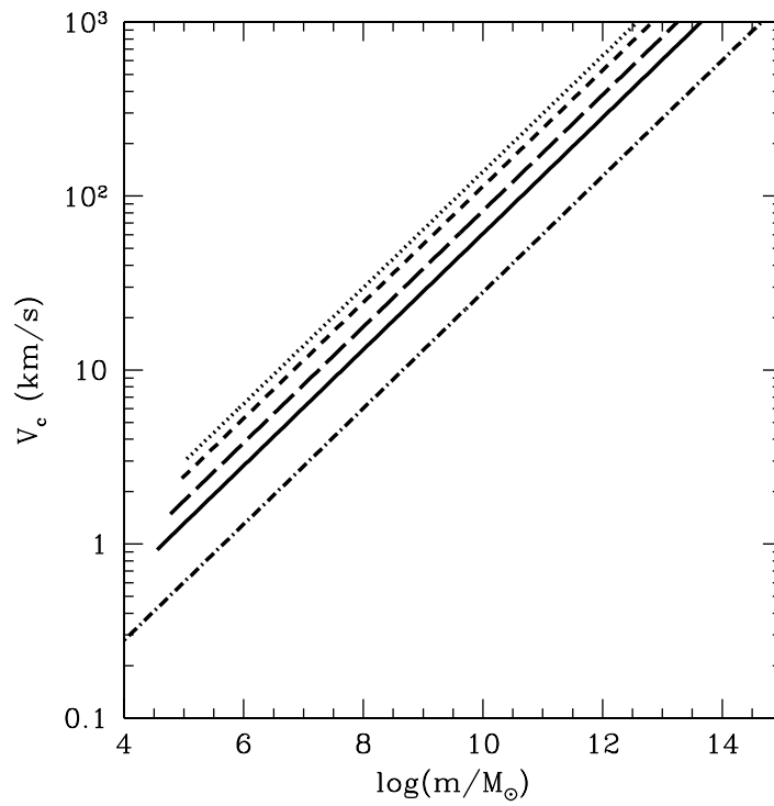
Figure 3.6 Circular velocity over a wide range of halo masses and redshifts (equation 3.31). The dotted, short-dashed, long-dashed, solid, and dot-dashed curves take z = 30, 20, 10, 5, and 0, respectively.
