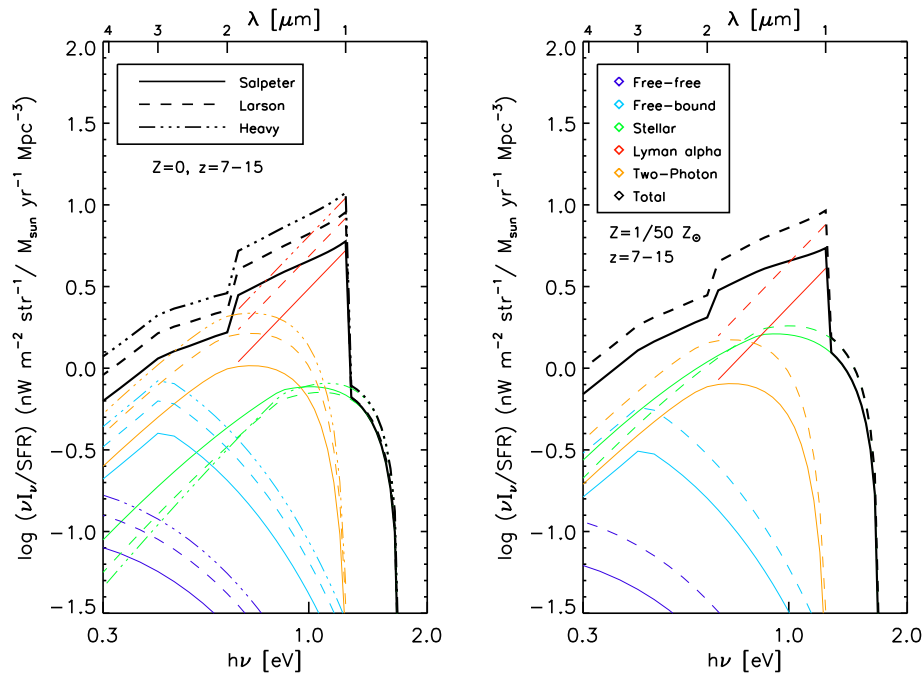
Figure 13.6 Near-infrared background spectrum (see Color Plate 31 for a color version of this figure). This example includes star formation from z = 7-15 (with constant comoving star formation rate), which dominates the background between 1-2 \mu\text{m} . The left panel assumes metal-free stars, while the right panel takes a metallicity Z = 0.02 Z_\odot . The different line styles show different IMFs (see text). The different curves show the total emission, the Lyman- \alpha contribution, the stellar continua, the two-photon continua, the free-bound emission, and finally the free-free emission (from top to bottom at 1 \mu\text{m} ). Figure credit: Fernandez, E. R. & Komatsu, E., Astrophys. J. 646 , 703 (2006). Reproduced with permission of the American Astronomical Society.
