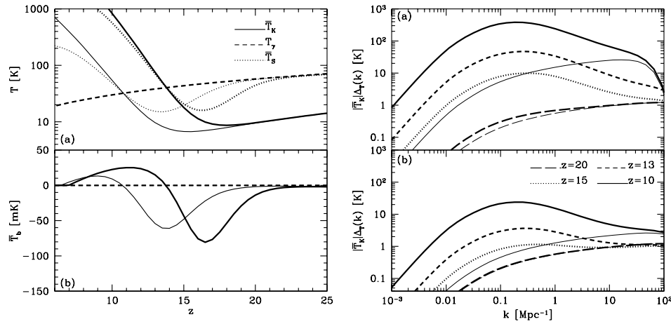
Figure 12.8 Left : Thermal history of two models of X-ray heating, Wouthuysen-Field coupling, and reionization. In the top panel, the solid, dashed, and dotted lines show T_K , T_\gamma , and T_S , respectively. The thick and thin lines take Population II and III star formation properties (see text for details). The bottom panel shows the mean spin-flip brightness temperature T_b in the same two models. Right : Power spectrum of temperature fluctuations in the same models, from z = 20 (where the mean temperature is nearly that of an adiabatically cooling IGM) to z = 10 (where T_K \gg T_\gamma ). The upper and lower panels are for the Population II and Population III models shown at left, respectively. The peak at late times corresponds to the typical mean free path of X-ray photons. The thin curves show the fluctuations for uniform heating for comparison (in this case the fluctuations arise from variations in the expansion cooling rate). Figure credit: Pritchard, J. R. & Furlanetto, S. R., Mon. Not. R. Astron. Soc. 376 , 1680 (2007). Copyright 2007 by the Royal Astronomical Society.
