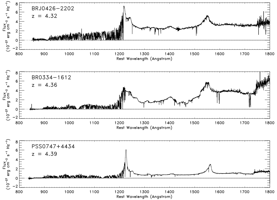
Figure 4.5 Example Lyman- \alpha forest spectra taken with the ESI spectrograph on the Keck Telescope. The highly variable absorption blueward of the Lyman- \alpha rest wavelength (at 1216 Å) is the Lyman- \alpha forest, not noise. Redward of this transition, the quasar continuum is visible, with only a few absorption features due to metal line absorbers in the IGM. Figure credit: Songaila, A. & Cowie, L., Astrophys. J. , 721 , 1448 (2011). Reproduced with permission of the American Astronomical Society.
