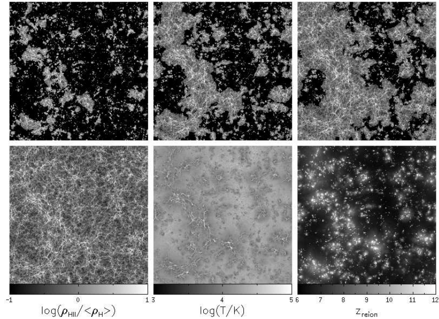
Figure 9.3 Snapshots from a numerical simulation illustrating the spatial structure of cosmic reionization in a slice of 140 comoving Mpc on a side. The simulation describes the dynamics of the dark matter and gas as well as the radiative transfer of ionizing radiation from galaxies. The first four panels (reading across from top left to bottom left) show the evolution of the ionized hydrogen density \rho_{\text{HII}} normalized by the mean proton density in the IGM \langle\rho_{\text{H}}\rangle = 0.76\Omega_b\bar{\rho} when the simulation volume is 25%, 50%, 75%, and 100% ionized, respectively. Large-scale overdense regions form large concentrations of galaxies whose ionizing photons produce joint ionized bubbles. At the same time, galaxies are rare within large-scale voids in which the IGM is mostly neutral at early times. The bottom middle panel shows the temperature at the end of reionization while the bottom right panel shows the redshift at which different gas elements are reionized. Higher-density regions tracing the large-scale structure are generally reionized earlier than lower density regions far from sources. At the end of reionization, regions that were last to get ionized and heated are still typically hotter because they have not yet had time to cool through the cosmic expansion. Figure credit: Trac, H. & Loeb, A. (2010).
