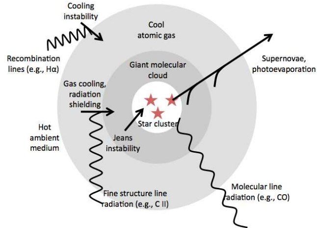
Figure 8.5 Cartoon of baryon flows in the ISM. The multiphase ISM is a hot, ambient medium surrounding cold gas clouds, which form when a thermal instability allows the hot gas to cool locally, producing recombination line radiation (such as \text{H}\alpha ). Inside these cool, neutral clouds, radiative cooling continues (largely through fine structure lines such as [\text{C II}] ), and the gas column eventually becomes sufficiently thick to shield \text{H}_2 from dissociating radiation, allowing a giant molecular cloud to form. Within the cloud, cooling continues via molecular transitions (such as \text{CO} ), until regions become gravitationally unstable and form stars. The radiation and eventual explosions of these stars return gas and energy into the hot ISM, so that the process is self-regulating.
