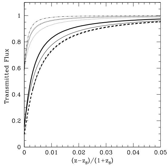
Figure 11.6 Damping wing absorption profiles, as a function of fractional wavelength offset from the source (at redshift z_s ). The thick curves show the absorption profiles for \bar{x}_D = 0.9, 0.5, and 0.1 assuming the “picket fence” model of absorption (with the dashed, solid, and dotted curves, respectively). Note that the two dashed curves overlap and are practically indistinguishable. The corresponding thin curves show the absorption profiles for uniformly ionized IGM normalized to the same transmission at z_s . The dot-dashed curve shows the profile of a DLA, normalized to the same transmission as the \bar{x}_D = 0.1 curves at z_s . Figure credit: Mesinger, A. & Furlanetto, S.R., Mon. Not. R. Astron. Soc. , 385 , 1348 (2008). Copyright 2008 by the Royal Astronomical Society.
