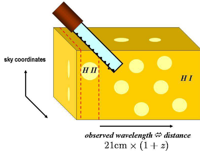
Figure 12.1 21-cm imaging of ionized bubbles during the epoch of reionization is analogous to slicing Swiss cheese for a color version of this figure). The technique of slicing at intervals separated by the typical dimension of a bubble is optimal for revealing different patterns in each slice.
