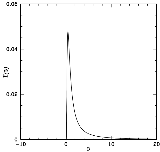
Figure 11.11 Monochromatic photon luminosity of a Lyman- \alpha halo as a function of normalized frequency shift from the Lyman- \alpha resonance, \tilde{\nu} \equiv (\nu_\alpha - \nu)/\nu_* . Note that only the photons inside the red damping wing scatter in this compact halo; those on the blue side of Lyman- \alpha scatter at much larger distances. The observed spectral flux of photons F(\nu) (in photons \text{cm}^{-2} \text{s}^{-1} \text{Hz}^{-1} ) from the entire Lyman- \alpha halo is F(\nu) = (\tilde{L}(\tilde{\nu})/4\pi d_L^2)(\dot{N}_\alpha/\nu_*)(1+z_s)^2 where \dot{N}_\alpha is the production rate of Lyman- \alpha photons by the source (in photons \text{s}^{-1} ), \nu = \tilde{\nu}\nu_*/(1+z_s) , and d_L is the luminosity distance to the source. Figure credit: Loeb, A. & Rybicki, G. B. Astrophys. J. 524 , 527 (1999). Reproduced with permission of the American Astronomical Society.
