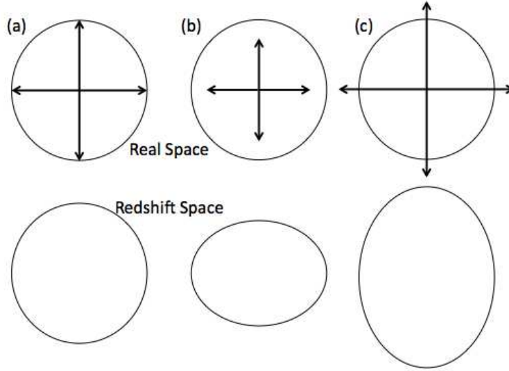
Figure 12.13 Cartoon of redshift space distortions in the linear regime. If an observation uses redshift as a proxy for distance, it is subject to confusion if velocities do not precisely follow the mean Hubble expansion. In (a), we imagine observing a region at the mean density, so that the Hubble flow is correct (top row). In that case, the inferred radial width of the region will be precisely correct (bottom row). However, if the region is overdense, so that the local expansion rate is smaller than the Hubble flow, the inferred radial width will be smaller than its true width, so the observed density will be even larger (column b). Finally, if the region is underdense (and so expanding faster than average, it will appear even more underdense in redshift-space (column c).
