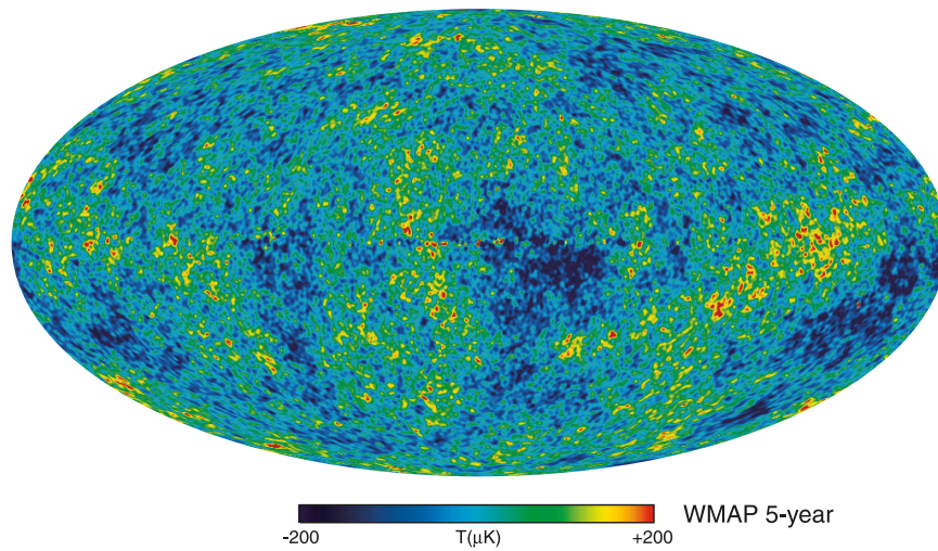
Figure 1.1 Image of the Universe when it first became transparent, 400,000 years after the Big Bang, taken over five years by the Wilkinson Microwave Anisotropy Probe (WMAP) satellite (see Color Plate 1 for a color version of this figure). Slight density inhomogeneities at the level of one part in \sim 10^5 in the otherwise uniform early Universe imprinted hot and cold spots in the temperature map of the cosmic microwave background on the sky. The fluctuations are shown in units of \mu\text{K} , with the unperturbed temperature being 2.73 K. The same primordial inhomogeneities seeded the large-scale structure in the present-day Universe. The existence of background anisotropies was predicted in a number of theoretical papers three decades before the technology for taking this image became available. Figure credit: WMAP/NASA, http://map.gsfc.nasa.gov/
