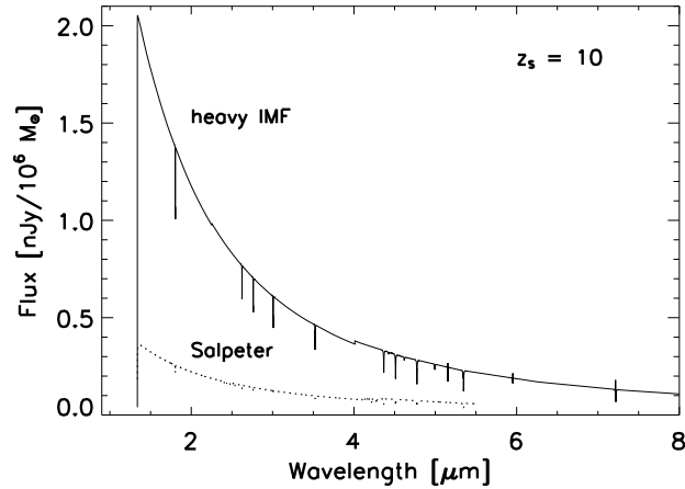
Figure 5.14 Comparison of the observed flux per unit frequency from a cluster of Population III stars at a redshift z_s = 10 for a Salpeter IMF ( dotted line ) and an IMF composed purely of very massive stars ( solid line ). The flux in units of nJy per 10^6 M_\odot of stars is plotted as a function of observed wavelength in \mu\text{m} . The cutoff below an observed wavelength of 1216 \text{ \AA} (1 + z_s) = 1.34 \mu\text{m} is due to hydrogen Lyman- \alpha absorption in the IGM (the so-called Gunn-Peterson effect; see §4.3). Figure credit: Bromm, V. Kudritzki, R. P. & Loeb, A. Astrophys. J. 552 , 464 (2001); Salpeter curve from Tumlinson, J., & Shull, M. J. Astrophys. J. 528 , L65 (2000). Reproduced with permission of the American Astronomical Society.
