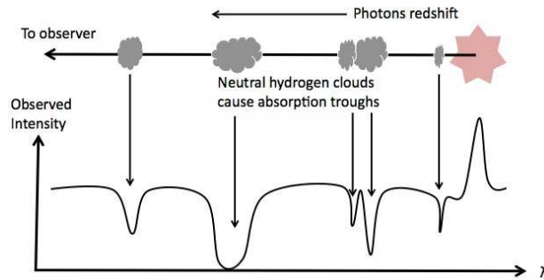
Figure 4.4 The Lyman- \alpha forest. In the top panel, light from a distant quasar passes through several clouds of neutral hydrogen along the line of sight. As these photons travel, they redshift. Photons beginning blueward of the Lyman- \alpha transition at the quasar will eventually redshift through that resonance. If they do so inside an H I cloud, they may be absorbed by those atoms, creating an absorption feature in the quasar's spectrum. The spectra of distant quasars therefore allow us to map the IGM's density and ionization structure.
