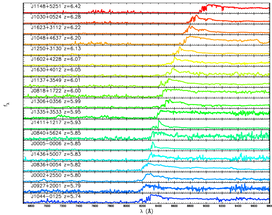
Figure 4.6 Observed spectra of 19 quasars with redshifts 5.74 < z < 6.42 from the Sloan Digital Sky Survey (see Color Plate 3 for a color version of this figure). For some of the highest-redshift quasars, the spectra show no transmitted flux shortward of the Lyman- \alpha wavelength at the quasar redshift, providing a possible hint of the so-called “Gunn-Peterson trough” and indicating a slightly increased neutral fraction of the IGM. It is evident from these spectra that broad-band photometry is adequate for inferring the redshift of sources during the epoch of reionization. Figure credit: Fan, X., et al. Astron. J. 128 , 515 (2004). Reproduced with permission of the American Astronomical Society.
