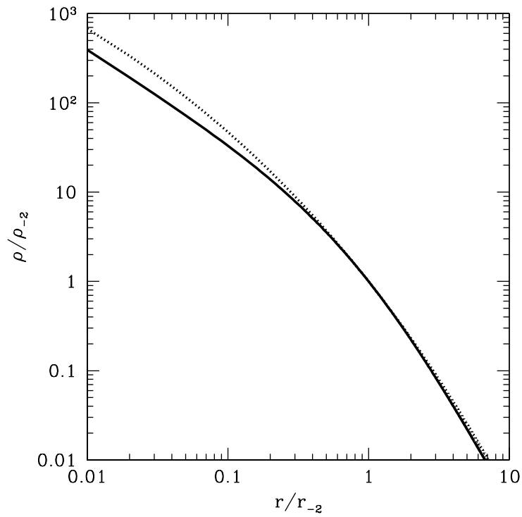
Figure 3.8 Parameterizations for the “universal” dark matter halo profile. The NFW prescription (eq. 3.34) is shown with the solid line, while the Einasto profile (eq. 3.36) is shown with the dotted line. We scale both to the point at which the logarithmic slope equals -2 . For the NFW profile, this is at r = r_{\text{vir}}/c_N , where c_N is the concentration.
