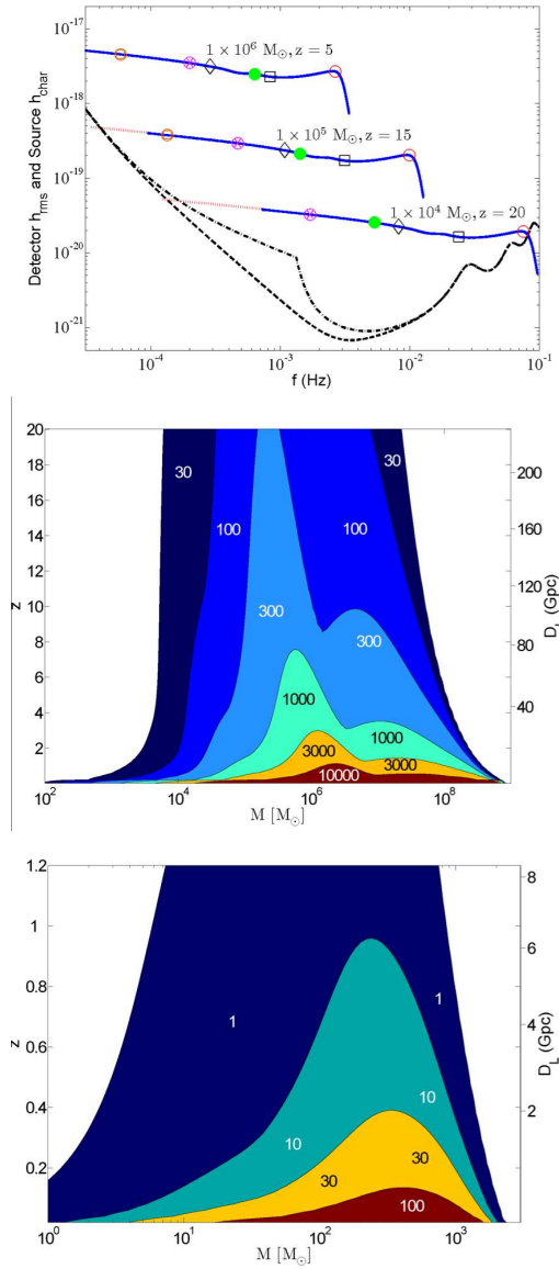
Figure 7.8 Sensitivity of the future gravitational wave observatories, LISA and Advanced-LIGO, to equal-mass ( M_1 = M_2 = M/2 ) binaries (see Color Plate 16 for a color version of this figure). Top panel: Root-mean-square noise amplitude of LISA h_{rms} from the detector only (dashed) and from the detector combined with the anticipated foreground confusion (dash-dotted), along with the characteristic amplitudes h_{char} of three binary masses M (solid). The locations on each h_{char} curve correspond to the peak amplitude (circle), 1 hour before the peak (filled circle), 1 day before the peak (circle with inscribed cross), and 1 month before the peak (circle with inscribed square) in the observer frame, as well as times of 25r_{Sch}/c (square) and 500r_{Sch}/c (diamond) before the peak in the source frame. Middle panel: Contour plot of the signal-to-noise ratio (SNR) with binary mass and redshift dependence for LISA. Bottom panel: SNR contour plot with mass and redshift dependence for Advanced-LIGO. Figure credit: Baker, J., et al. Phys. Rev. D 75 , 4024 (2007). Copyright 2007 by the American Physical Society.
