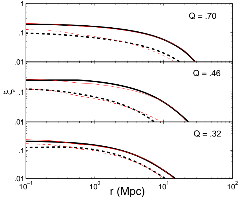
Figure 9.11 Comparison of the autocorrelation function of the ionized fraction (solid curves) and the cross-correlation function of the ionized fraction and density (dashed lines). In each case, the thick lines show our analytic approximations of equations (9.49) and (9.52), while the thin curves show results for a semi-numerical simulation in a 100h^{-1} Mpc box. The two methods are in quite good agreement at a wide range of ionized fractions. Figure credit: McQuinn, M. et al., Astrophys. J. , 630 , 643 (2005). Reproduced with permission of the American Astronomical Society.
