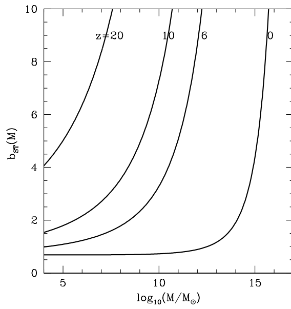
Figure 3.14 The linear bias of halos as a function of M at different redshifts z according to the Sheth-Tormen model (equations 3.46 and 3.54).
