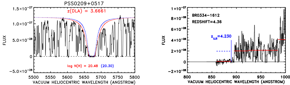
Figure 4.10 Example IGM Lyman- \alpha absorbers measured by the ESI spectrograph on the Keck Telescope. Left: A damped Lyman- \alpha absorber (DLA). The two curves show fits to the absorber; note the long damping wings. Right: A Lyman-limit system (LLS) that is opaque to ionizing radiation (with \lambda < 912 \text{ \AA} ). The horizontal bars redward of 912 \text{ \AA} show fits to the quasar continuum; the dashed line blueward of this wavelength shows the expected flux. The observed flux is much smaller because of the LLS, whose location is marked with the vertical line. Figure credit: Songaila, A. & Cowie, L., Astrophys. J. , 721 , 1448 (2011). Reproduced with permission of the American Astronomical Society.
