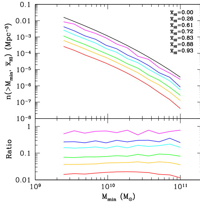
Figure 11.15 Luminosity function of LAEs at z = 9 in a semi-numeric simulation of reionization, as a function of the mean neutral fraction \bar{x}_{\text{HI}} = 1 - Q_{\text{H II}} . The sequence of curves from top to bottom goes from small to large \bar{x}_{\text{HI}} . The bottom panel shows the ratio of the curves to that in a fully-ionized Universe. Figure credit: Mesinger, A. & Furlanetto, S.R., Mon. Not. R. Astron. Soc. 386 , 1990 (2008). Copyright 2008 by the Royal Astronomical Society.
