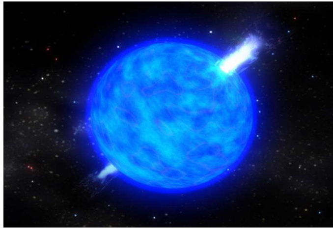
Figure 5.18 Illustration of a long-duration gamma-ray burst in the popular “collapsar” model (see Color Plate 7 for a color version of this figure). The collapse of the core of a massive star (which lost its hydrogen envelope) to a black hole generates two opposite jets moving out at a speed close to the speed of light. The jets drill a hole in the star and shine brightly towards an observer who happens to be located within the collimation cones of the jets. The jets emanating from a single massive star are so bright that they can be seen across the Universe out to the epoch when the first stars formed. Figure credit: NASA E/PO.
