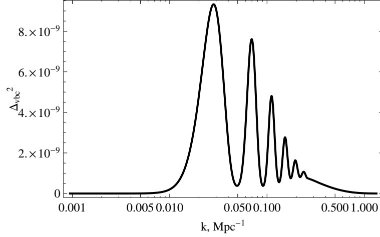
Figure 2.2 The variance of the velocity difference perturbations (in units of c ) between baryons and dark matter per \ln k as a function of comoving wavenumber k at z = 10^3 . Figure credit: Tseliaxhovich, D. & Hirata, C., Phys. Rev. D82 , 3520 (2010). Copyright 2010 by the American Physical Society.
