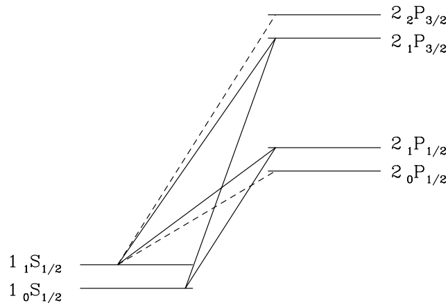
Figure 12.4 Level diagram illustrating the Wouthuysen-Field effect. We show the hyperfine splittings of the 1S and 2P levels. The solid lines label transitions that mix the ground state hyperfine levels, while the dashed lines label complementary allowed transitions that do not participate in mixing. Figure credit: Pritchard, J. R. & Furlanetto, S. R., Mon. Not. R. Astron. Soc. 367 , 1057 (2006). Copyright 2006 by the Royal Astronomical Society.
