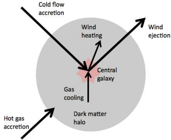
Figure 8.2 A cartoon of the “baryon cycle” in which gas flows into and out of galaxies. The central galaxy is embedded in a much larger dark matter halo. Gas accreting onto the halo follows one of two fates: (1) in large halos, some will be shocked at the virial radius and heated to high temperatures (from which point it must cool radiatively to settle onto the central galaxy), or (2) in small halos (and to some extent in larger ones), it travels along filamentary “cold flows” directly to the central galaxy. As the galaxy’s gas is turned into stars, feedback will launch winds, which both heats the halo gas (preventing it cooling onto the galaxy) and expels some gas into the IGM.
