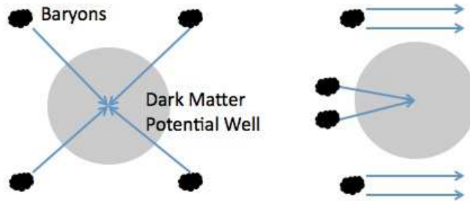
Figure 3.4 Cartoon representation of the effects of the relative streaming of baryons and dark matter on halo formation. In the absence of these motions ( left ), dark matter potential wells (which formed before recombination) attract nearby baryons, quickly building up their gas content so long as their total mass exceeds the filter mass. But when these motions are present ( right ), the baryons may move so quickly that they do not respond strongly to the dark matter potential unless they happen to pass very close to its center. In this case, baryonic accretion onto dark matter halos can be strongly suppressed (and can even affect dark matter accretion, by decreasing the total halo mass).
