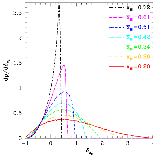
Figure 11.7 Probability distributions of the fractional bias in a simple damping wing estimate of the ionized bubble filling factor, \delta_{x_D} \equiv \bar{x}_D / (1 - Q_{\text{HII}}) - 1 . The different curves show different stages in reionization; all are computed with a semi-numerical simulation of reionization. Note that the mean is always non-zero, and the distribution becomes both wider and more biased as reionization progresses. Figure credit: Mesinger, A. & Furlanetto, S.R., Mon. Not. R. Astron. Soc. , 385 , 1348 (2008). Copyright 2008 by the Royal Astronomical Society.
