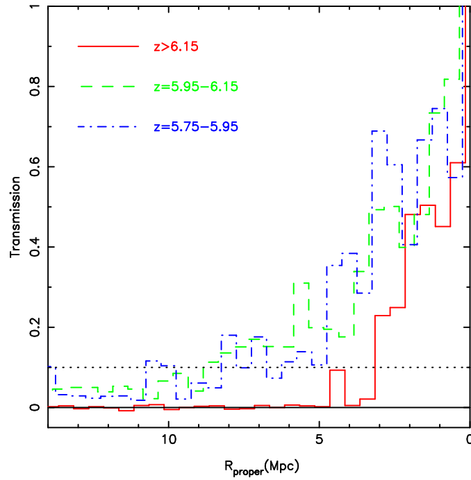
Figure 11.4 Average absorption profiles near the Lyman- \alpha line for quasars in three different redshift bins. Note that the Lyman- \alpha emission lines have been fitted and removed. The three redshift bins average over 8 ( 5.75 < z < 5.95 ), 9 ( 5.95 < z < 6.15 ), and 4 ( z > 6.15 ) quasars. The horizontal dotted line marks 10% transmission, conventionally taken as the edge of the near-zone. Figure credit: Carilli, C.L. et al., Astrophys. J. , 714 , L834 (2010). Reproduced with permission of the American Astronomical Society.
