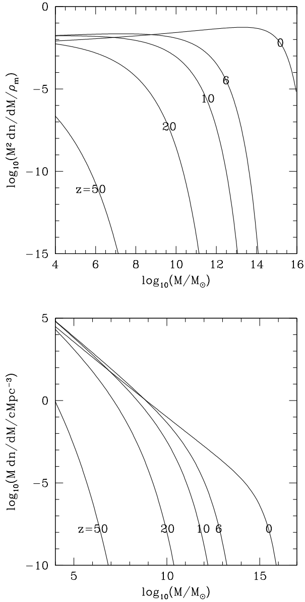
Figure 3.10 Top: The mass fraction incorporated into halos per logarithmic bin of halo mass (M^2 dn/dM)/\rho_m , as a function of M at different redshifts z . Here \rho_m = \Omega_m \rho_c is the present-day matter density, and n(M)dM is the comoving density of halos with masses between M and M + dM . The halo mass distribution was calculated based on an improved version of the Press-Schechter formalism for ellipsoidal collapse that better fits numerical simulations (see §3.4.3). Bottom: Number density of halos per logarithmic bin of halo mass, M dn/dM (in units of comoving \text{Mpc}^{-3} ), at various redshifts.
