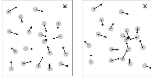
Figure 4.2 Illustration of the Zel'dovich approximation for evolution of the cosmological density field. In panel (a), we show the initial conditions for a calculation (approximating the density field as a set of discrete particles for simplicity). The arrow indicates the direction of the displacement field at the location of each particle. Panel (b) shows a later stage in the evolution. In the Zel'dovich approximation, each particle continues to move along the direction of its original displacement (generated from the potential field at the initial time). As a result, matter particles converge into sheets, filaments, and halos.
