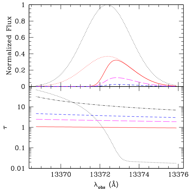
Figure 11.13 Top: Example line profiles for a galaxy at z = 10 . The upper dotted curve shows the intrinsic line profile, assumed to be a Gaussian with standard deviation 27 \text{ km s}^{-1} . The solid, long-dashed, and short-dashed curves show the observed line after reprocessing through the IGM; they place the galaxy in ionized bubbles with radii R_b = 10, 5, and 3 comoving Mpc, respectively. The lower dotted curve shows the line if we neglect resonant absorption within the ionized bubble, assuming R_b = 10 Mpc. Bottom: The dotted line shows the resonant absorption from the ionized bubble. The solid, long-dashed, short-dashed, and dot-dashed curves show the damping wing optical depth for R_b = 10, 5, 3, and 1 Mpc, respectively. Figure credit: Furlanetto, S.R. et al., Mon. Not. R. Astron. Soc. , 354 , 695 (2004). Copyright 2004 by the Royal Astronomical Society.
