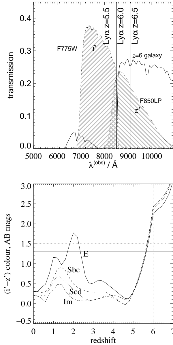
Figure 10.6 Top panel: The i' and z' bands of HST (shaded regions) on top of the generic spectrum from a galaxy at a redshift z = 6 (solid line). The Lyman- \alpha wavelength at various redshifts is also shown. Bottom panel: Models of the color-redshift tracks for different types of galaxies with non-evolving stellar populations. All of the standard galaxy types converge to have very red (i' - z') colors at high redshifts, so such galaxies can be efficiently identified with a cut in color space. The bump at z \sim 1-2 arises when the Balmer break or the 4000 \text{\AA} break redshift beyond the i' -filter. Synthetic models indicate that the Balmer break takes \sim 10^8 years to establish, providing a measure of the galaxy age. Figure credit: Bunker, A. et al., Frontiers of Astrophysics: A Celebration of NRAO's 50th Anniversary , ASP Conference Series, vol. 395, eds A. Bridle, J. Condon & G. Hunt (2008). Copyright 2008 by the Astronomical Society of the Pacific.
