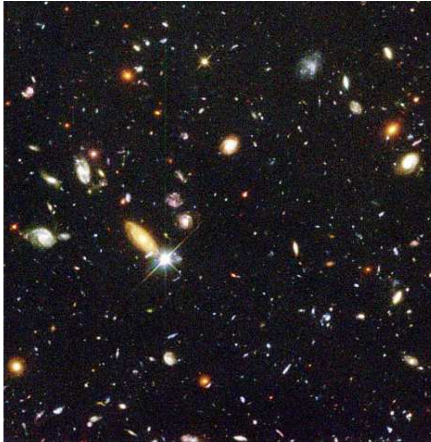
Figure 10.1 The first Hubble Deep Field (HDF) image taken in 1995 (see Color Plate 18 for a color version of this image). The HDF covers an area 2.5 arcminutes across and contains a few thousand galaxies (with a few candidates up to a redshift z \sim 6 ). The image was taken in four broadband filters centered on wavelengths of 3000, 4500, 6060, and 8140 Å, with an average exposure time of \sim 0.127 million seconds per filter.
