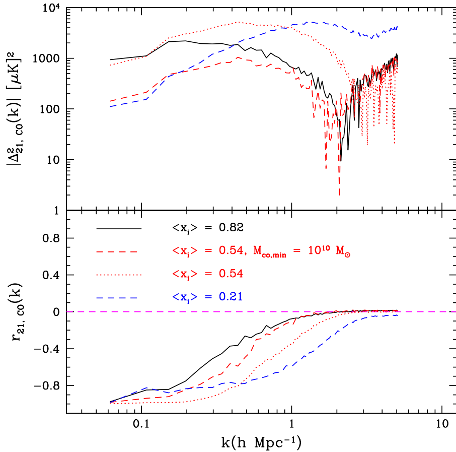
Figure 13.11 Cross-correlation between CO(2-1) emission and the spin-flip background in a numerical simulation of reionization (as in Figure 13.9). The dot-dashed, dotted, and solid curves take z = 9.8 , 7.3 , and 6.8 (or Q_{\text{HII}} = 0.21 , 0.54 , and 0.82 in this model), assuming that all galaxies emit CO(2-1). The long-dashed curve takes z = 7.3 but assumes that only massive galaxies emit CO. The top and bottom panels show the absolute value of the cross-power spectrum and the cross-correlation coefficient, respectively. Figure credit: Lidz, A. et al., Astrophys. J. 741 , 70 (2011). Reproduced with permission of the American Astronomical Society.
