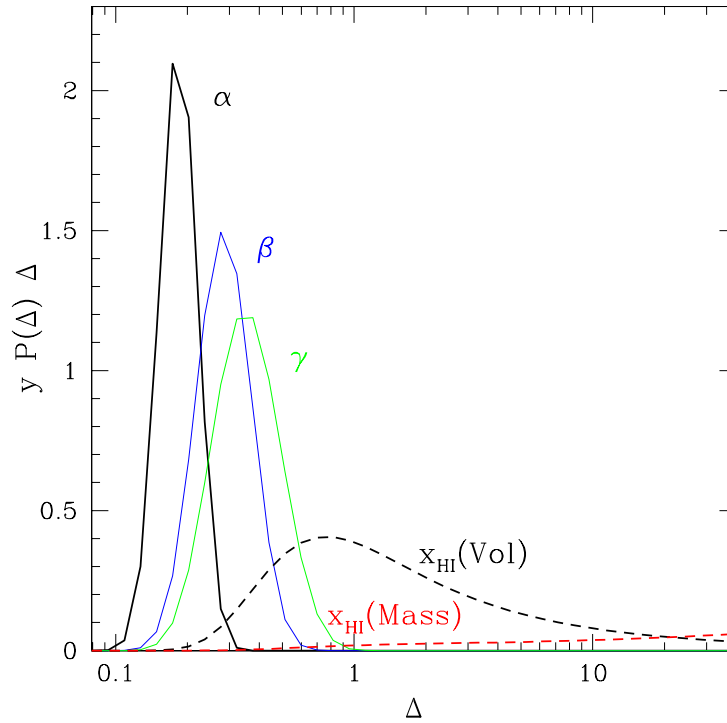
Figure 4.16 Logarithmic integrand y(1 + \delta)p(\delta) \propto \langle y \rangle in a simple model of the IGM density distribution; here \Delta = 1 + \delta . The three solid curves use the optical depth in the Lyman- \alpha , Lyman- \beta , and Lyman- \gamma transitions (from left to right) for y ; they thus show the integrands in equation (4.27) and its analogs for the higher-order transitions. The dashed lines show a similar calculation for the neutral fraction, with both volume and mass weighting (the latter peaks to the right of the plot). All curves assume a uniform \Gamma_{12} = 0.04 at z = 6.15 and an isothermal temperature-density relation. Figure credit: Oh, S. P. & Furlanetto, S. R., Astrophys. J. , 620 , L9 (2005). Reproduced with permission of the American Astronomical Society.
