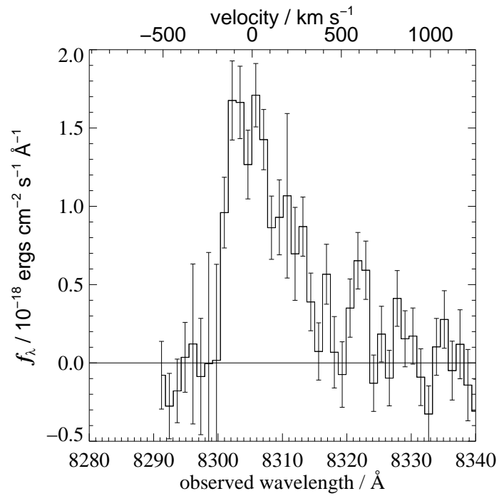
Figure 10.5 The Lyman- \alpha emission line of a typical i' -dropout galaxy SBM03# at z = 5.83 . Figure credit: Stanway, E., et al. Astrophys. J. 607 , 704 (2004). Reproduced with permission of the American Astronomical Society.
