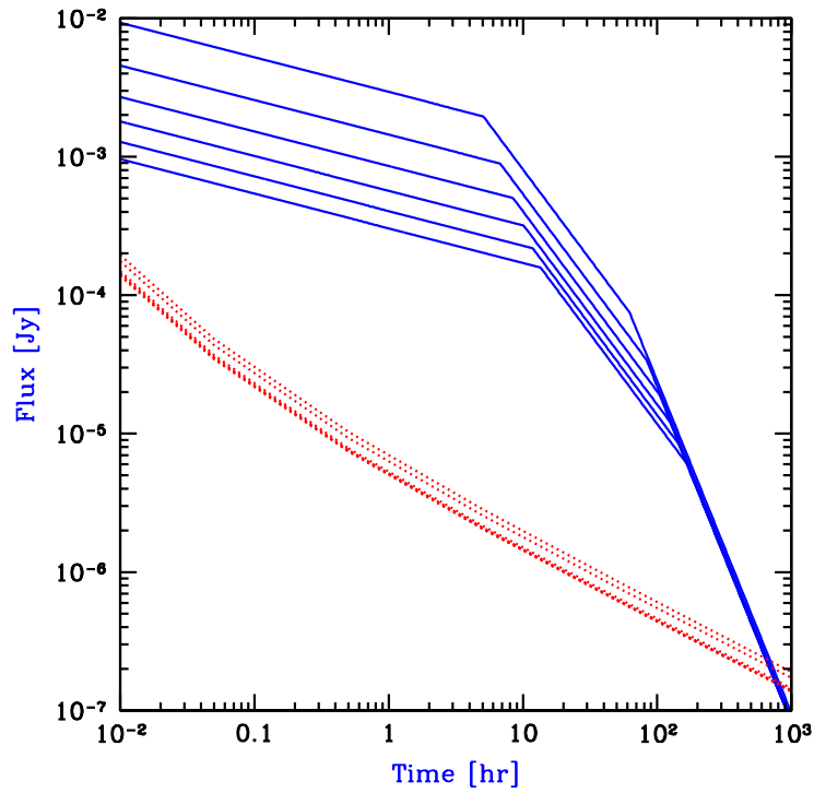
Figure 10.8 Detectability of high-redshift GRB afterglows as a function of time since the GRB explosion as measured by the observer. The GRB afterglow flux (in Jy) is shown at the redshifted Lyman- \alpha wavelength (solid curves). Also shown (dotted curves) is a crude estimate for the spectroscopic detection threshold of JWST , assuming an exposure time equal to 20% of the time since the GRB explosion. Each set of curves spans a sequence of redshifts: z = 5, 7, 9, 11, 13, 15 , respectively (from top to bottom). Figure credit: Barkana, R., & Loeb, A. Astrophys. J. 601 , 64 (2004). Reproduced with permission of the American Astronomical Society.
