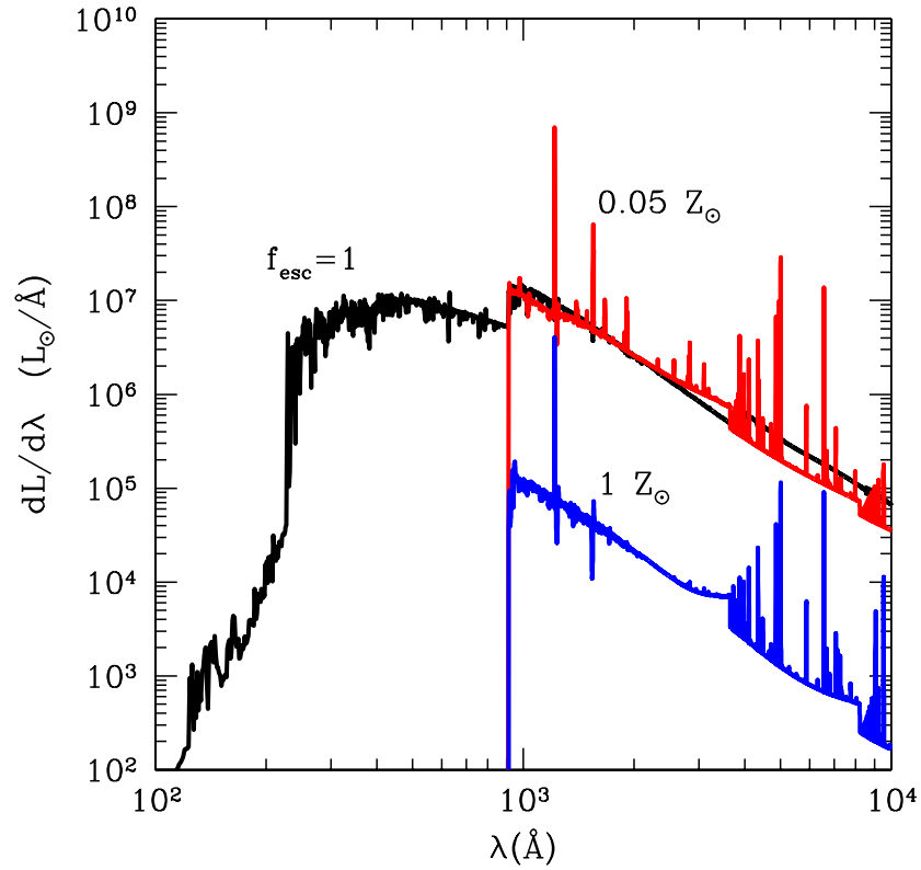
Figure 8.8 Effects of host galaxy absorption on stellar spectra. The curve extending to short wavelengths is the raw stellar spectrum (identical to the curve with binaries in Fig. 8.7 b ). The other two curves show the spectrum assuming that all ionizing photons are absorbed by the galaxy ISM and reprocessed into emission lines at longer wavelengths. The upper curve assumes Z = 0.05 Z_{\odot} ; the lower curve assumes solar metallicity for both the stars and ISM. The latter is shifted down by two orders of magnitude for clarity of presentation. Generated using the BPASS population synthesis code ( http://www.bpass.org.uk ).
