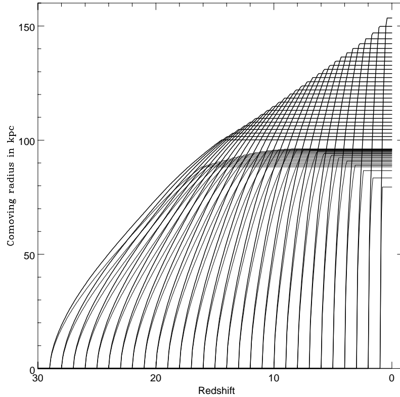
Figure 6.9 Shell sizes as a function of redshift, in comoving distance, from galaxies with M_h = 2 \times 10^6 M_\odot forming at redshifts from z = 29 to z = 1 . The model assumes a star formation efficiency near unity. The upper set of curves take f_d = 1 , while the lower set take f_d = 0 . The expansion is assumed to stop when the bubble interior falls below T = 15,000 K. Figure credit: Tegmark, M., Silk, J., & Evrard, A., Astrophys. J. 417 , 54 (1993). Reproduced with permission of the American Astronomical Society.
