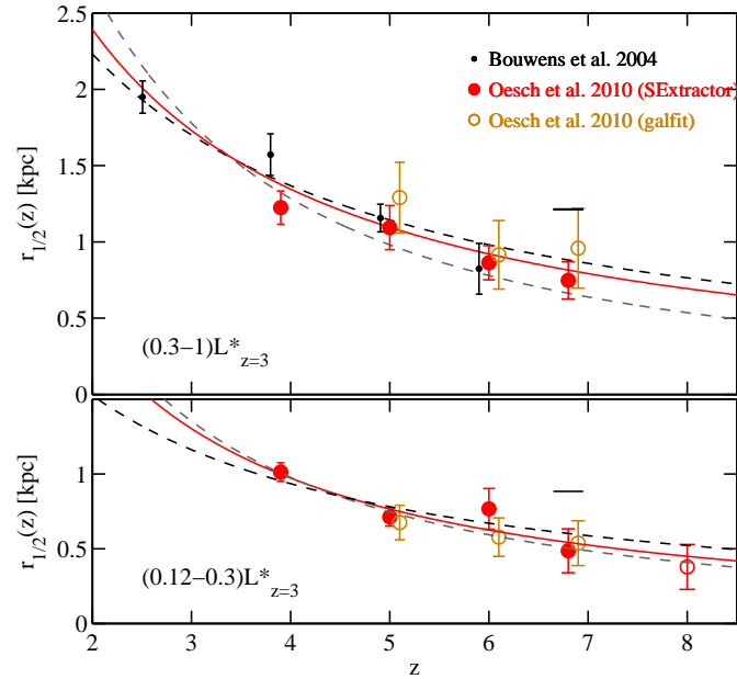
Figure 8.3 Observed evolution of the mean half-light radius of galaxies across the redshift range 2 < z < 8 in two bins of fixed intrinsic luminosity: (0.3-1)L_{*}(z = 3) (top) and (0.12-0.3)L_{*}(z = 3) (bottom), where L_{*}(z = 3) is the characteristic luminosity of a galaxy at z = 3 (equation 10.3). Different point types correspond to different methods of analysing the data. The dashed lines indicate the scaling expected for a fixed halo mass ( \propto (1+z)^{-1} ; black) or at fixed halo circular velocity ( \propto (1+z)^{-3/2} ; gray). The central solid lines correspond to the best-fit to the observed evolution described by \propto (1+z)^{-m} , with m = 1.12 \pm 0.17 for the brighter luminosity bin, and m = 1.32 \pm 0.52 at fainter luminosities. Figure credit: Oesch, P. A., et al., Astrophys. J. 709 , L21 (2010). Reproduced with permission of the American Astronomical Society.
