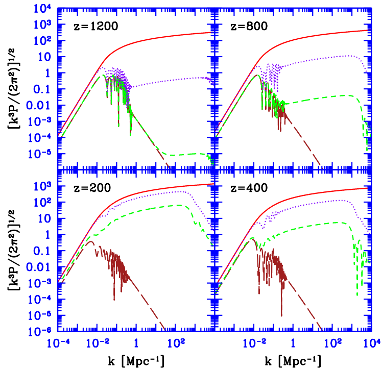
Figure 2.6 Power spectra for density and temperature fluctuations versus comoving wavenumber at four different redshifts. The curves show the CDM density (solid), baryon density (dotted), baryon temperature (short-dashed) and photon temperature (long-dashed). These curves do not include the relative streaming of the baryons and cold dark matter. Figure credit: Naoz, S. & Barkana, R., Mon. Not. R. Astron. Soc. , 362 , 1047 (2005). Copyright 2005 by the Royal Astronomical Society.
