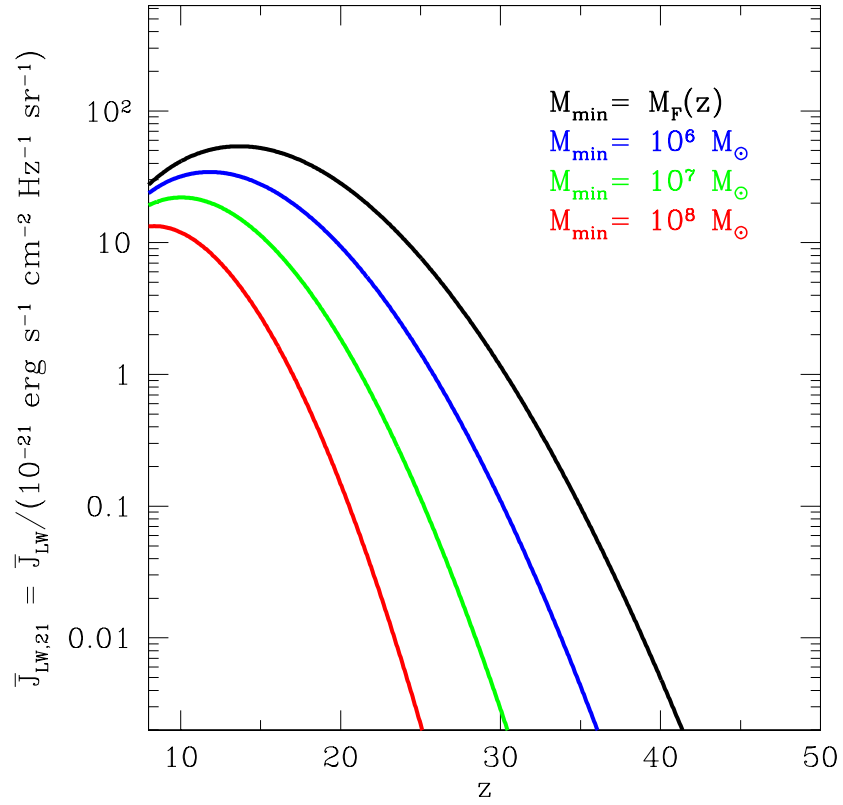
Figure 6.3 Evolution of the specific intensity of the metagalactic radiation field in the Lyman-Werner band at high redshifts. The solid lines show the amplitude of the radiation field over time, taking several different mass thresholds for star-forming halos: M_{\text{min}} = M_F(z) (the filtering mass), 10^6 , 10^7 , and 10^8 M_\odot , from top to bottom. The curves assume f_* = 0.1 ; all of the curves are proportional to this value.
