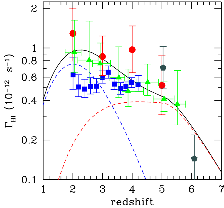
Figure 4.8 Measurements of the ionizing background at moderate redshifts (points with error bars), and models of it (curves). The measurements use the mean transmission of the Lyman- \alpha forest as described in this section as well as the proximity effect (see §11.3.2). The curves base the emissivity and mean free path inputs on measured values at z < 6 and use the method described in §4.4. The solid line shows the total \Gamma , while the dashed curves peaking at z \sim 4 and z \sim 2 show the separate contributions from star-forming galaxies and quasars, respectively. Figure credit: Haardt, F. & Madau, P., Astrophys. J. , submitted (2011), astro-ph/1105.2039; observational measurements collected from references therein. Reproduced with permission from the American Astronomical Society.
