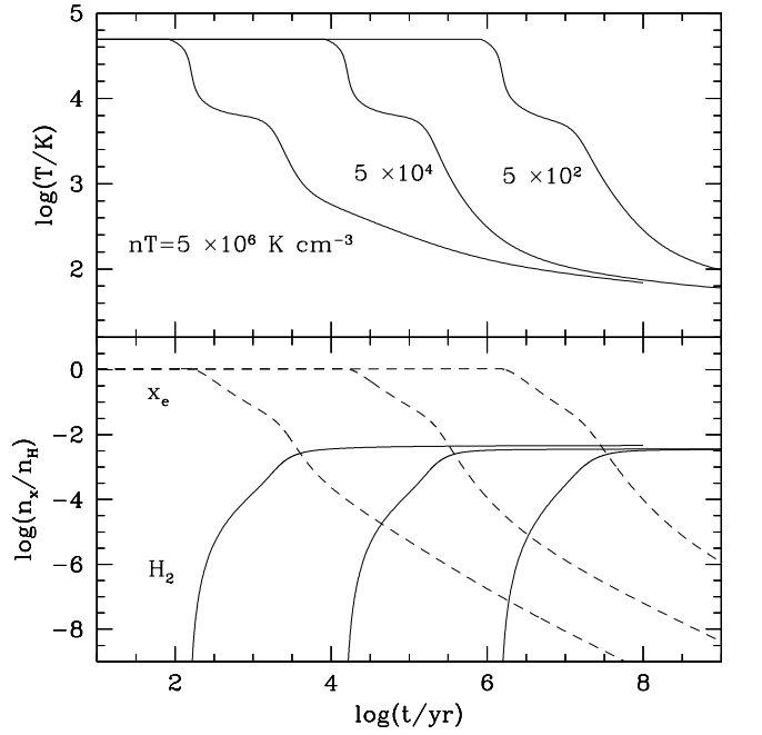
Figure 5.11 \text{H}_2 formation in initially ionized gas. The top panel shows the temperature evolution of gas at three different initial pressures, assuming isobaric cooling (the three models are offset in time for clarity of presentation). The bottom panel shows the molecular fractions (solid curves) and the free electron fractions (dashed curves) for the same three models. Note how f_{\text{H}_2} approaches a constant limit in all three cases. Figure credit: Oh, S. P. & Haiman, Z., Astrophys. J. , 569 , 558 (2002). Reproduced with permission of the American Astronomical Society.
