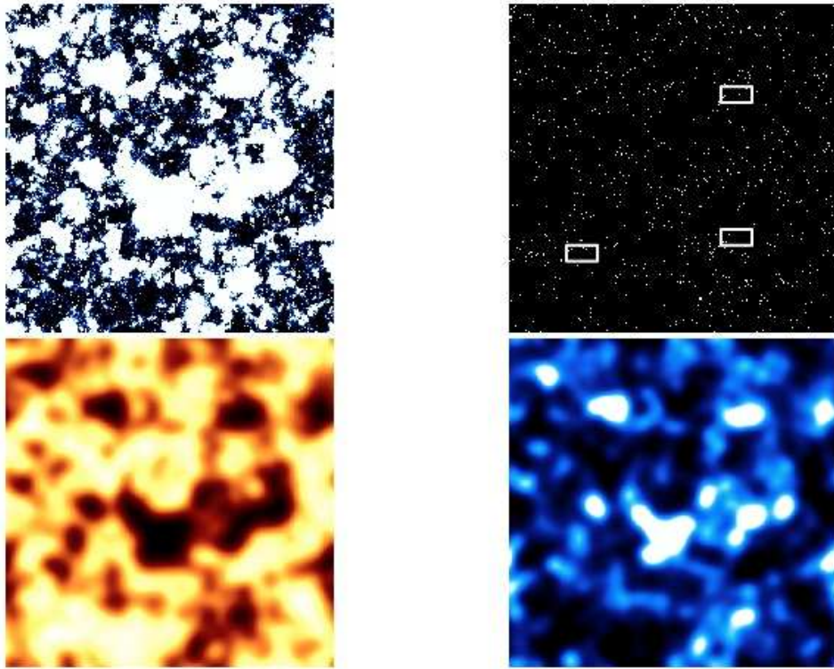
Figure 13.10 Schematic illustration of the cross-correlation between the spin-flip background and galaxy probes (see Color Plate 32 for a color version of this figure). Each panel shows a slice from a numerical simulation \sim 185 Mpc across. Upper left: Map of the ionized fraction midway through reionization (ionized regions are shown in white). Upper right: Map of the galaxy field. White squares show regions \sim 4 \times 8 arcmin across; these are each equivalent to four adjacent pointings of the James Webb Space Telescope. Lower left: Spin-flip background from this slice. Lower right: Galaxy map smoothed over a 6 arcmin beam, as might be observed in an intensity mapping measurement. Note the strong large-scale anti-correlation between the bottom two figures. Figure credit: A. Lidz.
