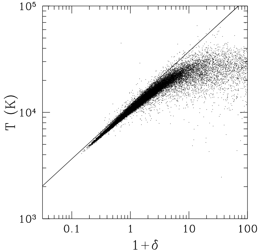
Figure 4.7 Temperature-density relation at z = 4 in a cosmological simulation (points), together with analytic prediction based on linear perturbation theory and equation (4.22). Note the near power-law relation, except at very high densities where the complex physics of nonlinear structure formation begin to matter. Figure credit: Hui, L. & Gnedin, N. Y. Mon. Not. R. Astron. Soc. 292 , 27 (1997). Copyright 1997 by the Royal Astronomical Society.
