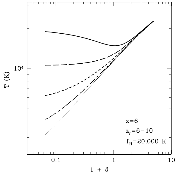
Figure 9.13 IGM temperature-density relation following H I reionization. All curves assume z = 6 and take a post-reionization temperature of T_H = 20,000 K. The solid, long-dashed, short-dashed, dot-dashed, and dotted curves set the reionization redshift at z_r = 6, 7, 8, 9, and 10 , respectively. Figure credit: Furlanetto, S. R., & Oh, S. P., Astrophys. J. 701 , 94 (2009). Reproduced with permission of the American Astronomical Society.
