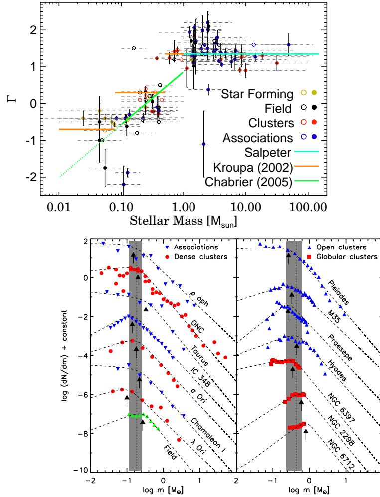
Figure 5.9 Upper panel : The derived power-law index, \Gamma , of the IMF in nearby star forming regions, clusters and associations of stars within the Milky Way galaxy, as a function of sampled stellar mass (points are placed in the center of the \log m_* range used to derive each index, with the dashed lines indicating the full range of masses sampled). The colored solid lines represent three analytic IMFs. Bottom panel : The present-day IMF in a sample of young star-forming regions, open clusters spanning a large age range, and old globular clusters. The dashed lines represent power-law fits to the data. The arrows show the characteristic mass of each fit, with the dotted line indicating the mean characteristic mass amongst the clusters in each panel, and the shaded region showing the standard deviation of the characteristic masses in that panel. The observations are consistent with a single underlying IMF. See Color Plate 6 for a color version of this figure. Figure credit: Bastian, N., Covey, K. R., & Meyer, M. R., Ann. Rev. Astr. & Astrophys. 48 (2010). Copyright 2010 by Annual Reviews.
