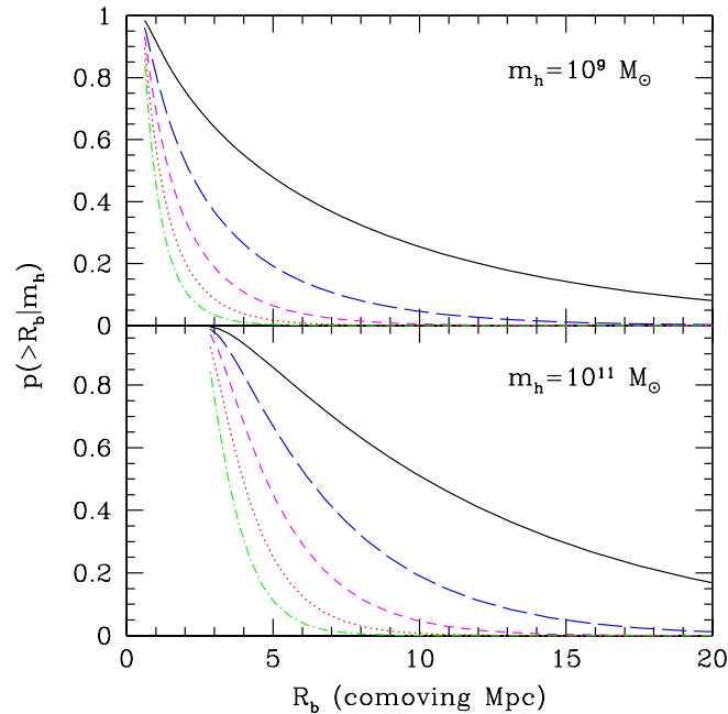
Figure 11.14 Probability that halos with m_h = 10^9 and 10^{11} M_\odot reside in ionized bubbles larger than a given radius R_b . Here we use the excursion set model of reionization with \zeta = 40 ; the bubble sizes are relatively independent of this choice, for a fixed Q_{\text{HII}} , but the halo populations themselves are highly-redshift dependent. In each panel, the curves correspond to z = 12 ( Q_{\text{HII}} = 0.74 , solid), z = 13 ( Q_{\text{HII}} = 0.48 , long dashed), z = 14 ( Q_{\text{HII}} = 0.3 , short-dashed), z = 15 ( Q_{\text{HII}} = 0.19 , dotted), z = 16 ( Q_{\text{HII}} = 0.11 , dot-dashed), Figure credit: Furlanetto, S.R. et al., Mon. Not. R. Astron. Soc. , 354 , 695 (2004). Copyright 2004 by the Royal Astronomical Society.
