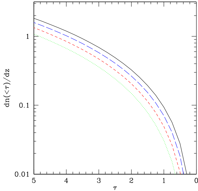
Figure 11.9 A model for the expected cumulative number of Lyman- \alpha forest transmission features at z = 6.1 if the IGM has Q_{\text{HII}} = 0.9, 0.85, 0.8, and 0.75 (solid, long-dashed, short-dashed, and dotted curves, respectively). The calculation uses the excursion set model for reionization (see §9.4) and an inhomogeneous IGM density distribution calibrated to simulations at lower redshifts. Figure credit: Furlanetto, S.R. et al., Mon. Not. R. Astron. Soc. , 354 , 695 (2004). Copyright 2004 by the Royal Astronomical Society.
