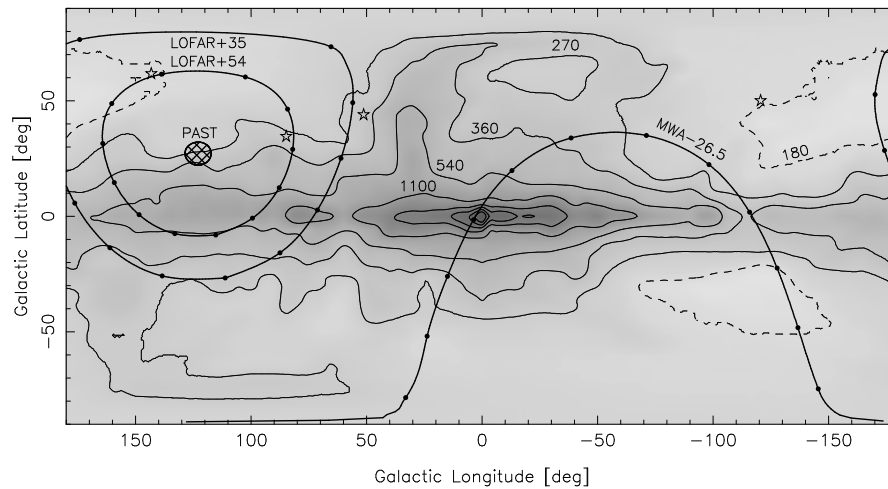
Figure 12.11 Brightness temperature of the radio sky at 150 MHz in Galactic coordinates. Contours are drawn at 180 (dashed), 270, 360, 540, 1100, 2200, 3300, 4400, and 5500 K. A potential survey field at the North celestial pole is cross-hatched. Heavy lines indicate constant declinations: -26.5^\circ , +35^\circ , and +54^\circ with dots to mark 2 hour intervals of time (these are ideal for two other existing experiments, the Murchison Wide-field Array or MWA and LOFAR). Star symbols indicate the coordinates of four bright z > 6.2 quasars. Figure credit: Landecker, T. L. & Weilebinski, R., Proc. Astron. Soc. Aust. 1 , 210 (1969); Furlanetto, S. R., Oh, S. P., & Briggs, F. H., Physics Reports 433 , 181 (2006). Copyright 2006 by Elsevier.
