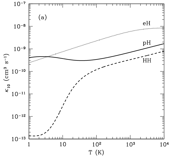
Figure 12.3 De-excitation rate coefficients for H-H collisions (dashed line), H-e - collisions (dotted line), and H-p collisions (solid line). Note that the net rates are also proportional to the densities of the individual species, so H-H collisions still dominate in a weakly-ionized medium. Figure credit: Furlanetto, S. R. & Furlanetto, M. R., Mon. Not. R. Astron. Soc. 379 , 130 (2007). Copyright 2007 by the Royal Astronomical Society.
