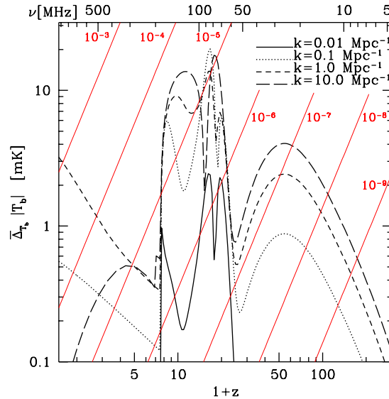
Figure 12.17 Redshift evolution of the angle-averaged 21 cm power spectrum in a model with reionization ending at z = 6.5 . We show the amplitude for k = 0.01 \text{ Mpc}^{-1} (solid curve), k = 0.1 \text{ Mpc}^{-1} (dotted curve), k = 1 \text{ Mpc}^{-1} (short-dashed curve), and k = 10 \text{ Mpc}^{-1} (long-dashed curve). After reionization, the fluctuations trace neutral gas inside galaxies and DLAs and so mirror the galaxy power spectrum. The diagonal curves show contours of a fixed fraction of the sky brightness as a function of frequency. Figure credit: Pritchard, J. R. & Loeb, A. Phys. Rev. D 78 , 103511 (2008). Copyright 2008 by the American Physical Society.
