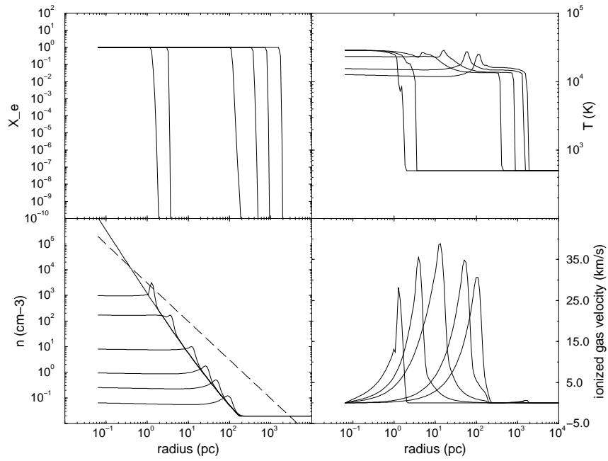
Figure 6.6 Evolution of a cosmological halo as an ionization front propagates through it. The simulation takes a single 200 M_{\odot} star at z = 18.2 in a halo of total mass 7 \times 10^5 M_{\odot} . Clockwise from top left, the panels show the ionized fraction, the temperature, the (outward) velocity, and the density profile. Each panel shows snapshots at 63, 82, 95, 127, 317, and 2200 kyr (left to right in all panels except bottom left, where they are top to bottom). In the bottom left, the dashed line shows the minimum density required to trap the ionization front. Figure credit: Whalen, D. et al. Astrophys. J. 610 , 14 (2004). Reproduced with permission of the American Astronomical Society.
