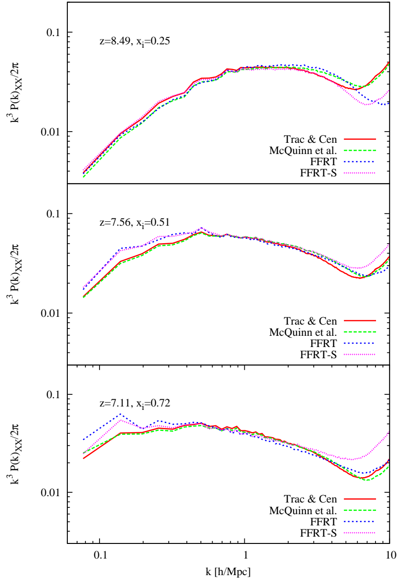
Figure 9.10 Comparison of the power spectrum of the ionization field in the radiative transfer and semi-numerical models of reionization. The three panels correspond to the columns of Fig. 9.9, and the curves correspond to the four models shown there as well. Note the close match in the predictions of all four models on scales k < 8h/\text{Mpc} , although the semi-numerical schemes do overpredict the power on very large scales in the late stages of reionization. The differences at k > 8h/\text{Mpc} are due to shot noise, which differs between the schemes. Figure credit: Zahn, O. et al., Mon. Not. R. Astron. Soc. , 414 , 727 (2011). Copyright 2011 by the Royal Astronomical Society.
