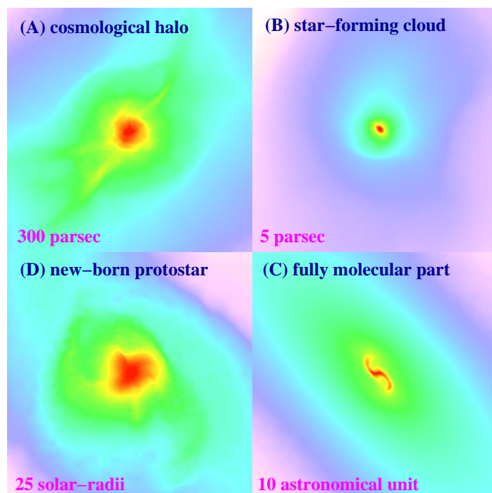
Figure 5.6 Projected gas distribution around a primordial protostar from a numerical simulation (see also Color Plate 4 for a color version of this figure). Shown is the gas density of a single object on different spatial scales: (a) the large-scale gas distribution around the cosmological mini-halo; (b) the self-gravitating, star-forming cloud; (c) the central part of the fully molecular core; and (d) the final protostar. Figure credit: Yoshida, N., Omukai, K., & Hernquist, L. Science 321 , 669 (2008). Copyright 2008 by the American Association for the Advancement of Science.
