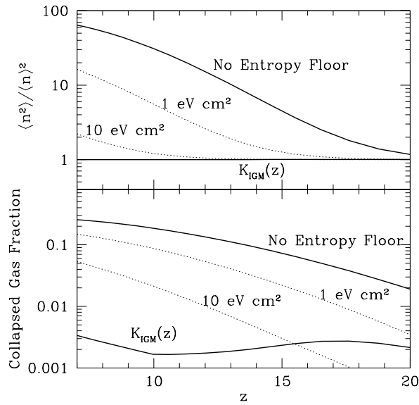
Figure 9.14 Effects of the IGM “entropy floor” on gas clumping from virialized minihalos ( top panel ) and the collapse fraction of gas onto dark matter halos ( bottom panel ). In each panel, the uppermost solid curve shows the model calculation with no entropy injection. The lower solid curve, labeled K_{\text{IGM}}(z) , shows the effect of a numerical calculation of entropy injection via photoionization and subsequent recombination (which decreases K through radiative cooling). The two dotted curves show estimates for entropy injection at fixed levels (perhaps by an X-ray background). Figure credit: Oh, S. P. & Haiman, Z. Mon. Not. R. Astron. Soc. 346 , 456 (2005). Copyright 2005 by the Royal Astronomical Society.
