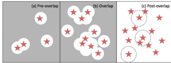
Figure 9.2 Cartoon of the three phases of reionization. (a) In the pre-overlap phase, galaxies are uncommon, and their H II regions grow in relative isolation. In practice, galaxies are highly-clustered, so even in this stage some of those H II regions meet each other. Nevertheless, the average ionizing background grows fairly slowly during this epoch. (b) Once galaxies become sufficiently common, the overlap phase, in which ionized bubbles rapidly intersect, begins. During this phase, the ionizing background can increase relatively rapidly as sources are quickly added to each discrete H II region. (c) Once nearly all of the IGM is ionized, the post-overlap phase begins, in which ionizing photons are absorbed by dense clouds of optically thick gas, or Lyman-limit systems. The finite mean free path of ionizing photons, even in a “reionized” universe, is represented here by the dashed circles surrounding a few of the sources.
