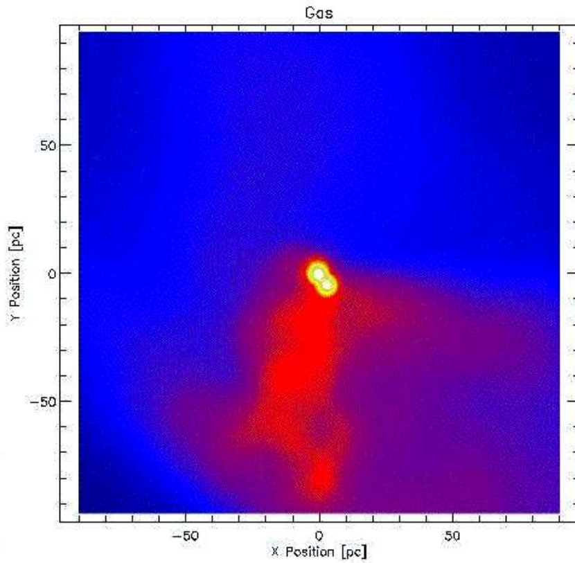
Figure 7.6 Numerical simulation of the collapse of an early dwarf galaxy with a virial temperature just above the cooling threshold of atomic hydrogen and no H_2 (see Color Plate 14 for a color version of this figure). The image shows a snapshot of the gas density distribution 500 million years after the Big Bang, indicating the formation of two compact objects near the center of the galaxy with masses of 2.2 \times 10^6 M_\odot and 3.1 \times 10^6 M_\odot , respectively, and radii < 1 pc. Sub-fragmentation into lower mass clumps is inhibited because hydrogen atoms cannot cool the gas significantly below its initial temperature. These circumstances lead to the formation of supermassive stars that inevitably collapse to make massive seeds for supermassive black holes. The simulated box size is 200 pc on a side. Figure credit: Bromm, V. & Loeb, A. Astrophys. J. 596 , 34 (2003). Reproduced with permission of the American Astronomical Society.
