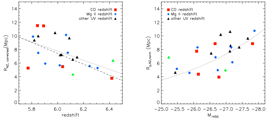
Figure 11.5 Left : Measured radii of near zones in a set of high- z quasars; the symbols denote the method used to compute the quasar’s redshift. All near-zone measurements have been scaled to a common quasar luminosity using the R_b relation in equation (11.18) to better illustrate the trend with redshift. Typical errors in the near-zone size are \sim 1 Mpc. The two lines are fits to the trend with redshift. Right : Dependence of the near-zone size on quasar absolute magnitude; all the data points have been scaled to a common redshift using the mean relation in the left-hand panel to better illustrate the behavior with luminosity. The dotted line shows R_b \propto \dot{N}_Q^{1/3} with arbitrary scaling; note that it is not a fit but is merely meant to guide the eye. Figure credit: Carilli, C.L. et al., Astrophys. J. , 714 , L834 (2010). Reproduced with permission of the American Astronomical Society.
