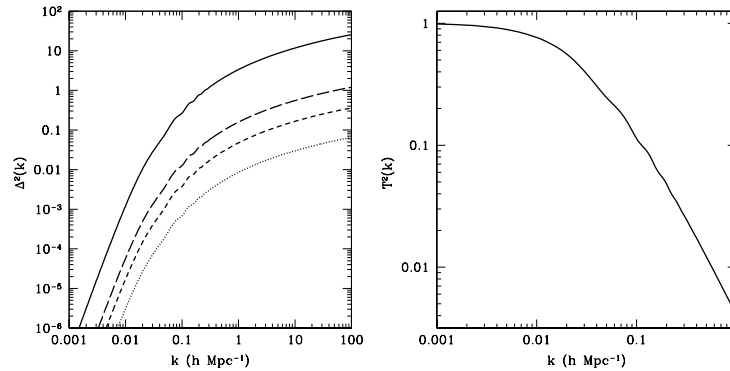
Figure 2.1 Left : The matter power spectrum in our fiducial cosmology at z = 0, 5, 10, and 25 , from top to bottom. Right : The corresponding transfer function. Computed using the publicly available code CAMB ( http://camb.info ).
