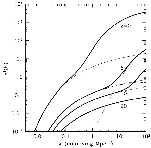
Figure 3.17 Dark matter density power spectrum predictions over a range of redshifts in the context of the halo model. The solid curves show the halo model prediction including only linear bias, while the dashed curves show the corresponding linear theory predictions. For the z = 6 curves, we also show separately the one-halo and two-halo terms with the dotted curves; these dominate at large and small k , respectively.
