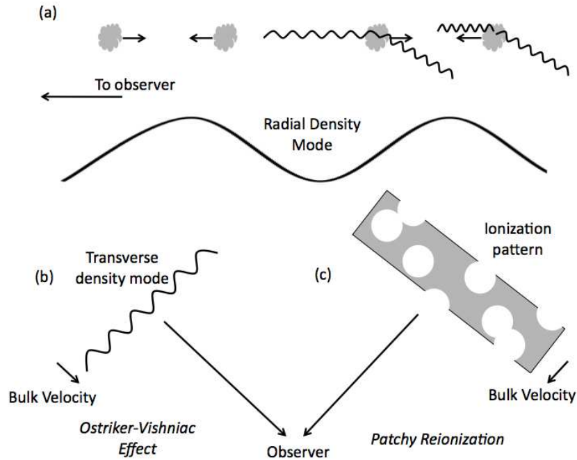
Figure 13.4 Cartoon of the kinetic Sunyaev-Zel'dovich effect. (a) We imagine a plane wave perturbation oriented along the line of sight. The density perturbations generate peculiar velocities as matter falls into the overdense regions. CMB photons that scatter on the far side of these perturbations get blueshifted (on average), but photons that scatter on the near side get redshifted. To linear order, there is a net cancellation of the two frequency shifts. (b) However, at higher order the Doppler shifts do not cancel out, so long as another density mode affects the scattering. Here, we imagine a region with a net velocity toward the observer and a density mode transverse to the line of sight. Overdensities across the sky will generate a stronger blueshift than the underdensities thanks to their larger optical depth. On small scales, these will not cancel with other structures along the line of sight. This density modulation is called the Ostriker-Vishniac effect . (c) Alternatively, we imagine another region with a bulk velocity directed toward the observer, in which the ionized fraction varies spatially due to discrete H II regions during reionization. This modulation is associated with patchy reionization . Both nonlinear effects (b) and (c) source CMB temperature fluctuations on small angular scales.
