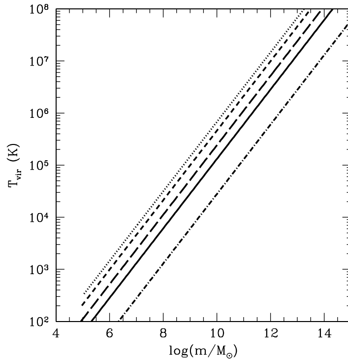
Figure 3.7 Virial temperature over a wide range of halo masses and redshifts (equation 3.30). The dotted, short-dashed, long-dashed, solid, and dot-dashed curves take z = 30, 20, 10, 5, and 0, respectively. For simplicity we assume fully-ionized gas in all these halos, though the low-mass objects may actually accrete neutral gas.
