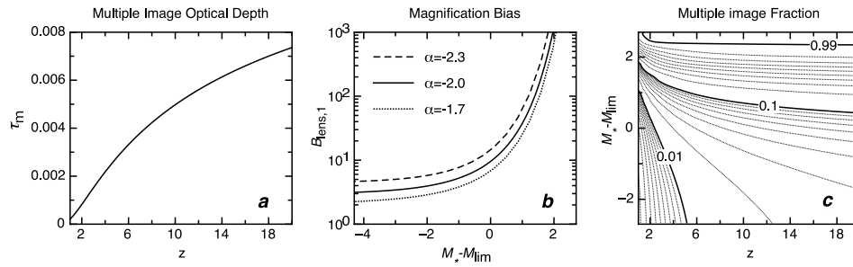
Figure 10.13 Probability for multiple imaging of high redshift galaxies by an unevolving population of SIS lenses. (a): Lensing probability \tau_m for obtaining multiple images as a function of source redshift. (b): Magnification bias as a function of the difference between the characteristic magnitude of a galaxy M_* (assuming a Schechter luminosity function) and the limiting survey magnitude M_{\text{lim}} . Three values of the faint-end slope of the luminosity function (labeled by \alpha here) are shown. (c): Contours of the fraction of multiply-imaged sources as a function of source redshift and (M_* - M_{\text{lim}}) , assuming a faint end slope for their luminosity function of -2 . Figure credit: Wyithe, J. S. B., et al., Nature 469 , 7329 (2011). Copyright 2011 by Nature Publishing Group.
