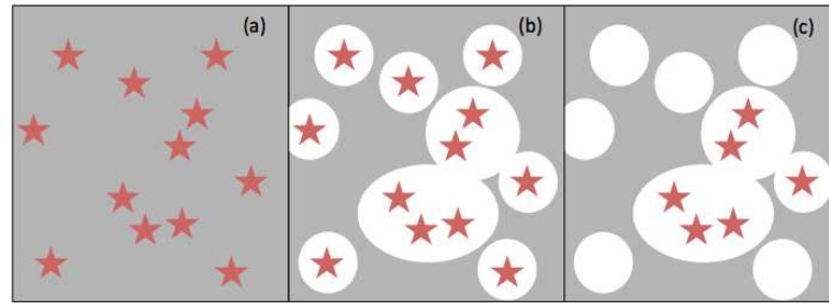
Figure 11.17 Toy model for the excess clustering induced in a Lyman- \alpha selected galaxy population during reionization. (a) First, assume that we have a randomly-distributed galaxy population. A continuum survey, sensitive to all these galaxies, would detect no clustering signal. (b) The H II regions generated by these galaxies: note that, when galaxies are close together, their H II regions overlap, producing long stretches of nearly ionized gas through which Lyman- \alpha photons can easily propagate. (c) A LAE survey would only see galaxies inside these large H II regions, all of which have neighbors (by construction), so the apparent clustering would be large even though the underlying population is randomly distributed.
