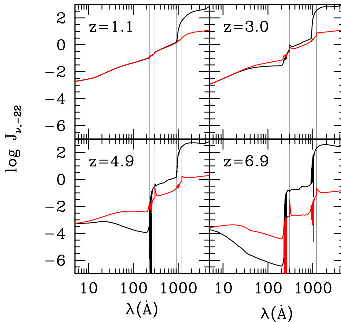
Figure 4.13 Metagalactic ionizing background spectrum at z = 1.1, 3.0, 4.9, and 6.9 , in the same theoretical model as Figure 4.8. The units correspond to J_{\nu,-22} = J_{\nu}/(10^{-22} \text{ erg cm}^{-2} \text{ s}^{-1} \text{ Hz}^{-1} \text{ sr}^{-1}) . The dark and light lines show models with galaxies and quasars and only quasars, respectively. The vertical lines bracket the Lyman-series transitions of H I and He II. Figure credit: Haardt, F. & Madau, P., Astrophys. J. , submitted (2011), astro-ph/1105.2039. Reproduced with permission of the American Astronomical Society.
