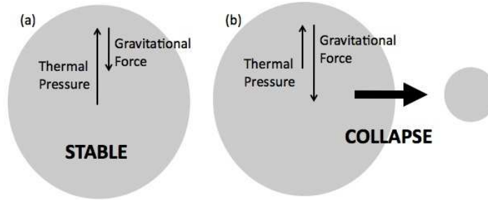
Figure 3.2 The Jeans criterion for gravitational collapse of baryonic material. In (a), the outward pressure gradient exceeds the inward gravitational force, so the region is stable. In (b), the opposite is true, and the resulting instability causes runaway collapse. Note that, if the pressure changes over time, a time-averaged pressure restoring force must be used, as described in §3.2.1.
