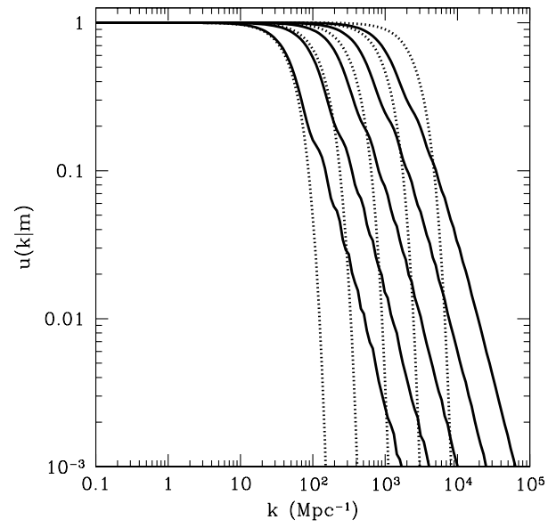
Figure 3.16 Fourier transforms of the normalized halo density profiles for a series of halos at z = 6 . The solid lines show the profiles for halos with NFW profiles and m = 10^6, 10^7, 10^8, 10^9, \text{ and } 10^{10} M_{\odot} , from right to left (equation 3.56). The dotted lines show the Gaussian profiles of equation (3.59), with the same value of r_s .
