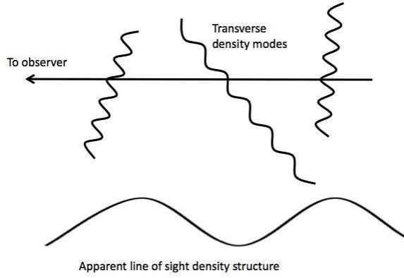
Figure 4.11 Illustration of aliasing in the Lyman- \alpha forest. The observer can only measure structure along the line of sight. However, density modes transverse to that skewer can still leave imprints in the one-dimensional field where they intersect it. The superposition of many such modes can mimic large-scale fluctuations along the line of sight, aliasing power from small to large scales.
