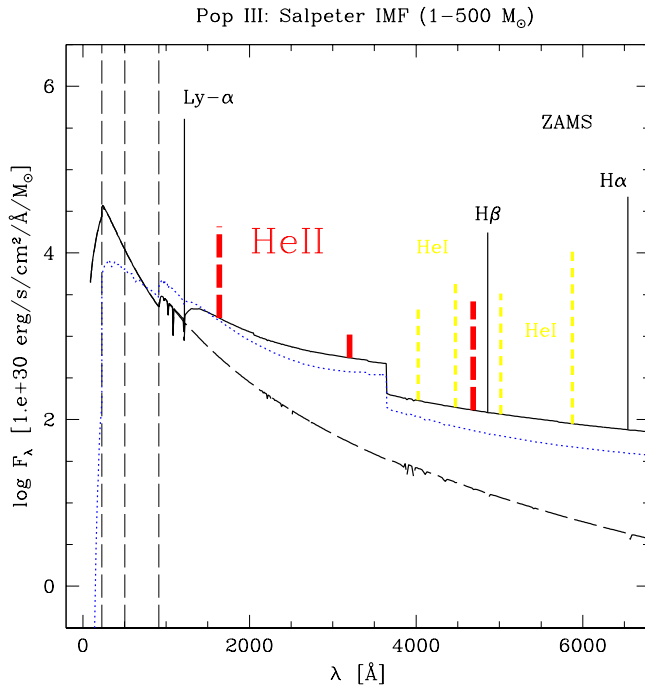
Figure 5.15 Spectral energy distribution of a cluster of Population III stars with a Salpeter IMF ranging from 1–500 M_{\odot} (solid line), all of which have just entered the main sequence. Nebular reprocessing and recombination line emission are included assuming that f_{\text{esc}} = 0 ; emission lines are shown with solid, short-dashed, and long-dashed lines for H I, He I, and He II, respectively. The pure stellar continuum (neglecting nebular emission) is shown by the long-dashed line. The contrasting case of a Population II cluster with Z = 0.02 Z_{\odot} and a Salpeter IMF ranging from 1–150 M_{\odot} is shown by the dotted line. The vertical dashed lines indicate the ionization potentials of H I, He I, and He II (from right to left). Figure credit: Schaerer, D., A & A , 382 , 28 (2002).
