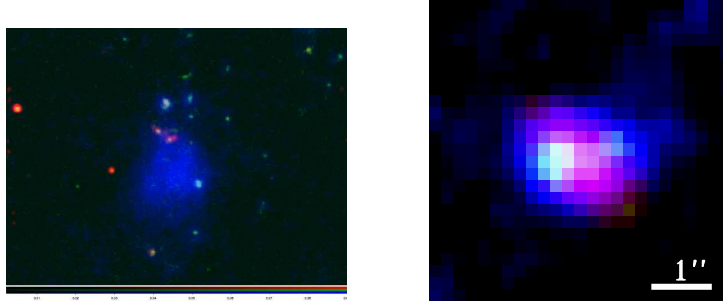
Figure 11.12 Left : A false color image of a Lyman- \alpha blob (LAB) at a redshift z = 2.656 . The hydrogen Lyman- \alpha emission is shown in blue, and images in the optical V-band and the near-infrared J and H bands are shown in green and red, respectively. Note the compact galaxies lying near the northern (top) end of the LAB. The Lyman- \alpha image was obtained using the SuprimeCam imaging camera on the Subaru Telescope, and the V, J, and H band images were obtained using the ACS and NICMOS cameras on the Hubble Space Telescope. This LAB was originally discovered by the Spitzer Space Telescope. Image credit: Prescott, M., & Dey, A. (2010). Right : A false color image of an LAB at a redshift z = 6.6 , obtained from a combination of images at different infrared wavelengths. See Color Plate 25 for a color version of this figure. Image credit: Ouchi, M. et al. Astrophys. J. 696 , 1164 (2009). Reproduced with permission of the American Astronomical Society.
