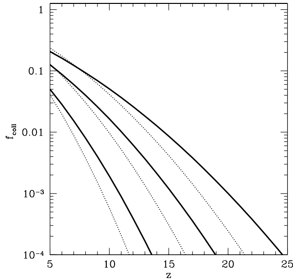
Figure 3.12 The collapse fraction of dark matter halos at high redshifts. The solid curves show f_{\text{coll}} computed from the mass function of equation (3.46), which is motivated by ellipsoidal collapse with parameters determined by a fit to numerical simulations. From top to bottom the three curves show the fraction of mass in halos with T_{\text{vir}} > 10^3 , 10^4 , and 10^5 K. The dotted curves use the original Press-Schechter form in equation (3.38).
