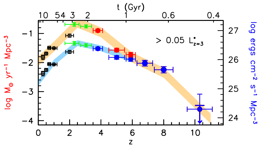
Figure 10.10 The star formation rate density (left vertical axis) or luminosity density (right vertical axis) as functions of redshift (lower horizontal axis) and cosmic time (upper horizontal axis), for galaxies brighter than an AB magnitude of -17.7 (corresponding to 0.05L_* at z = 3 ). The conversion from observed UV luminosity to star formation rate assumed a Salpeter IMF for the stars. The upper curves includes dust correction based on estimated spectral slopes of the observed UV continuum. Figure credit: Bouwens, R., et al., Astrophys. J. , 737 , 90 (2011). Reproduced with permission of the American Astronomical Society.
