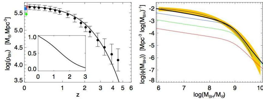
Figure 7.4 Left panel : the black hole mass density of quasars from the data (circles) and the best fit luminosity function (solid line). The inset shows the fraction of the mass density relative to today's value, \rho_{\text{BH}}(z)/\rho_{\text{BH}}(0) , on a linear scale. Right : the black hole mass function at z = 0 (thick black line) and z = 1, 2, 3 (from top to bottom). The shaded region shows the 1\sigma observational uncertainty. Figure credit: Hopkins, P. F., Richards, G. T., & Hernquist, L., Astrophys. J. 654 , 731 (2007). Reproduced with permission of the American Astronomical Society.
