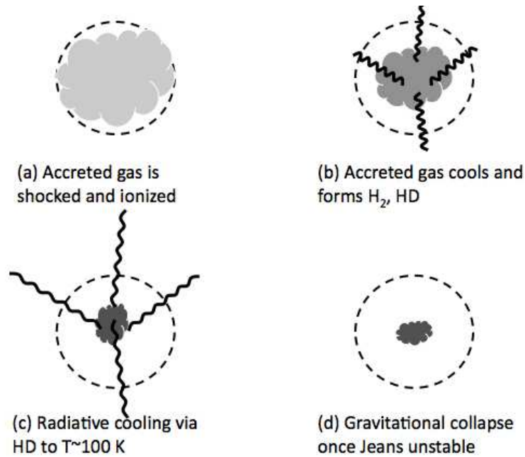
Figure 5.10 Basic stages in Population III.2 protostar formation. (a) A dark matter halo passes the threshold to ionize infalling gas. (b) The accreted gas cools rapidly due to H I line cooling. Because it begins highly ionized, a large fraction of H_2 and HD are formed in the process (c) Instead of stalling, HD line cooling continues to function to T \sim 100 K, substantially below the “loitering” temperature for Population III.1 star formation. (d) Finally, runaway collapse begins once the dense clump’s mass exceeds the local Jeans mass. Further fragmentation may then occur due to gravitational instability, turbulence, or chemical processes.
