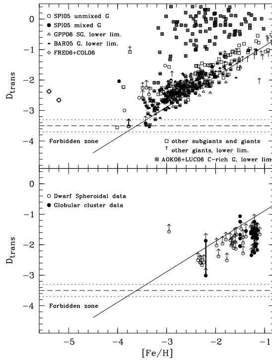
Figure 13.12 Measure of the carbon and oxygen abundance for metal-poor stars, D_{\text{trans}} \equiv \log_{10} \left( 10^{[\text{C}/\text{H}]} + 0.3 \times 10^{[\text{O}/\text{H}]} \right) , as a function of the iron abundance relative to hydrogen, [\text{Fe}/\text{H}] . Top panel: Galactic halo stars. Bottom panel: Stars in dwarf spheroidal galaxies and globular clusters. G and SG indicate giants and subgiants. The critical limit marked with a dashed line was predicted theoretically by comparing the cooling rate for carbon and oxygen lines to \text{H}_2 cooling (which controls the formation of massive Population III stars). Without metal line cooling, no low mass stars should be found below this line. The dotted lines define the uncertainty in the theoretical prediction without dust cooling. If dust cooling is added, the dashed line is lowered by \sim 2 orders of magnitude. Interestingly, all data points are well above the theoretical lines for metal and dust cooling so far. Figure credit: Frebel, A., Johnson, J. L., & Bromm, V., Mon. Not. R. Astron. Soc. 380 , L49 (2007). Copyright 2007 by the Royal Astronomical Society.
