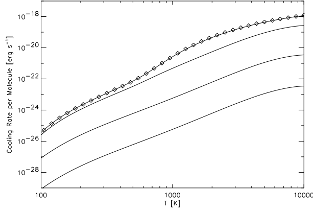
Figure 5.4 Cooling rate from H 2 per molecule. The solid lines show n = 10^{-1} , 10^1 , 10^3 , and 10^5 cm -3 , from bottom to top. The diamonds show the cooling rate in LTE; note how the cooling function approaches this limit when n > n_{\text{cr}} due to the transition to LTE. Figure credit: Bromm V., et al., Astrophys. J. , 564 , 23 (2002). Reproduced with permission of the American Astronomical Society.
