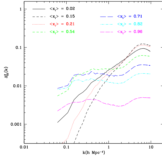
Figure 12.16 Dimensionless power spectra \Delta_{21}^2(k) of spin-flip background during the reionization era in a numerical simulation with radiative transfer; to obtain the 21-cm signal one needs to multiply \Delta_{21}^2(k) by the mean brightness temperature in a fully neutral medium, \sim [28^2(1+z)/10] mK 2 . The curves show the power spectrum through a sequence of mean ionized fractions; the redshifts at which these points are achieved (not listed) do not significantly affect the signal, except through the mean brightness temperature. Figure credit: Lidz, A. et al., Astrophys. J. , 680 , 982 (2008). Reproduced with permission of the American Astronomical Society.
