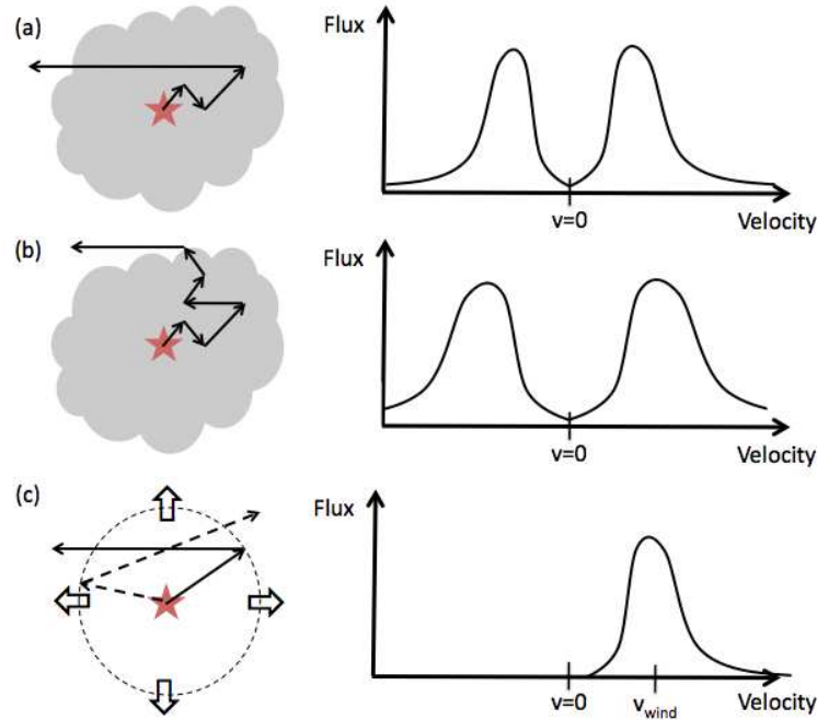
Figure 11.2 Schematic illustrations of the radiative transfer of Lyman- \alpha photons through a dust-free, homogeneous interstellar medium. (a) For a moderately optically thick cloud, a Lyman- \alpha photon undergoes a random walk until its frequency diffuses into the wings of the line, escaping once the optical depth \tau_\nu < 1 at the photon frequency \nu . This produces a double-peaked emission line and spatially compact emission. (b) For a very optically thick cloud, the photon may need to diffuse out of the cloud in space rather than frequency. In that case, the two peaks are substantially broader, and the emission is spatially extended. (c) If the scattering medium has a velocity gradient (here we imagine an expanding shell of gas), photons initially directed toward the observer are scattered away by the blueshifted near side of the shell. However, photons directed toward the far side of the shell that backscatter toward the observer pass through the near side of the shell far out of resonance and escape toward the observer. The result is a single emission line centered on the velocity of the far side of the shell.
