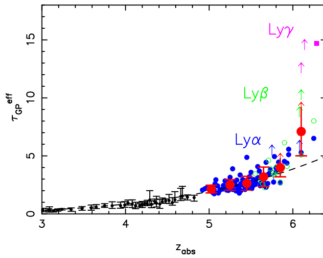
Figure 4.15 Measurements of the effective optical depth in the Lyman- \alpha transition at high redshifts. The small filled circles at z > 5 are direct measurements from the Lyman- \alpha forest, the open circles are measurements from Lyman- \beta absorption translated into Lyman- \alpha , and the filled squares are the same for Lyman- \gamma . The large filled circles with error bars show the average inferred from the Lyman- \alpha and Lyman- \beta measurements. At z > 5.5 , \tau_{\text{eff}} \propto (1+z)^{11} or possibly even steeper. Figure credit: Fan, X. et al., Astron. J. 132 , 117 (2006). Reproduced with permission of the Royal Astronomical Society.
