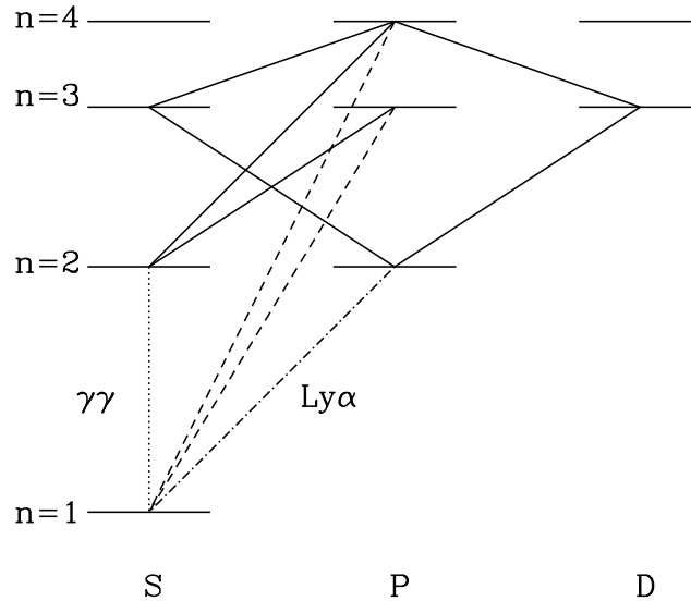
Figure 12.5 Decay chains for Lyman- \beta and Lyman- \gamma excitations. We show Lyman- n transitions by dashed curves, Lyman- \alpha by the dot-dashed curve, cascades by solid curves, and the forbidden 2S \rightarrow 1S transition by the dotted curve. Figure credit: Pritchard, J. R. & Furlanetto, S. R., Mon. Not. R. Astron. Soc. 367 , 1057 (2006). Copyright 2006 by the Royal Astronomical Society.
