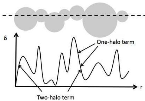
Figure 3.15 Cartoon of the halo model for the cosmic density field. The model splits the dark matter field into gravitationally bound halos (gray circles) with a range of masses. Each of these follows a well-defined density structure, so one can reconstruct the density field purely from the locations of the halos (bottom plot). Correlations amongst the dark matter particles may then be quantified in two steps: the one-halo term describes correlations amongst particles in a single halo, while the two-halo term describes correlations between dark matter particles in separate halos.
