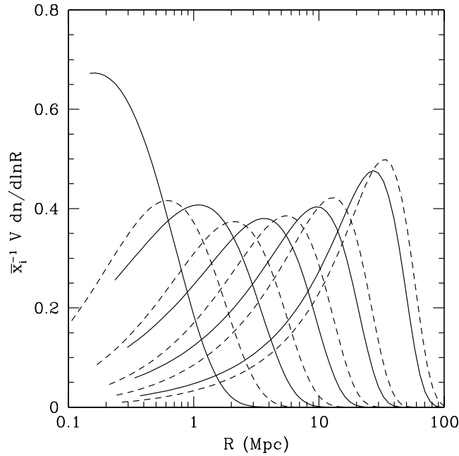
Figure 9.5 H II region size distributions at z = 15 in the analytic model of equation (9.21). The solid and dashed curves assume \zeta \propto m_h^0 and m_h^{2/3} , respectively. From left to right within each set, we take \bar{x}_i = 0.05, 0.2, 0.4, 0.6, and 0.8 . Recombinations are assumed to be uniform throughout the IGM. Figure credit: Furlanetto, S. R., McQuinn, M., & Hernquist, L., Mon. Not. R. Astron. Soc. 365 , 529 (2006). Copyright 2006 by the Royal Astronomical Society.
