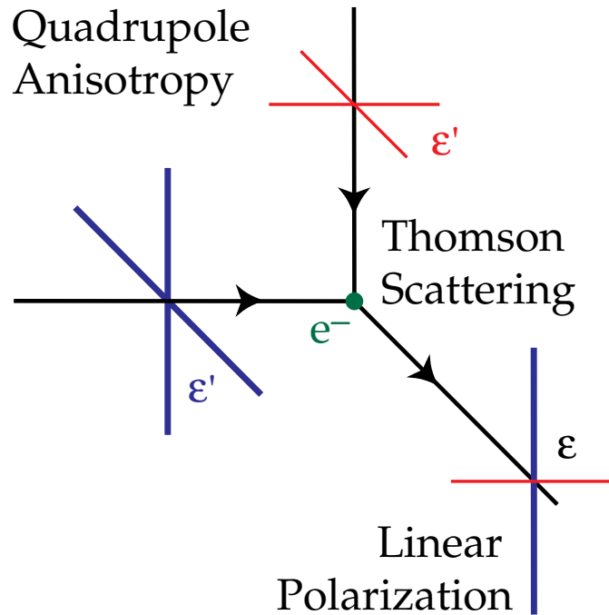
Figure 13.2 Cartoon of the generation of CMB polarization through Thomson scattering. The central electron scatters photons from the CMB. The scattering process only allows photons polarized perpendicular to the plane defined by the lines joining the observer and electron and the photon's source and the electron. For photons from the left of the page, this is the vertical polarization, which corresponds to the thick vertical line at the lower right. For photons from the top of the page, this is the horizontal component (thin vertical line at lower right). If the incident photon field has a quadrupole anisotropy (here, a larger intensity from the left), the resulting scattered field will be polarized. Figure credit: Hu, W. & White, M., New Astron. 2, 323 (1997). Copyright 1997 by Elsevier.
