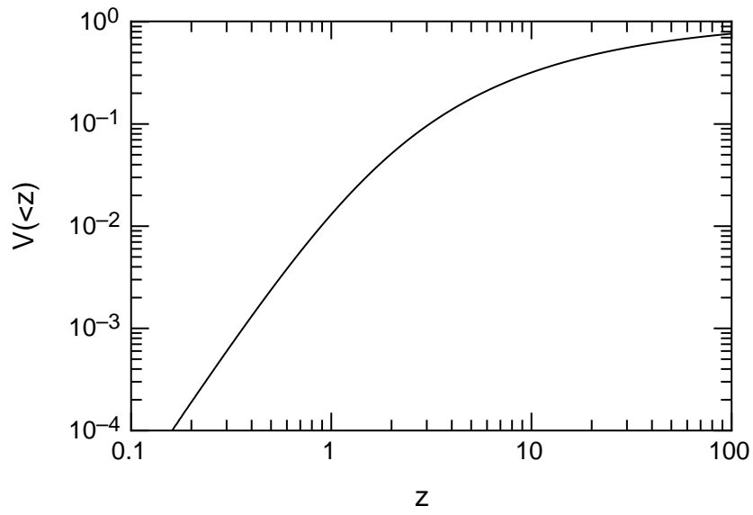
Figure 12.18 The fraction of the total comoving volume of the observable Universe that is available up to a redshift z , as a function of z . Image credit: Loeb, A. & Wyithe, J. S. B., Phys. Rev. Lett. 100 , 161301 (2008). Copyright 2008 by the American Physical Society.
