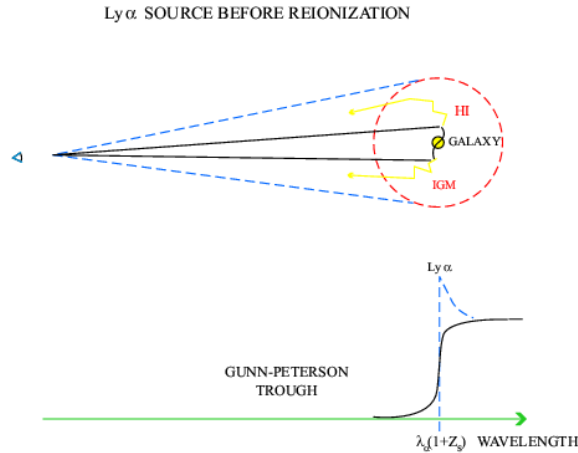
Figure 11.10 Halo of scattered Lyman- \alpha line photons from a galaxy embedded in the neutral IGM prior to reionization (also called a Loeb-Rybicki halo ); see Color Plate 24 for a color version of this figure. The line photons diffuse in frequency due to the Hubble expansion of the surrounding medium and eventually redshift out of resonance and escape to infinity. A distant observer sees a Lyman- \alpha halo surrounding the source, along with a characteristically asymmetric line profile. The observed line should be broadened and redshifted by \sim 1000 \text{ km s}^{-1} relative to other lines (such as \text{H}\alpha ) emitted by the galaxy.
