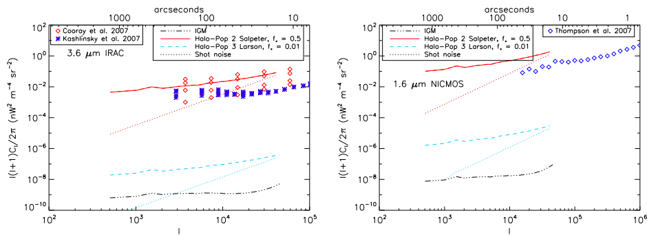
Figure 13.7 Comparison of recent observational data with theoretical predictions (taken from a numerical simulation of reionization) for the angular power spectrum of near-infrared background fluctuations. The two panels also show measurements of angular fluctuations in the 3.6 \mu\text{m} IRAC band and the 1.6 \mu\text{m} NICMOS band (see text). In each one, the double-dot-dashed curve shows predictions for the IGM emission, while the solid and dashed curves show the range of predictions for the total angular power spectra; these two limiting cases take a light, metal-poor population with high f_* and small f_{\text{esc}} (solid) and a heavy, metal-free population with low f_* and high f_{\text{esc}} (dashed curve), both normalized to have the same overall IGM ionization. The dotted curves show the associated shot noise terms. Figure credit: Fernandez, E. R. et al., Astrophys. J. 710 , 1089 (2010). Reproduced with permission of the American Astronomical Society.
