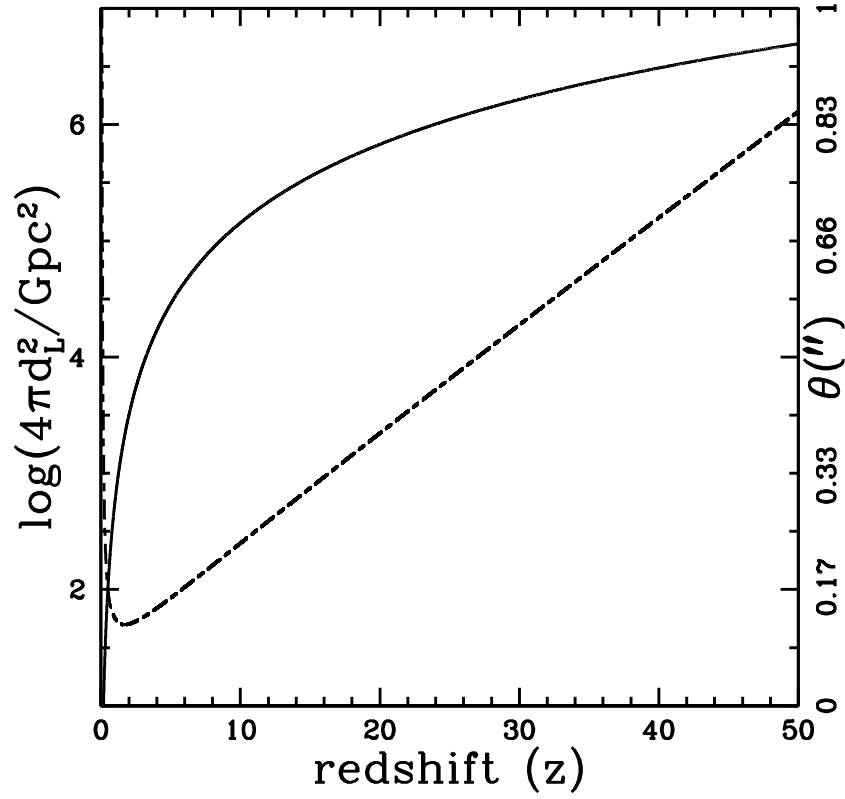
Figure 1.5 The solid line (corresponding to the label on the left-hand side) shows \log_{10} of the conversion factor between the luminosity of a source and its observed flux, 4\pi d_L^2 (in \text{Gpc}^2 ), as a function of redshift, z . The dashed-dotted line (labeled on the right) gives the angle \theta (in arcseconds) occupied by a galaxy of a 1 kpc diameter as a function of redshift.
