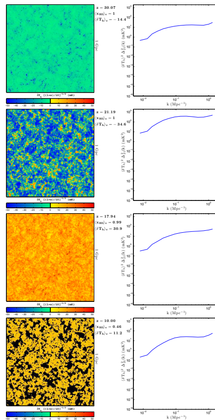
Figure 12.14 Slices through a “semi-numerical” simulation ( left ), and the corresponding spherically-averaged power spectra ( right ), for a model of the spin-flip background at z = 30.1, 21.2, 17.9, 10.0 ( top to bottom ); see Color Plate 29 for a color version of this figure. The slices were chosen to highlight various epochs in the cosmic 21-cm signal (from top to bottom): the onset of Lyman- \alpha pumping (here the blue regions show the cold gas around the first galaxies), the onset of X-ray heating (here the blue regions are cold gas, while the compact red regions represent hot gas around the first black holes), the completion of X-ray heating (where all the gas is hot), and the mid-point of reionization (where black regions are ionized bubbles). All comoving slices are 1 Gpc on a side and 3.3 Mpc deep. Figure credit: Mesinger, A., Furlanetto, S. R., & Cen, R., Mon. Not. R. Astron. Soc. 411 , 955 (2011). Copyright 2011 by the Royal Astronomical Society.
