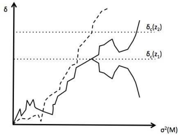
Figure 3.11 Several random walk trajectories for the overdensity as a function of \sigma^2(M) , assuming a sharp k -space filter (or uncorrelated step sizes). The scale is arbitrary here; \delta_c denotes a threshold of interest (i.e., \delta_{\text{crit}} in the Press-Schechter model). Note the wide variation between the trajectories and the rapid variations with scale: a particular trajectory may cross the threshold on multiple scales. In the excursion set model, however, we consider the barrier to be absorbing , so that a trajectory is marked by its first up-crossing. The two solid trajectories have equal probability to occur, which allows us to compute the halo abundance using the “mirror” trick described in the text.
