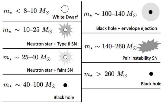
Figure 5.16 Likely fate of Population III stars based on their progenitor mass. Note that the mass ranges are only estimates and depend upon both rotation and mass loss. Many of these supernovae may have unique observational signatures as well, such as gamma-ray bursts. See text for details.
