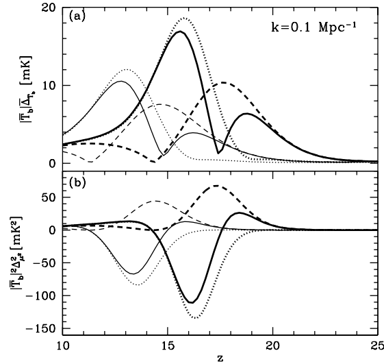
Figure 12.15 Evolution of brightness temperature fluctuations at k = 0.1 \text{ Mpc}^{-1} in two models of the early history of the 21-cm background; this is near the peak sensitivity of most of the planned experiments. The thick curves use parameters similar to our fiducial model in Figure 12.9 (and also the thick curves in Figure 12.8); the thin curves use the Population III model from Figure 12.8. The dashed curve includes the effects of Lyman- \alpha fluctuations only , the dotted curve includes the effects of heating fluctuations only ; the solid curve includes both (but not ionization). Panels (a) and (b) show the spherically averaged rms fluctuation and one of the anisotropic components, respectively. Figure credit: Pritchard, J. R. & Furlanetto, S. R., Mon. Not. R. Astron. Soc. 376 , 1680 (2007). Copyright 2007 by the Royal Astronomical Society.
