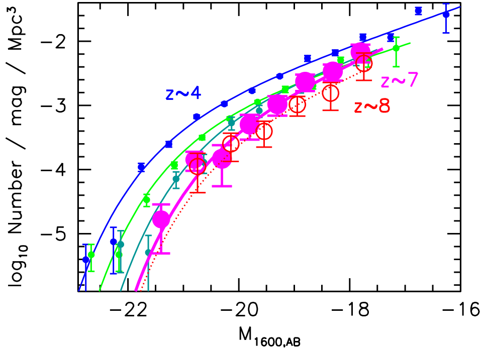
Figure 10.9 Rest-frame ultraviolet luminosity functions derived for galaxies at z \sim 7 (large filled circles) and z \sim 8 (large open circles) compared to lower redshift data (from z = 6 to z = 4 ; the density increases as redshift decreases); see Color Plate 22 for a color version of this image. The vertical axis gives the number of galaxies per comoving \text{Mpc}^3 per AB magnitude at a rest-frame wavelength of 1600 \text{ \AA} , as a function of this magnitude on the horizontal axis. Note the sharp decline in the number density of bright galaxies with redshift and tentative evidence for a steepening faint-end slope. Figure credit: Bouwens, R., et al., Astrophys. J. , 737 , 90 (2011). Reproduced with permission of the American Astronomical Society.
