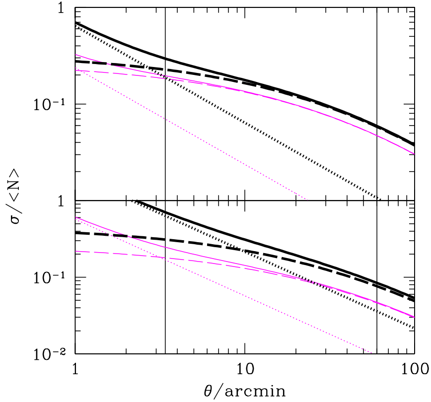
Figure 10.14 The theoretically predicted contributions to the total variance (equation 10.23; solid lines) in Lyman-break galaxy dropout surveys as a sum of cosmic variance (dashed lines) and Poisson shot noise (dotted lines) contributions. The top and bottom panels show results for surveys extending from z = 6-8 and z = 8-10 , respectively. The thin lines assume a luminosity threshold of z_{850,AB}=29 , while the thick ones make a cut at z_{850,AB}=27 , where here z_{850,AB} refers to the AB magnitude in the z_{850} photometric band. Figure credit: Munoz, J., Trac, H., & Loeb, A. Mon. Not. R. Astron. Soc. , 405 , 2001 (2010). Copyright 2010 by the Royal Astronomical Society.
