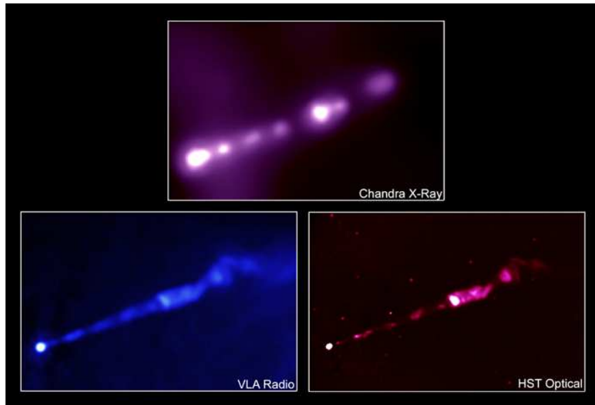
Figure 7.3 Multi-wavelength images of the highly collimated jet emanating from the supermassive black hole at the center of the giant elliptical galaxy M87 (see Color Plate 13 for a color version of this figure). The X-ray image (top) was obtained with the Chandra X-ray satellite, the radio image (bottom left) was obtained with the Very Large Array (VLA), and the optical image (bottom right) was obtained with the Hubble Space Telescope (HST). Figure credit: CXO/NASA.
