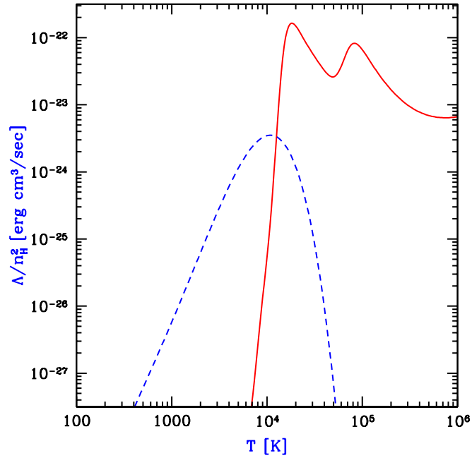
Figure 5.1 Cooling rates as a function of temperature for a primordial gas composed of atomic hydrogen and helium, as well as molecular hydrogen, in the absence of any external radiation. We assume a hydrogen number density n_H = 0.045 \text{ cm}^{-3} , corresponding to the mean density of virialized halos at z = 10 . The plotted quantity \Lambda/n_H^2 , where \Lambda is the volume cooling rate (in \text{erg/sec/cm}^3 ), is roughly independent of density (unless n_H > 10 \text{ cm}^{-3} ). The solid line shows the cooling curve for an atomic gas, with the characteristic peaks due to collisional excitation of hydrogen and helium. The dashed line shows the additional contribution of molecular cooling, assuming a molecular abundance equal to 1% of n_H . Figure credit: Barkana, R. & Loeb, A., Phys. Rep 349, 125 (2001). Copyright 2001 by Elsevier.
