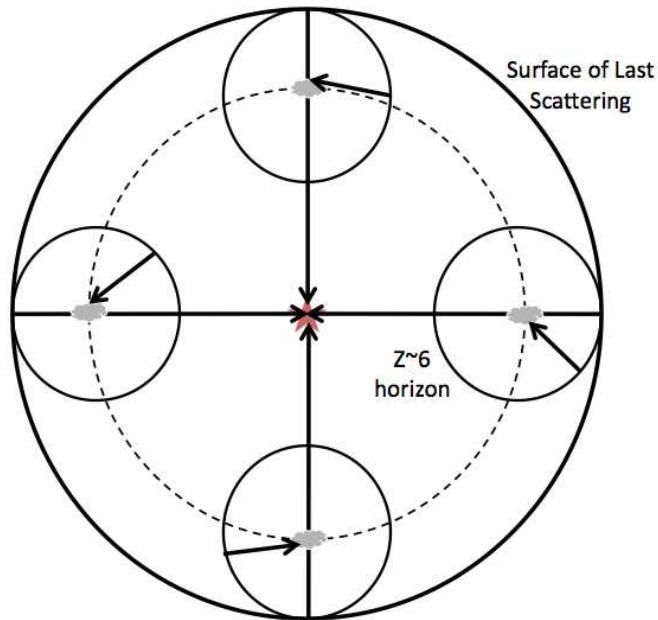
Figure 13.1 Cartoon of the damping of primordial CMB anisotropies after reionization (in comoving coordinates, not to scale). The observer is represented by the star at the center; the thick outer circle represents the surface of last scattering of the observer. CMB photons (arrows) propagate through a screen of parcels of free electrons at z \sim 6 (located at the dashed circle for the observer). Each parcel sees the CMB out to its causal horizon, represented by the smaller circle surrounding it. The low optical depth of free electrons implies that most CMB photons propagate through without interaction (long arrows), but some photons are scattered into the line of sight from other directions. This partially washes out the primordial anisotropies on scales smaller than the horizon at the time of scattering.
