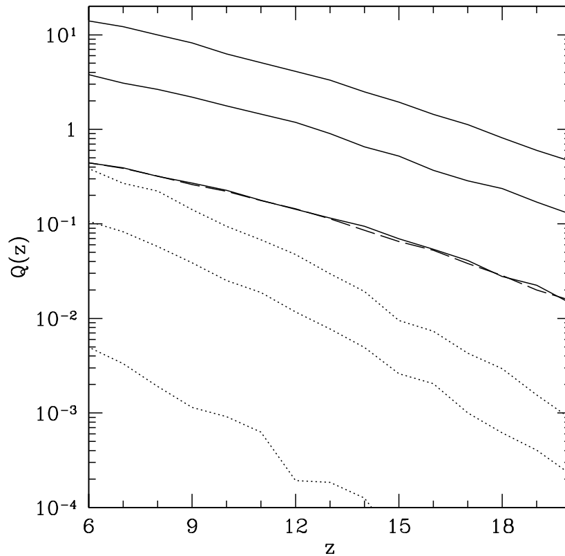
Figure 6.11 Filling factor of wind-enriched regions in different models of star formation and wind expansion, using the same Monte Carlo methods as Figure 6.10. The solid and dotted sets of curves show models with and without efficient star formation in halos below the atomic cooling threshold (in all halos with T_{\text{vir}} > 400 K); otherwise we allow star formation only in halos above the atomic cooling threshold ( T_{\text{vir}} > 10^4 K). Within each set, the curves take f_{\star} = 0.5, 0.1, and 0.01 , from top to bottom. For the \text{H}_2 cooling case, we assume that \omega_{\text{SN}} = 10^{50} \text{ erg } M_{\odot}^{-1} to reflect the powerful supernovae of very massive Population III.1 stars. The dashed curve (nearly coincident with the lowest solid curve) shows the \text{H}_2 case with f_{\star} = 0.1 and \omega_{\text{SN}} = 10^{49} \text{ erg } M_{\odot}^{-1} . Figure credit: Furlanetto, S.R. & Loeb, A., Astrophys. J. 588 , 18 (2003). Reproduced with permission of the American Astronomical Society.
