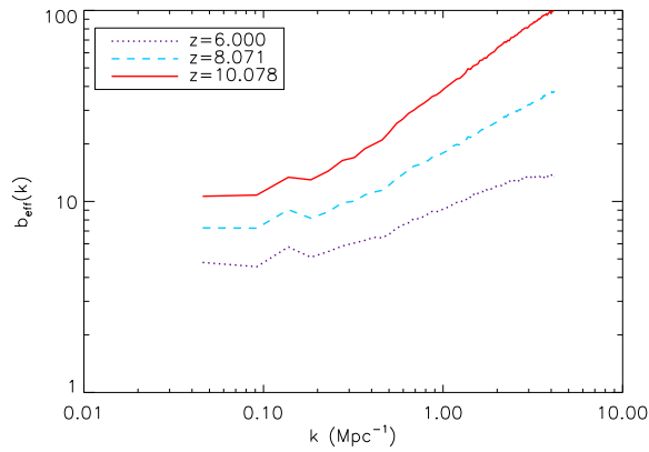
Figure 3.18 Average effective bias for halos with M > 2 \times 10^9 M_{\odot} as a function of spatial scale, estimated by comparing the nonlinear and linear power spectra via b_{\text{eff}}^2(k) = P(k)/P_{\text{lin}}(k) , where the “shot noise” term is already subtracted to obtain the clustering-driven component of the power spectrum P(k) . The three different curves vary the redshift of the bias measurement. Figure credit: Fernandez, E. et al., Astrophys. J. , 710 , 1089 (2010). Reproduced with permission of the American Astronomical Society.
