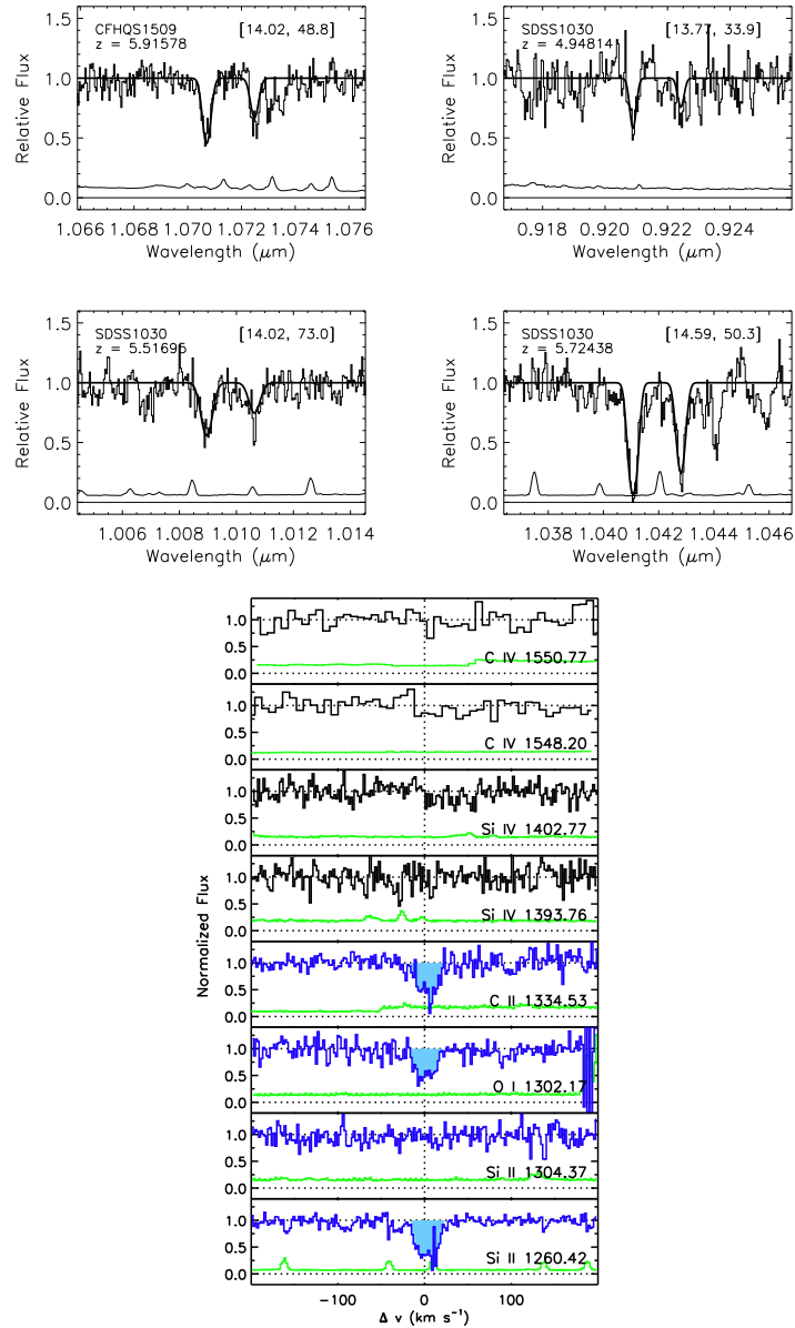
Figure 4.14 Examples of high- z metal absorption systems. Top : Several C IV doublets discovered with the Magellan Baade telescope. The upper histograms show the data; the lower histograms show the errors. The solid curve in each panel is a Voigt profile fit to the two components of the doublet; the column density N_{\text{CIV}} and Doppler width b are listed in brackets in each panel. Bottom : An example low-ionization absorber at z = 5.8765 toward the quasar SDSS J0818+1722 discovered with the Keck telescope. The solid dark lines are the data; the errors are shown as the lower lines in each panel. Shaded regions represent detected transitions. The H I lines are completely saturated in both absorbers. Figure credit: Simcoe, R. A., Astrophys. J. 743 , 21 (2011, top panels); Becker, G. D., Astrophys. J. , submitted (2011), astro-ph/1101.4399 (bottom panels). Reproduced with permission of the American Astronomical Society.
