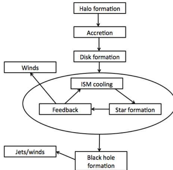
Figure 8.1 Cartoon of the basic steps in galaxy formation, each discussed in this chapter. The process begins with a dark matter halo forming and accreting more matter (either through smooth accretion or mergers). The gas then settles into a rotationally-supported “disk” with an interstellar medium. Within the ISM, self-regulation occurs through cooling and feedback, which ejects some fraction of the halo’s gas through winds. Gas flowing toward the center of the galaxy may accrete onto a central black hole, which would then unbind other ISM gas through winds or jets.
