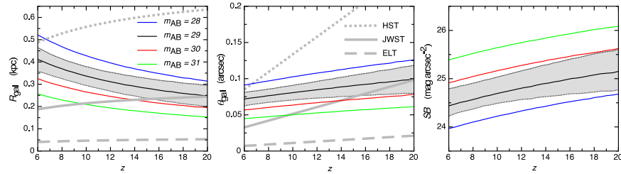
Figure 8.4 Theoretically extrapolated relation between galaxy size and redshift for four values of apparent AB magnitude. The left and central panels show the physical ( R_{\text{gal}} ) and apparent angular sizes ( \theta_{\text{gal}} ), respectively. The thick grey lines indicate the resolution of telescopes with diameters corresponding to HST (2.5 m), JWST (6.5 m) and a ground-based extremely large telescope or ELT (30 m). The right panel shows the average surface brightness within a galaxy scale radius as a function of redshift. In each panel, the grey band around the case of m_{\text{AB}} = 29 mag shows the 68% range of uncertainty on the mean. Figure credit: Wytke, J. S. B., & Loeb, A. Mon. Not. R. Astron. Soc. 413 , L38 (2011). Copyright 2011 by the Royal Astronomical Society.
