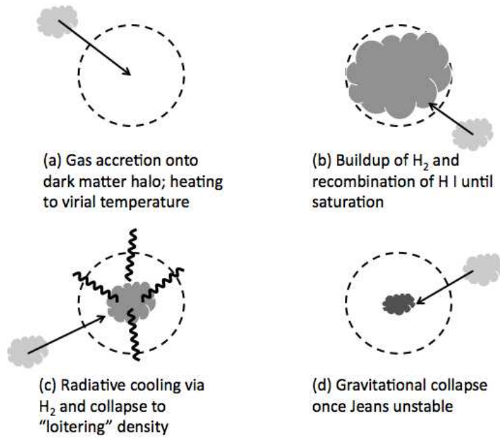
Figure 5.2 Basic stages in Population III.1 protostar formation. (a) A dark matter halo passes the filter mass threshold and begins to accumulate baryons. The virial shock (dashed line) heats the gas to the halo's virial temperature. (b) Inside the warm, dense gas, free electrons catalyze H 2 formation until those electrons disappear thanks to recombinations, when the H 2 fraction saturates. (c) The H 2 fraction remains roughly constant while the gas cloud cools (via the rotational and vibrational transitions of H 2 ) and condenses to higher density until it reaches a critical density and temperature at which gas cooling becomes inefficient. (d) Finally, runaway collapse begins once the dense clump's mass exceeds the local Jeans mass. Further fragmentation may then occur due to gravitational instability, turbulence, or chemical processes.
