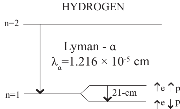
Figure 4.3 Two important transitions of the Hydrogen atom. The 21-cm transition of hydrogen is between the two hyperfine states of the ground energy level (principal quantum number n = 1 ). In the higher energy state, the spin of the electron (e) is aligned with that of the proton (p), and in the lower energy state the two are anti-aligned. A spin flip of the electron results in the emission of a photon with a wavelength of 21-cm (or a frequency of 1420 MHz). The second transition is between the n = 2 and the n = 1 levels, resulting in the emission of a Lyman- \alpha photon of wavelength \lambda_{\alpha} = 1.216 \times 10^{-5} \text{ cm} (or a frequency of 2.468 \times 10^{15} \text{ Hz} ).
