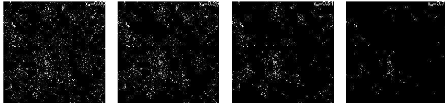
Figure 11.16 Maps of visible LAEs at z = 9 in a semi-numeric simulation, assuming \bar{x}_{\text{HI}} \approx 0, 0.26, 0.51, 0.77 , from left to right. All slices are 250 Mpc on a side and 20 Mpc deep. We assume that all halos with observed luminosities greater than that corresponding to an unattenuated galaxy with M_h > 1.67 \times 10^{10} M_\odot are visible and that L \propto M_h . Figure credit: Mesinger, A. & Furlanetto, S.R., Mon. Not. R. Astron. Soc. 386 , 1990 (2008). Copyright 2008 by the Royal Astronomical Society.
