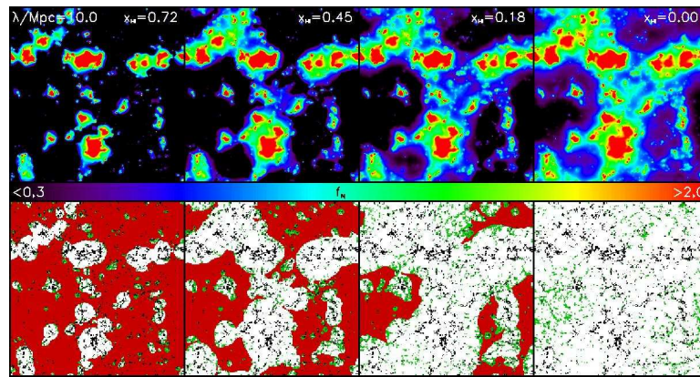
Figure 9.8 IGM absorbers in a “semi-numerical” simulation of reionization (see Color Plate 17 for a color version of this figure). In each panel, we set (by hand) the mean free path of ionizing photons to 10 comoving Mpc; the four columns show different H II fractions at a fixed redshift z = 10 . The upper panels show the ionizing flux (arbitrary normalization) inside ionized zones according to the colorscale. The lower panels show the locations of halos (dark points inside the white regions) and absorbers (green points). Figure credit: Crociani, D. et al., Mon. Not. R. Astron. Soc. , 411 , 289 (2011). Copyright 2011 by the Royal Astronomical Society.
