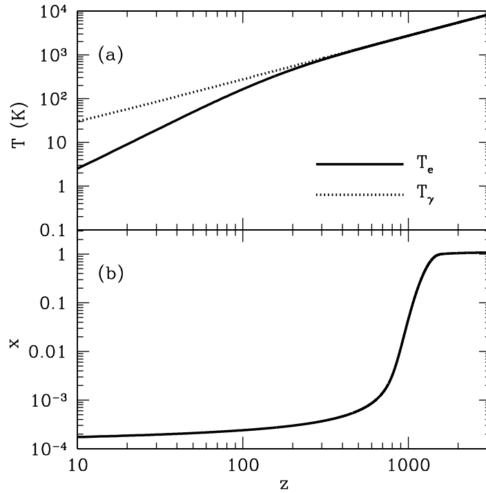
Figure 2.5 Thermal and ionization history of the Universe before the first stars form (panels a and b, respectively). In the top panel, the solid and dotted curves show T_e and T_\gamma , respectively. Note how the ionized fraction x decreases rapidly after recombination at z \sim 1100 and then “freezes-out” at z \sim 300 . Meanwhile, Compton scattering keeps T_e \approx T_\gamma until z \sim 200 , after which the declining CMB energy density and small residual ionized fraction are no longer sufficient to maintain thermal contact between the gas and CMB. At later times, T_e \propto (1+z)^2 as appropriate for an adiabatically expanding non-relativistic gas. These results were produced with the publicly available code RECFAST ( http://www.astro.ubc.ca/people/scott/recfast.html ).
