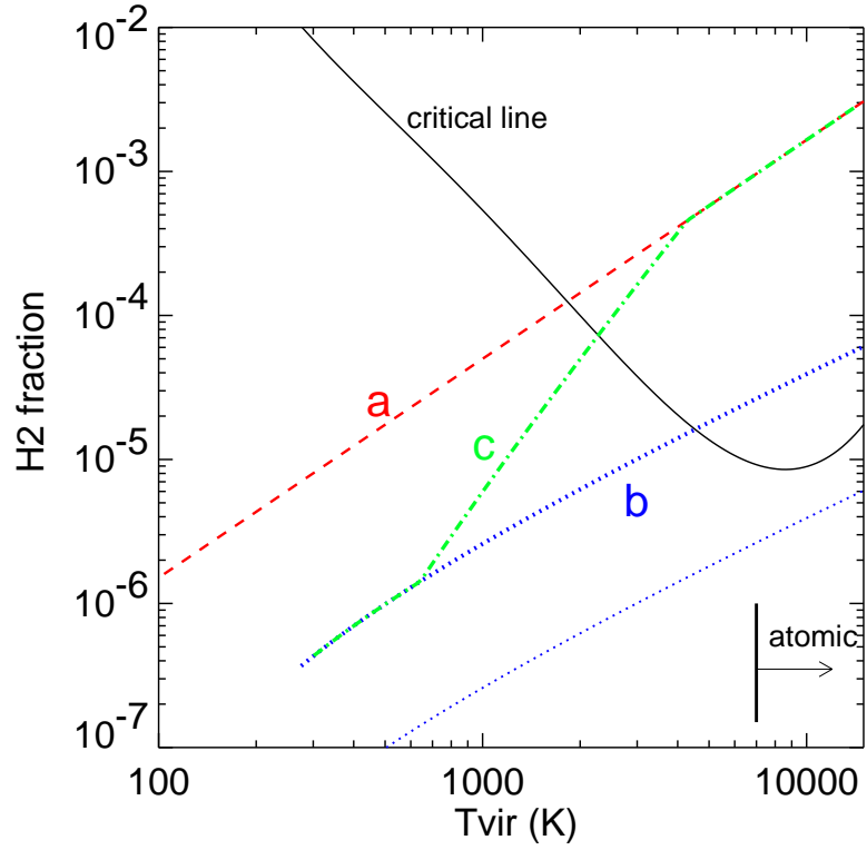
Figure 6.4 Schematic illustration of molecular hydrogen fraction as a function of virial temperature for halos inside a cosmological simulation at z = 17 . The solid line shows f_{\text{H}_2,c} , the critical fraction required for efficient cooling. The dashed line (marked a ) shows f_{\text{H}_2} \sim f_{\text{H}_2,s} in the absence of radiative feedback (see Figure 5.5). The thick (marked b ) and thin dotted lines show f_{\text{H}_2} if self-shielding is neglected and J_{\text{LW},21} = 0.01 or 0.1 , respectively. The dot-dashed line (marked c ) shows the same, but with self-shielding approximately included. Figure credit: Yoshida, N. et al. Astrophys. J. 592 , 645 (2003). Reproduced with permission of the American Astronomical Society.
