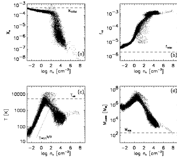
Figure 5.3 Gas properties during dense cloud collapse in a numerical simulation of first star formation. (a) Free electron abundance; note the rapid decline at n_H \sim 10^3 \text{ cm}^{-3} , thanks to efficient recombinations. (b) Molecular fraction f_{\text{H}_2} . The fraction increases rapidly during cloud collapse until the saturation value (eq. 5.10) is reached, when recombinations remove the free electron catalysts. (c) Gas temperature as a function of number density. Note the strong clump at T \sim 500 \text{ K} and n_H \sim n_{\text{cr}} , when radiative cooling becomes inefficient so the evolution stalls. (d) The Jeans mass for this gas; note that M_J \approx 10^3 M_\odot for gas in the aforementioned stalling stage. Figure credit: Bromm, V. et al. Astrophys. J. 564 , 23 (2002). Reproduced with permission of the American Astronomical Society.
