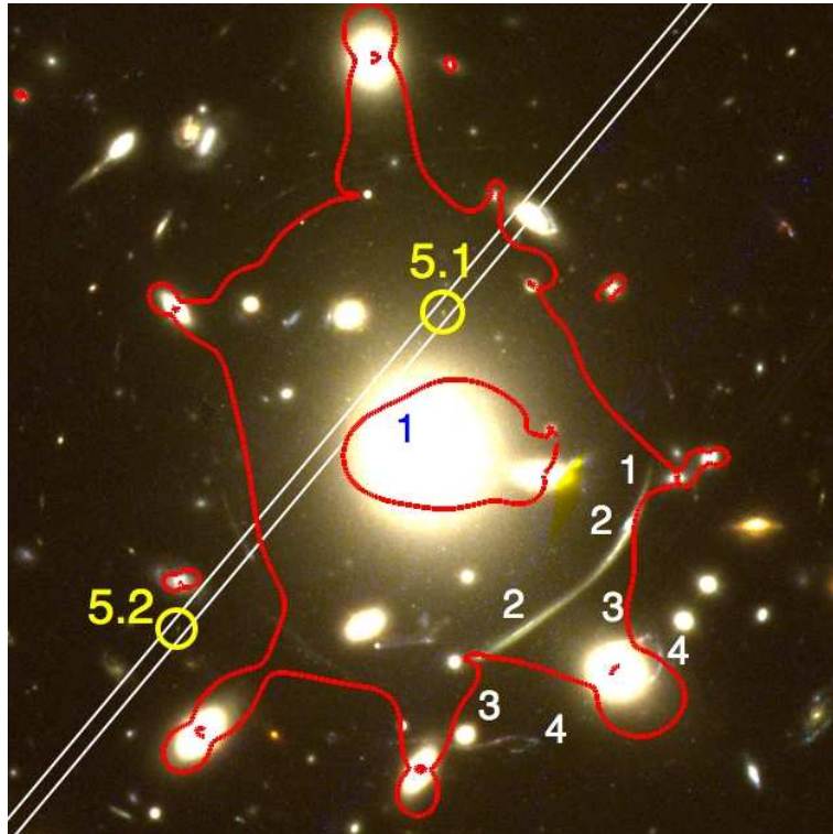
Figure 10.7 Image of the core of the cluster Abell 383, including known multiply-imaged sources (marked 1 to 5) and the non-circular critical lines for sources at z_s = 6 (see Color Plate 21 for a color version of this image). The two images of a galaxy with z_s = 6.027 are marked by circles. The long-slit used for spectroscopic follow-up is shown in white. Figure credit: Richard, J., et al., Mon. Not. R. Astron. Soc. 414 , L31 (2011). Copyright 2011 by the Royal Astronomical Society.
