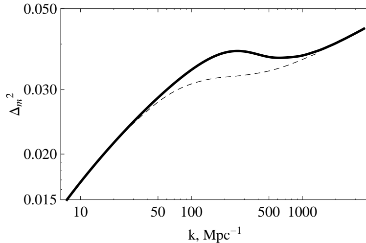
Figure 2.3 The isotropically averaged power spectrum of the matter distribution at z = 40 with and without the relative streaming motions (dashed and solid lines, respectively). Figure credit: Tseliakhovich, D. & Hirata, C., Phys. Rev. D82 , 3520 (2010). Copyright 2010 by the American Physical Society.
