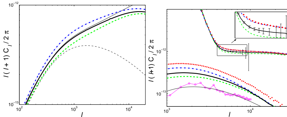
Figure 13.5 Left : Angular power of the Ostriker-Vishniac effect on the CMB. The thick dashed, solid, and dot-dashed curves take models in which reionization ends at z_{\text{reion}} = 8, 12, and 18, respectively. The thin solid curve shows the signal without any baryonic filtering, while the thin dashed curve shows the signal assuming only a linear theory density field. Right : The patchy reionization signal from the same models (lower left, thick curves) and the total CMB anisotropy power spectrum (at upper right, including the primordial, lensing, and Ostriker-Vishniac components as well); note the change in the scale of the vertical axis on this panel. In addition, the dotted curve shows the patchy signal from a model with extended reionization. The open circles show the estimate from a semi-numeric simulation of reionization, with the thin line a corresponding analytic estimate with the same reionization history; the two match very well. The error bars at upper right are representative of current instruments, assuming perfect foreground removal. Figure credit: McQuinn, M. et al., Astrophys. J. 630 , 643 (2005). Reproduced with permission of the American Astronomical Society.
