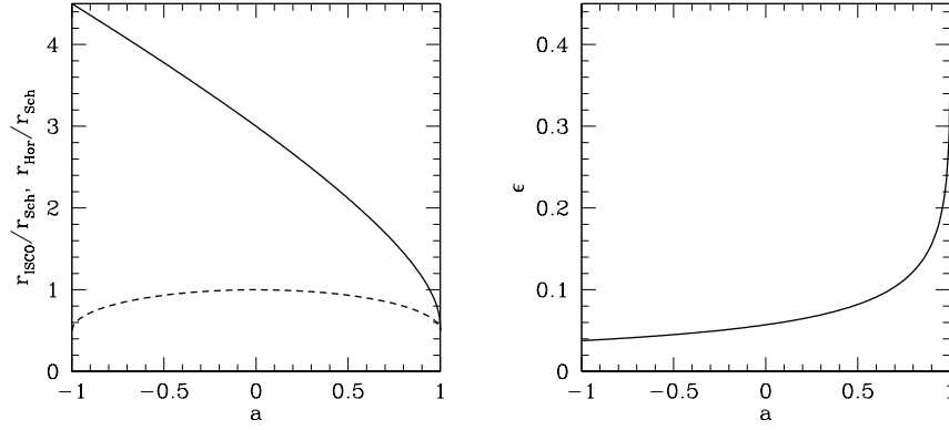
Figure 7.5 The left panel shows the radius of the black hole horizon r_{\text{Hor}} (dashed line) and the Innermost Stable Circular Orbit (ISCO) around it r_{\text{ISCO}} (solid line), in units of the Schwarzschild radius r_{\text{Sch}} (see equation 7.2), as functions of the black hole spin parameter a . The limiting value of a = 1 ( a = -1 ) corresponds to a corotating (counter-rotating) orbit around a maximally-spinning black hole. The binding energy of a test particle at the ISCO determines the radiative efficiency \epsilon of a thin accretion disk around the black hole, shown on the right panel.
