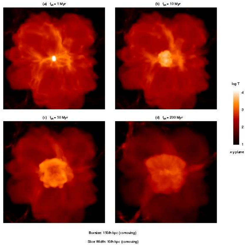
Figure 6.7 Temperature maps from a numerical simulation of a supernova explosion (see Color Plate 9 for a color version of this figure). The supernova of a 200 M_{\odot} star is set off at z \approx 20 in a halo with M = 5 \times 10^5 M_{\odot} and r_{\text{vir}} \approx 100 \text{ pc} . The snapshots are 1, 10, 50, and 200 Myr after the explosion. In the first panel on the top left, the supernova is the central hot region; the star's H II region fills most of the box (fading with time as the gas recombines and cools). The supernova remnant expands over the four panels, gradually becoming more anisotropic as it encompasses the filamentary structure surrounding the halo. Figure credit: Greif, T. et al. Astrophys. J. 670 , 1 (2007). Reproduced with permission of the American Astronomical Society.
