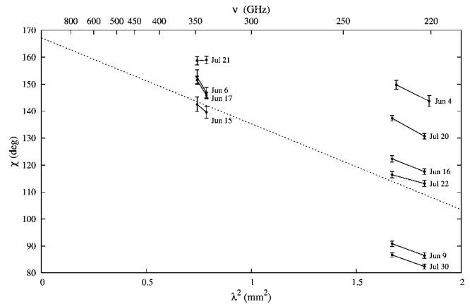
FIG. 1.—Position angles observed in each sideband on each of the 10 epochs. The slope between the two sidebands at each epoch is proportional to the RM, and the extrapolated intercept at the \chi -axis is \chi_0 . The mean RM- \chi_0 fit is also plotted. Variability in \chi_0 is visible in the 230 GHz points (at right), which show slopes similar to the mean but are widely dispersed in \chi .
