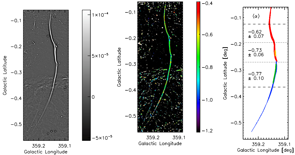
Figure 1. (Left, a ) A filtered image of the total intensity of the Snake at 1.28 GHz with 6.4 arcsec resolution (Yusef-Zadeh et al. 2022a) based on MeerKAT observations (Heywood et al. 2022). The unit in the grey scale bar is Jansky beam -1 . (Middle, b ) The in-band spectral index at 1.28 GHz (20 cm or L band) values along the Snake stretched to values between -1.2 and -0.4 . (Right, c ) Colour traces of different sub-filaments in the Snake. The colours are arbitrarily chosen to distinguish the four sub-filaments. The mean spectral indices within three bright intervals of the Snake are listed (and shown in more detail in Fig. 2). The uncertainties on \langle\alpha\rangle are the standard deviation of \alpha for each segment.
