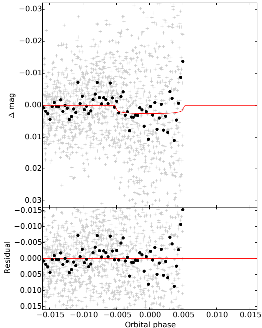
Figure 4. The partial transit event of LTT 1445Ab (top panel) observed by MEarth-South, suggesting that the transit comes from LTT 1445A. The data have been phase-folded using the final transit parameters given in Table 8. The individual data points are indicated in gray; black points indicate the data binned by 2.5 minutes; the red line illustrates the fit to the transit event, computed by taking the mean of the MCMC posterior parameters from Table 8. Error bars on the individual data points have been omitted for clarity, but are large due to the high airmass of the observation. Residuals to the fit are shown in the bottom panel.
