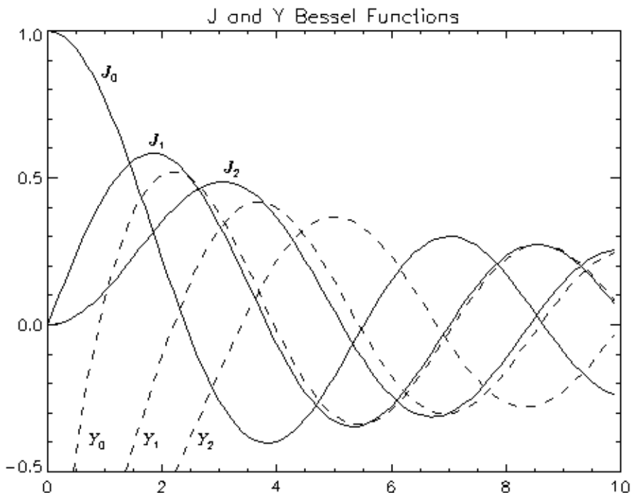
Figure 4-4: The J and Y Bessel Functions.
