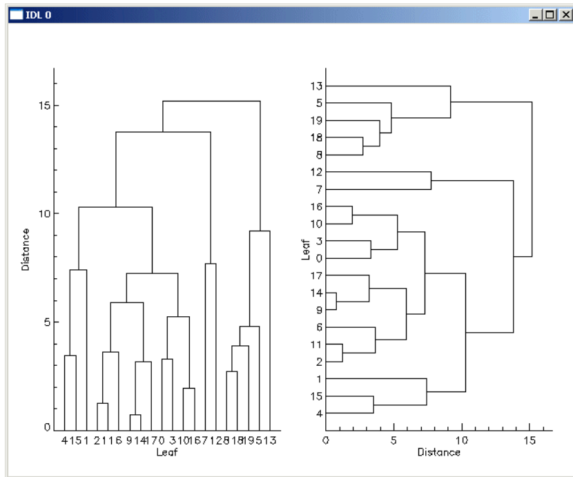
Figure 6-1: Dendroplot
