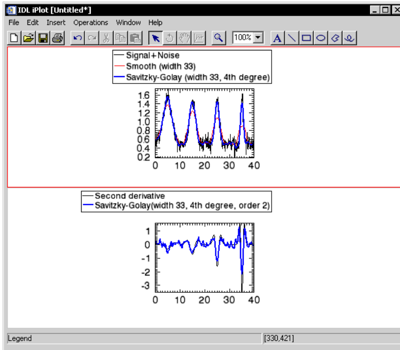
Figure 21-1: SAVGOL Example
