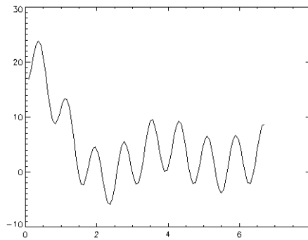
Figure 21-22: Example Plot
