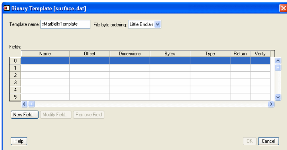
Figure 4-8: Binary Template
