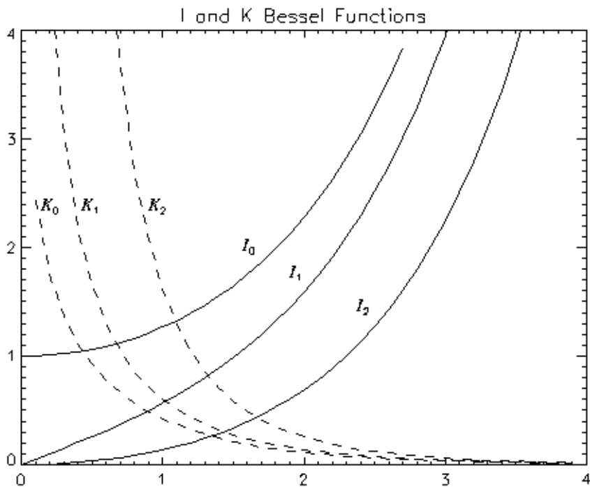
Figure 4-6: I and K Bessel Functions.
