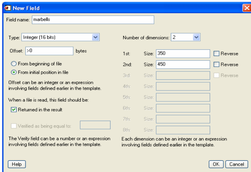
Figure 4-9: Binary Template - New Field
