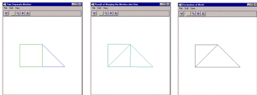
Figure 15-8: Original (left), Merged (center), and Decimated Meshes (right)
