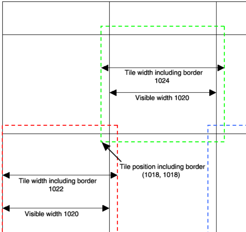
Figure 31-3: Visible Versus Actual Tile Data
