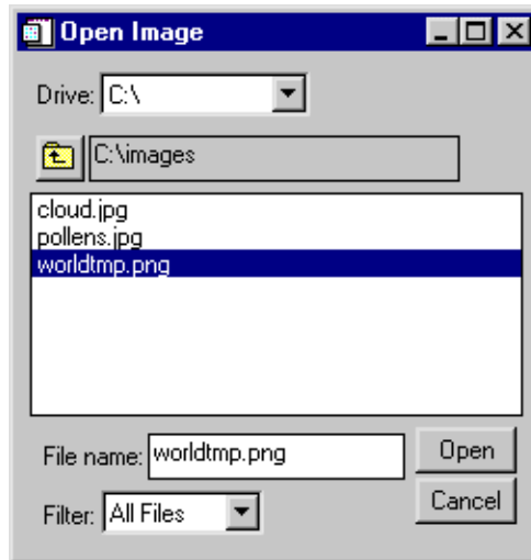
Figure 5-20: CW_FILESEL
