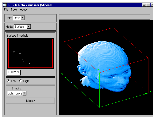
Figure 21-11: Surface Mode
