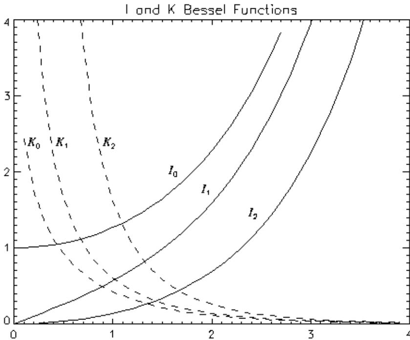
Figure 4-3: I and K Bessel Functions.
