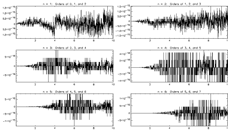
Figure 4-5: Recurrence Relationship for J(x)
