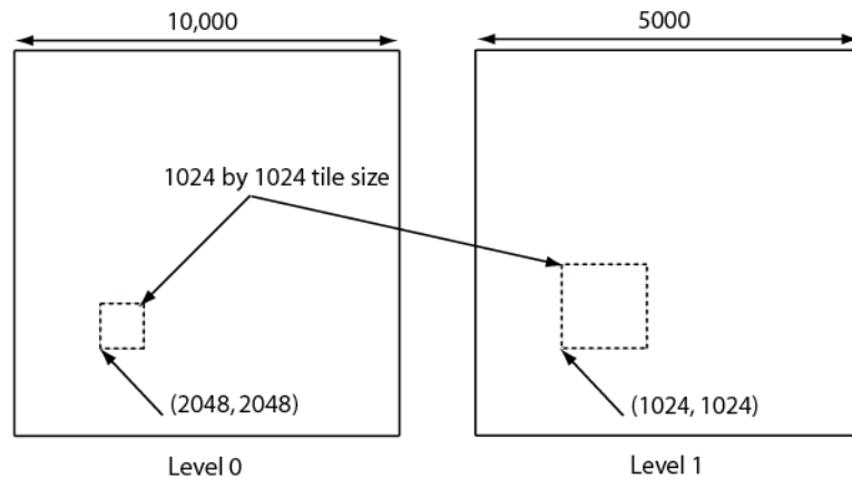
Figure 31-9: Interaction Between Image Level and Zoom with Equal Tile Sizes
