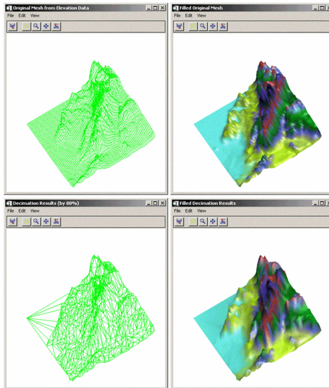
Figure 15-7: Before Decimating (top row) and After Decimating (bottom row)
