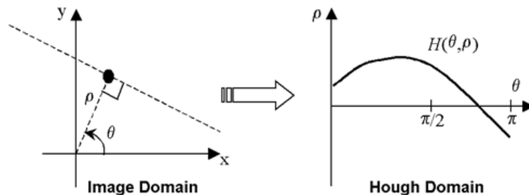
Figure 10-5: Hough Transform
