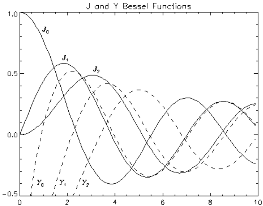
Figure 4-7: The J and Y Bessel Functions.
