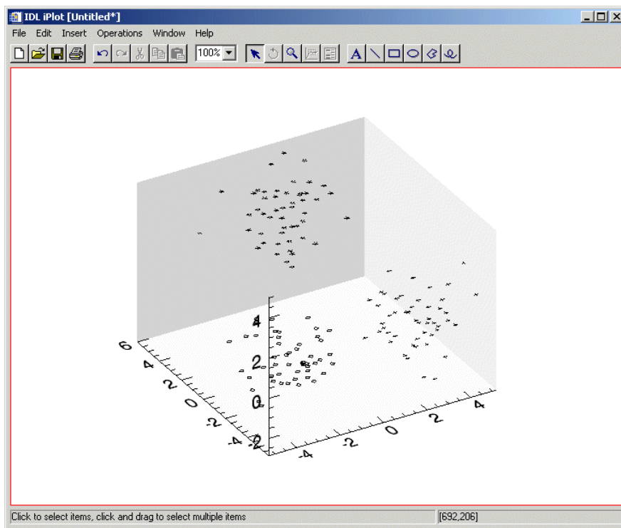
Figure 5-2: CLUSTER Example
