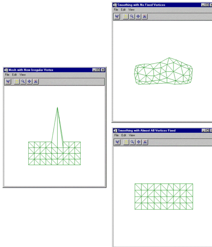
Figure 15-9: The Spiked Mesh (left) and the Two Smoothed Meshes (right)
