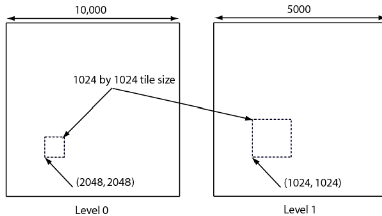
Figure 31-2: Interaction Between Image Level and Zoom with Equal Tile Sizes
