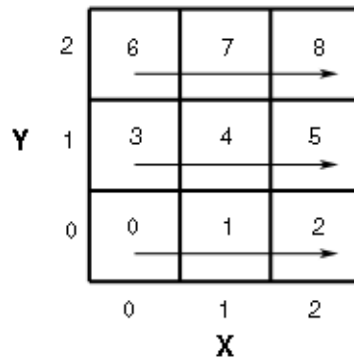
Figure 31-10: Mapping Texture Coordinates
