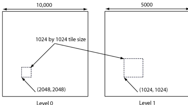
Figure 31-11: Interaction Between Image Level and Zoom with Equal Tile Sizes
