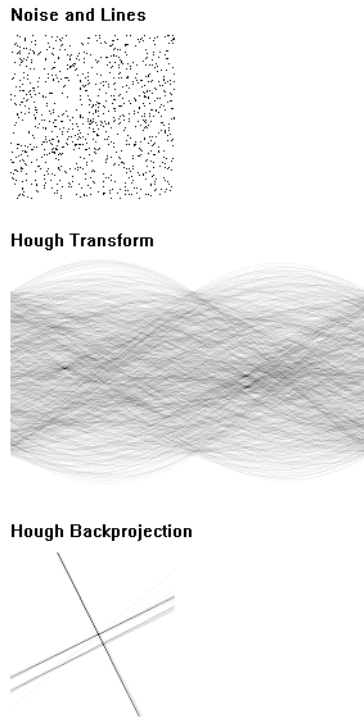
Figure 10-6: HOUGH example showing random pixels (top), Hough transform (center) and Hough backprojection (bottom)
