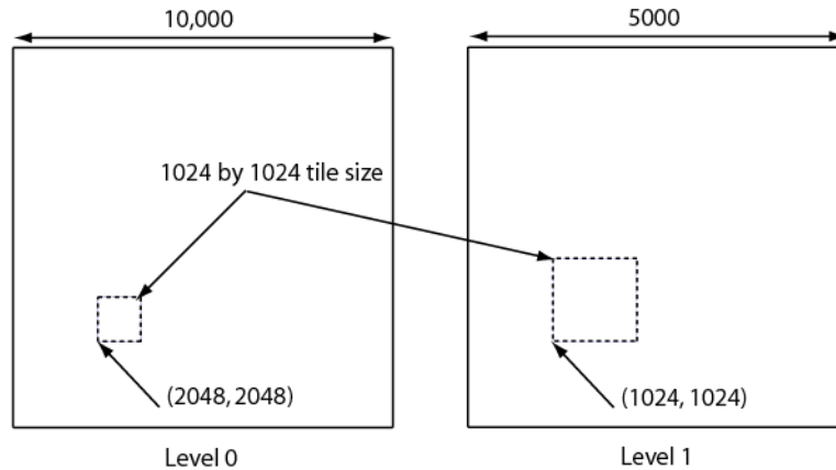
Figure 31-1: Interaction Between Image Level and Zoom with Equal Tile Sizes
