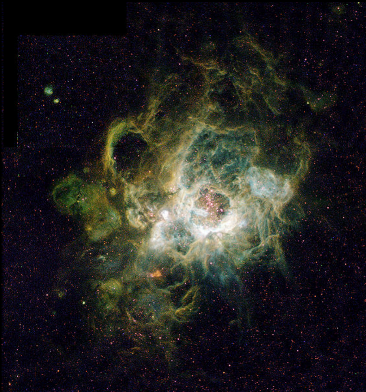
HST view of NGC 604 in M33 (1 Mpc away)
