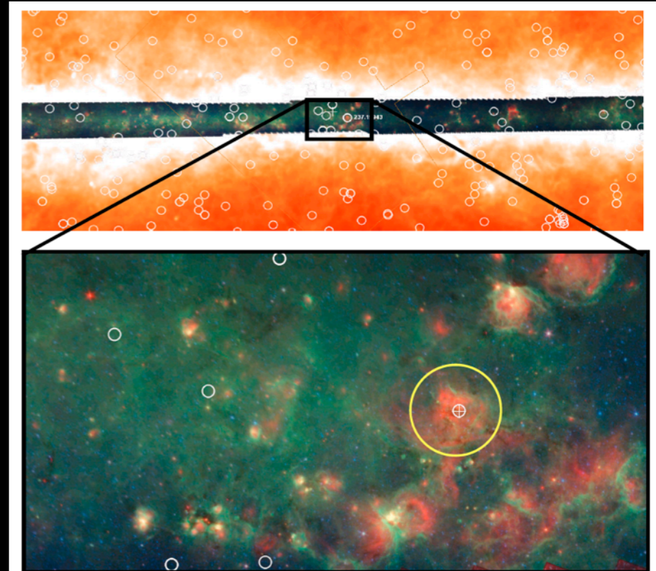
Figure 3.9: Apparent B Star Shell in Glimpse Data The yellow circle surrounds an example of coincidental overlap between B stars and molecular cloud structure separated radial to our line of sight by hundreds of parsecs.
