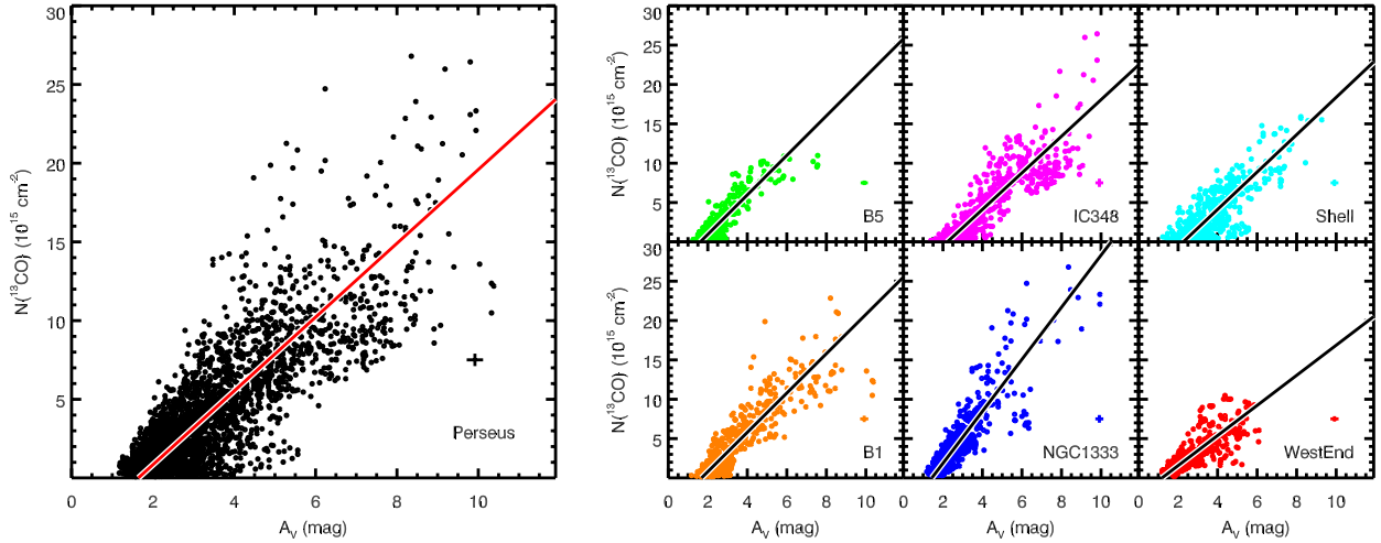
Fig. 8.— The left panel shows ^{13}\text{CO} column density. The median of the 1-sigma errors are shown in bottom right of each plot. The excitation temperature is estimated using the ^{12}\text{CO} peak temperature, assuming this transition to be optically thick. The best fit is shown with a solid line. The right panel show the same as the left panel, but separated into different regions.
