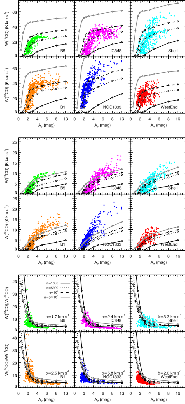
Fig. 11.— Results of the PDR modelling. Upper, middle and bottom panels show the comparison between W(^{12}\text{CO}) , W(^{13}\text{CO}) and the ratio W(^{12}\text{CO})/W(^{13}\text{CO}) with A_V , respectively. Black and grey lines are derived from PDR models.
