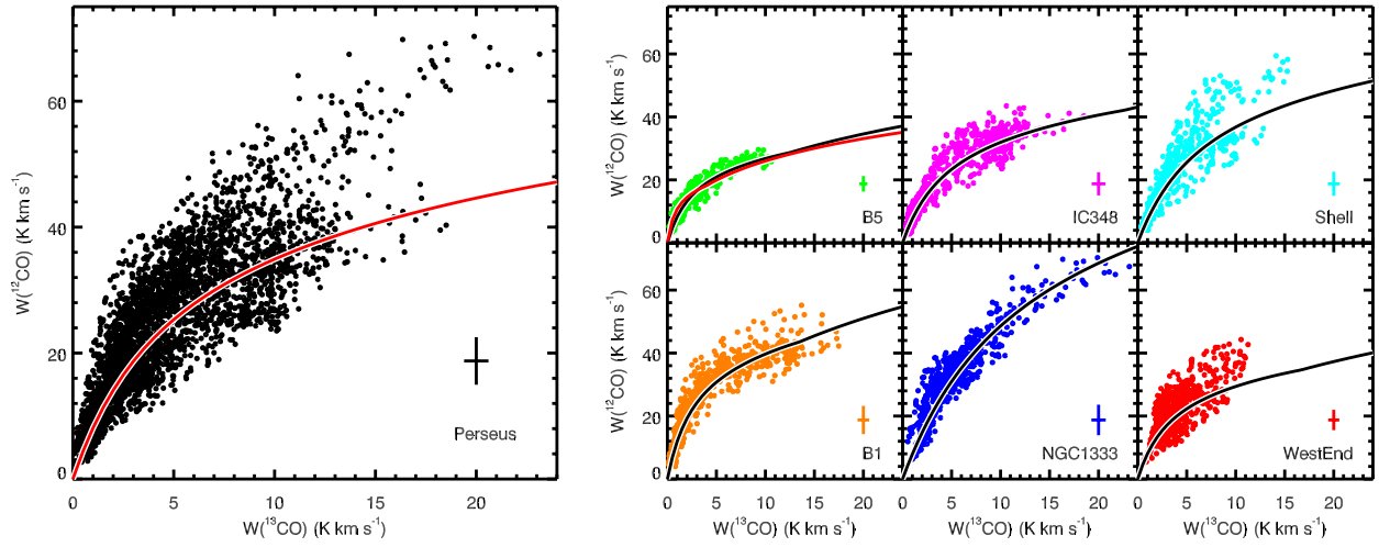
Fig. 5.— Integrated intensity of ^{12}\text{CO} is plotted against the integrated intensity of ^{13}\text{CO} . The left panel shows all data used while right panel shows each region separately, using the same colors as in Figure 3. The median of the 1-sigma errors are shown in bottom right of each plot. Solid lines are the growth curve fit, while the red curve in B5 is the fit from Langer et al. (1989).
