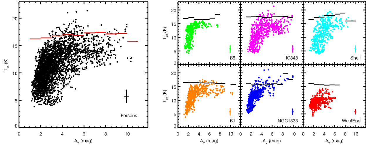
Fig. 10.— Excitation temperature derived using ^{12}\text{CO} plotted against the visual extinction at the same position. The median of the 1-sigma errors are shown in bottom right of each plot. The solid line is the median dust temperature for each sample within the extinction bin. The left panel shows all data used while the right panel shows them separated by regions.
