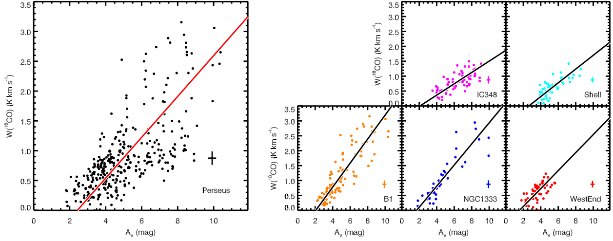
Fig. 9.— Left panel shows \text{C}^{18}\text{O} Integrated intensity compared with the extinction. The median of 1-sigma errors are shown in the bottom right corner of each plot. The best linear fit is shown with a solid line. The right panel show the same that left panel but separated by region.
