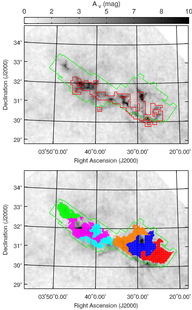
Fig. 3.— ( Top ) The extinction map derived using NICER. The green border is the region observed in ^{12}\text{CO} and ^{13}\text{CO} (1-0) by COMPLETE, while the red border is the region observed in \text{C}^{18}\text{O} (1-0) by Hatchell & van der Tak (2003). ( Bottom ) The re-gridded molecular data that fulfil the requirements detailed in § 3 are shown as boxes. Each of the defined regions are presented in a different color. B5 is green, IC 348 is magenta, the Shell is cyan, B1 is orange, NGC 1333 is blue and Westend is red.
