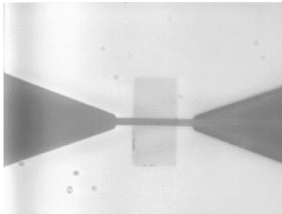
Fig. 1 Photograph of an NbTiN HEB device. The width of the element is 8 μm. The distance between the normal electrodes is about 1 μm. This photo is taken on an optical microscope looking from the back side of the quartz substrate.
