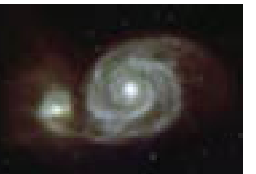
Whirlpool Galaxy
