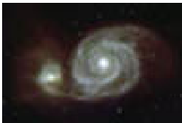
Whirlpool Galaxy
