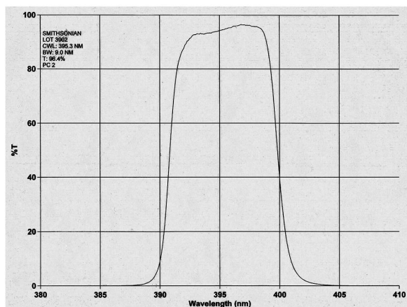
Figure 38: Ca 41 filter transmission.
