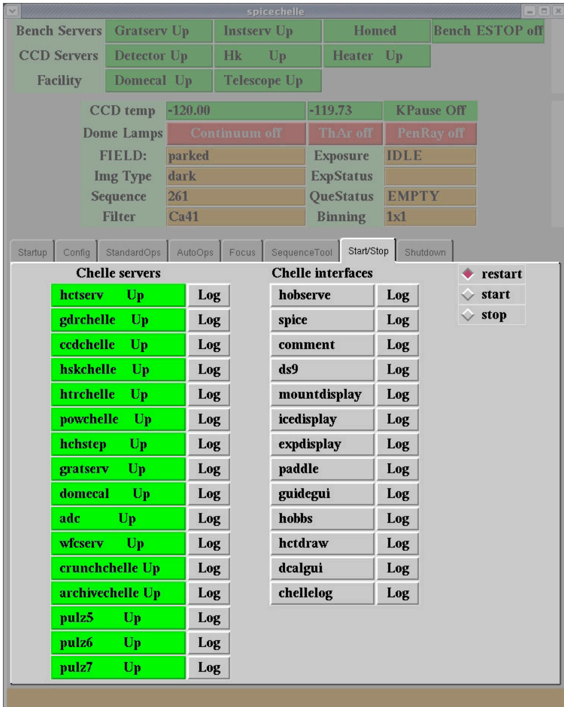
Figure 12: Start/Stop window
