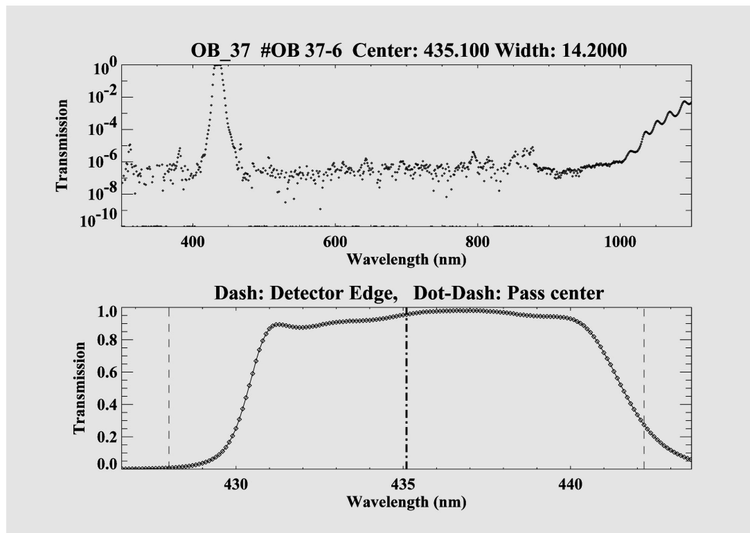
Figure 31: OB 37 filter transmission.
