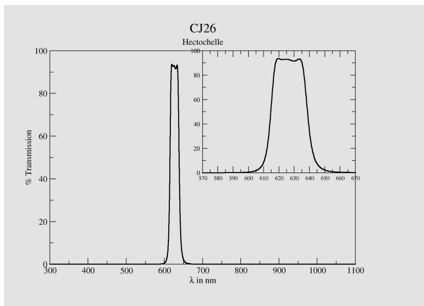
Figure 33: CJ 26 filter transmission.
