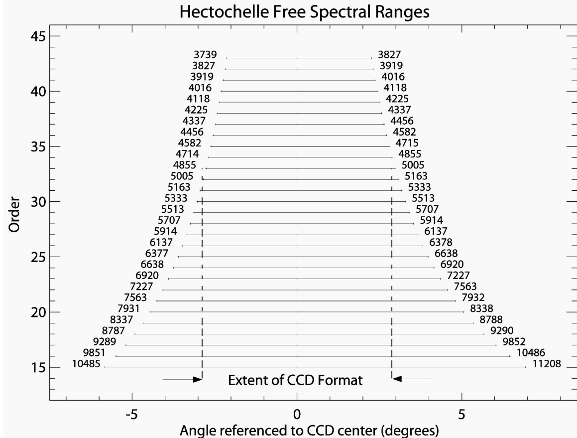
Figure 21: The diffractive orders of the Hectochelle. The dotted line indicates the extent of the CCD format when the grating is operated on blaze. The grating may be rotated, thus moving wavelengths that were lost onto the CCD format.
