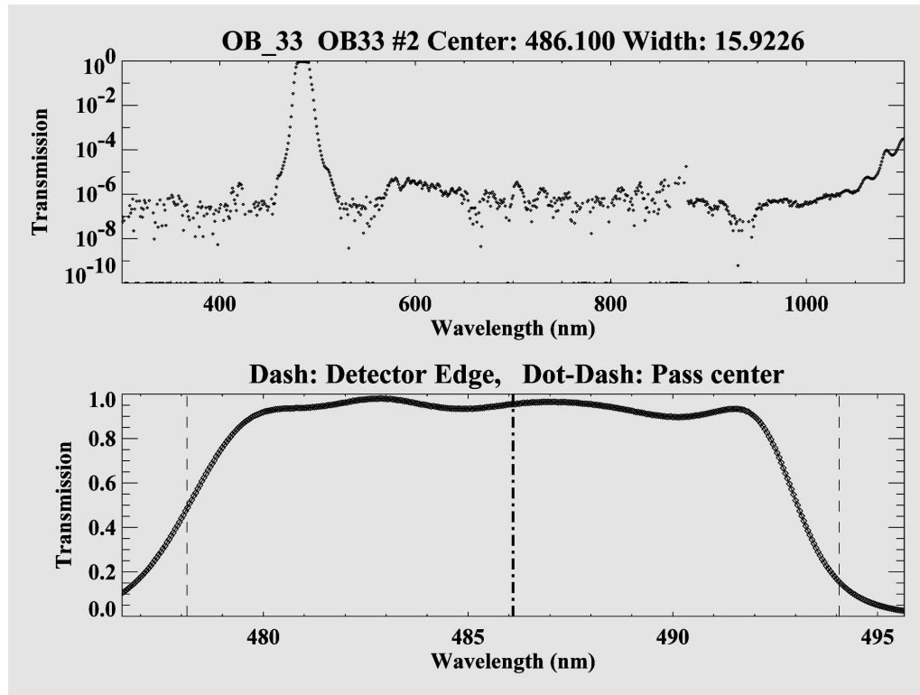
Figure 30: OB33 filter transmission.
