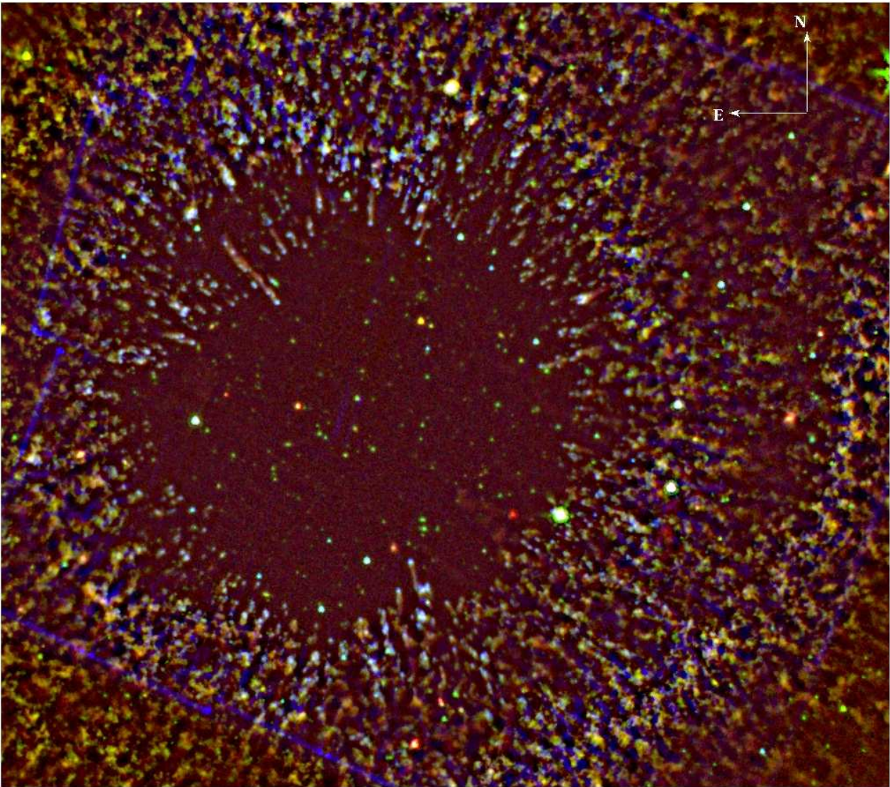
FIG. 17.— Three-color image (the 8 and 4.5 \mu\text{m} IRAC images and the ACS F658N image are mapped to RGB) of the central region of the Helix. This image used the structure-enhanced versions of the images as described in Section 4.1.
