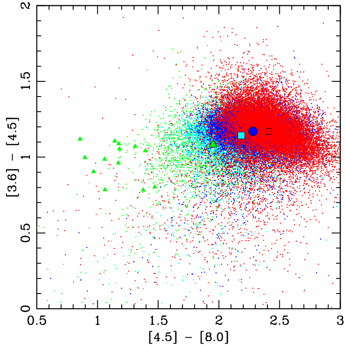
FIG. 5.— Plotted are the IRAC [3.6] - [4.5] vs. [4.5] - [8.0] color of the nebula. The small dots are the binned ( 2'' \times 2'' ) pixels above the minimum flux cutoff. The green dots are those in the inner 200'' , the cyan dots are in the range 220 - 300'' , blue are 320 - 400'' , and red are >400'' from the center of the nebula. Larger green, cyan, blue, and red symbols show the median of the distribution for the radius range. Smaller green filled triangles that appear left of center are the colors of the tips of isolated cometary knots, showing that they are much brighter in the 4.5 \mu\text{m} band than the rest of the nebula.
