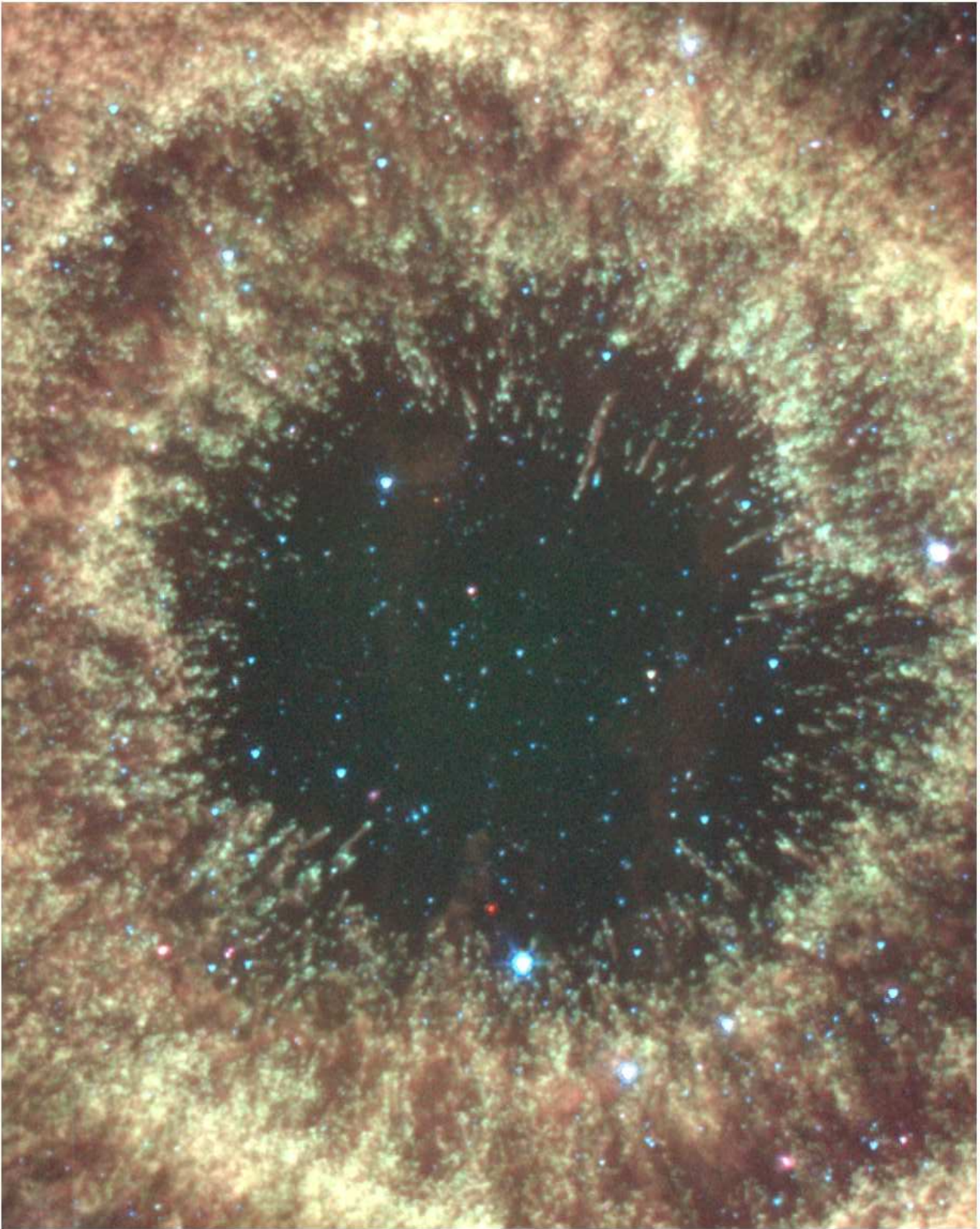
FIG. 2.— Same as in Fig. 1, except showing the 12 \times 11 arcmin region around the central star. This shows the structure of the knots inside the main nebular ring.
