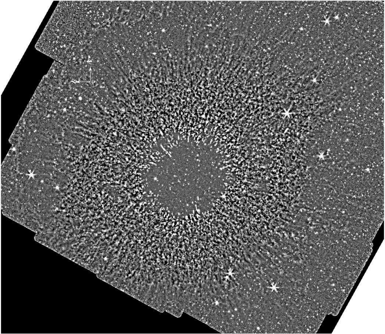
FIG. 12.— IRAC images with the small-scale structure enhanced by taking the ratio of the original image to its local median, as described in Section 4.1. N is at the top, and the field shown is approximately 45 \times 23 arcmin. a) 4.5 \mu\text{m} image.
