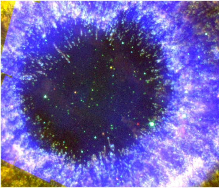
FIG. 7.— A three-color image of the central region of the Helix. The IRAC 8\ \mu\text{m} image is red, 4.5\ \mu\text{m} is green, and the ACS F658N image ( \text{H}\alpha + [\text{N II}] ) is blue. The ACS image was smoothed to match the resolution of the IRAC images. The ACS image does not completely cover the field, which is evident in the corners of this image.
