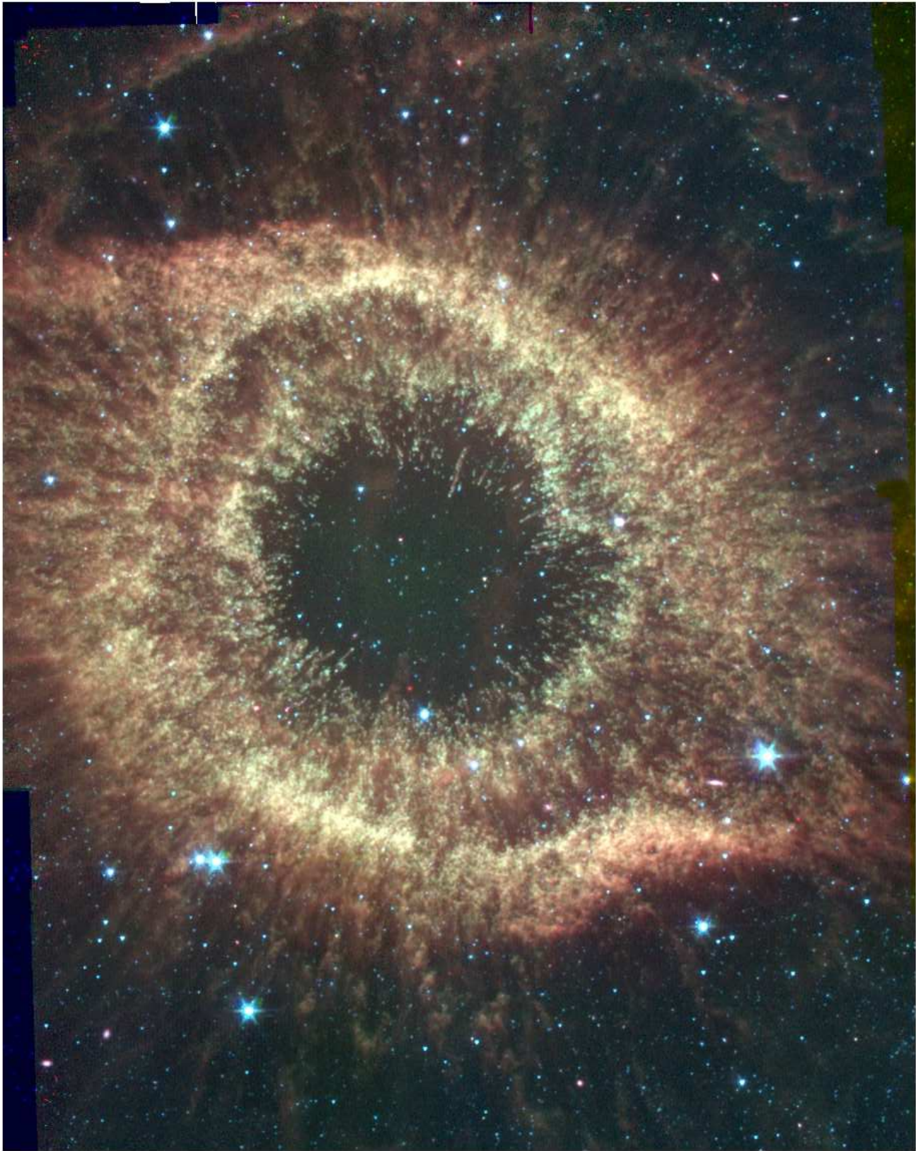
FIG. 1.— Three-color image of the Helix, showing the regions that were imaged in all IRAC bands. The 3.6, 4.5, and 8 \mu\text{m} IRAC bands are mapped to blue, green, and red, respectively. The orientation of the mosaic is in array coordinates, the vertical axis is 59.6 degrees East of North (see Figure 3). The image is approximately 24.2 \times 26.2 arcmin in size.
