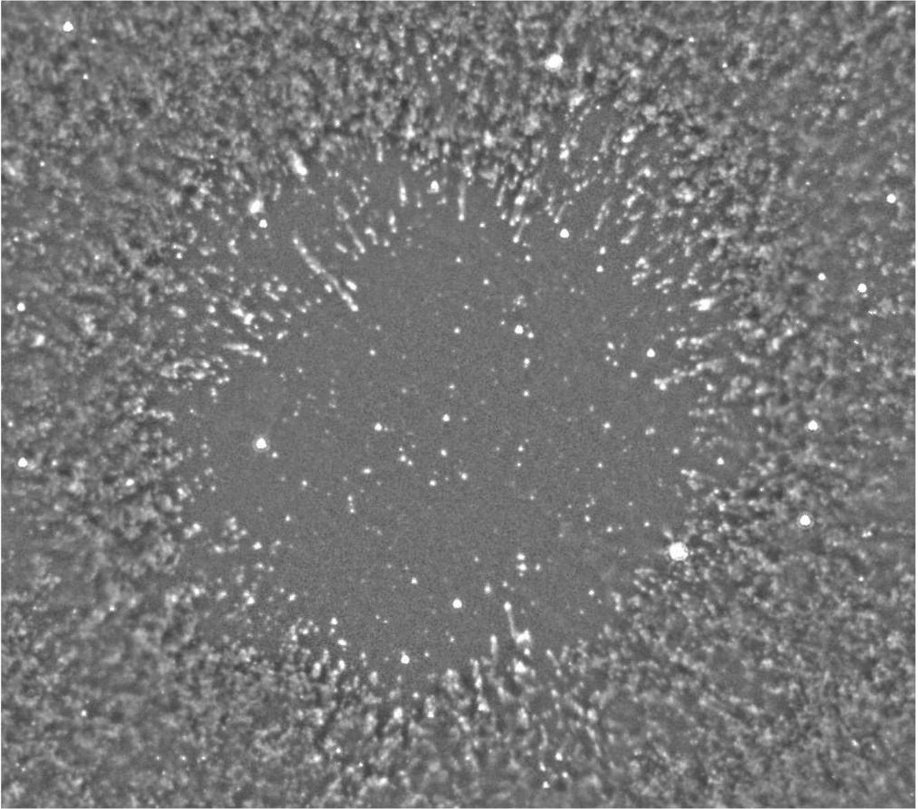
FIG. 14.— Same as Figure 12, but showing the inner 10 \times 9 arcmin region.
