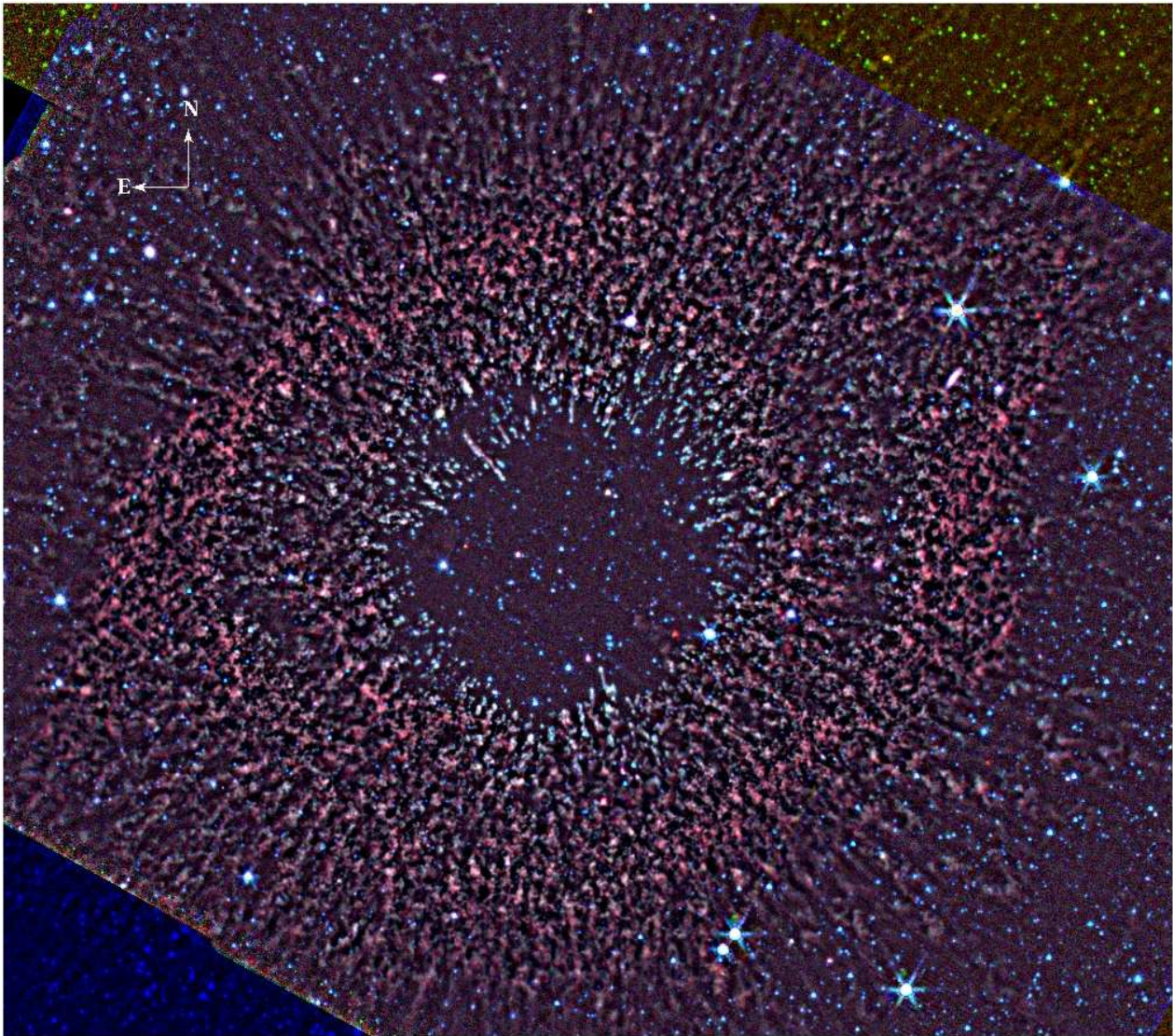
FIG. 16.— IRAC 3 color image (the 8, 4.5, and 3.6 \mu\text{m} images mapped to RGB) using the structure-enhanced images as described in Section 4.1.
