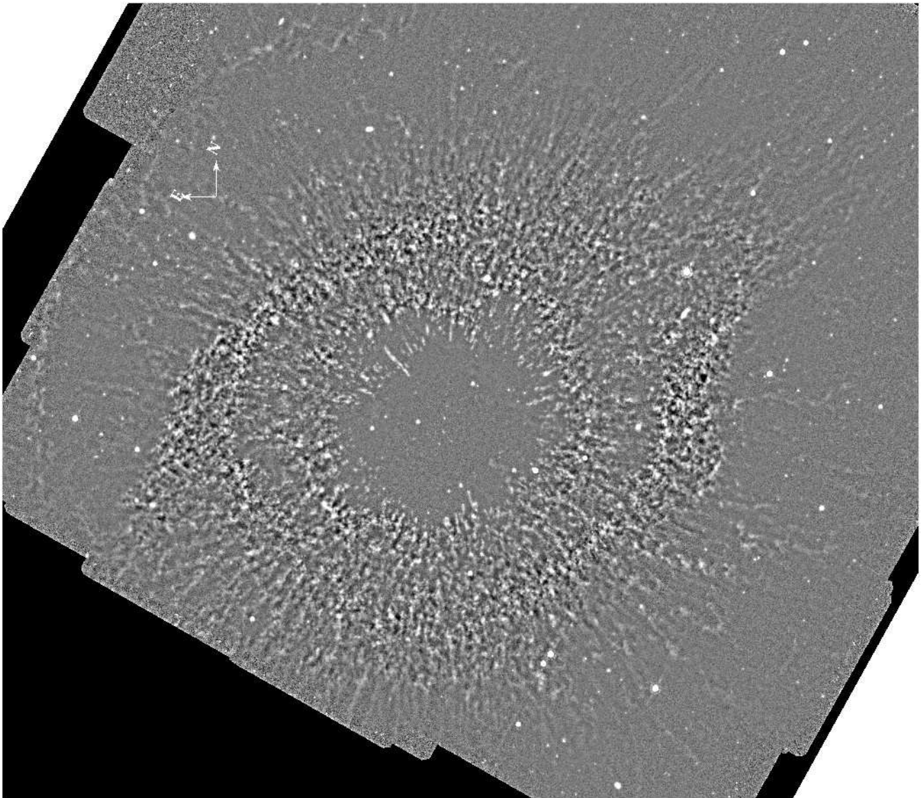
FIG. 13.— same as Figure 12, but the 8 \mu\text{m} image.
