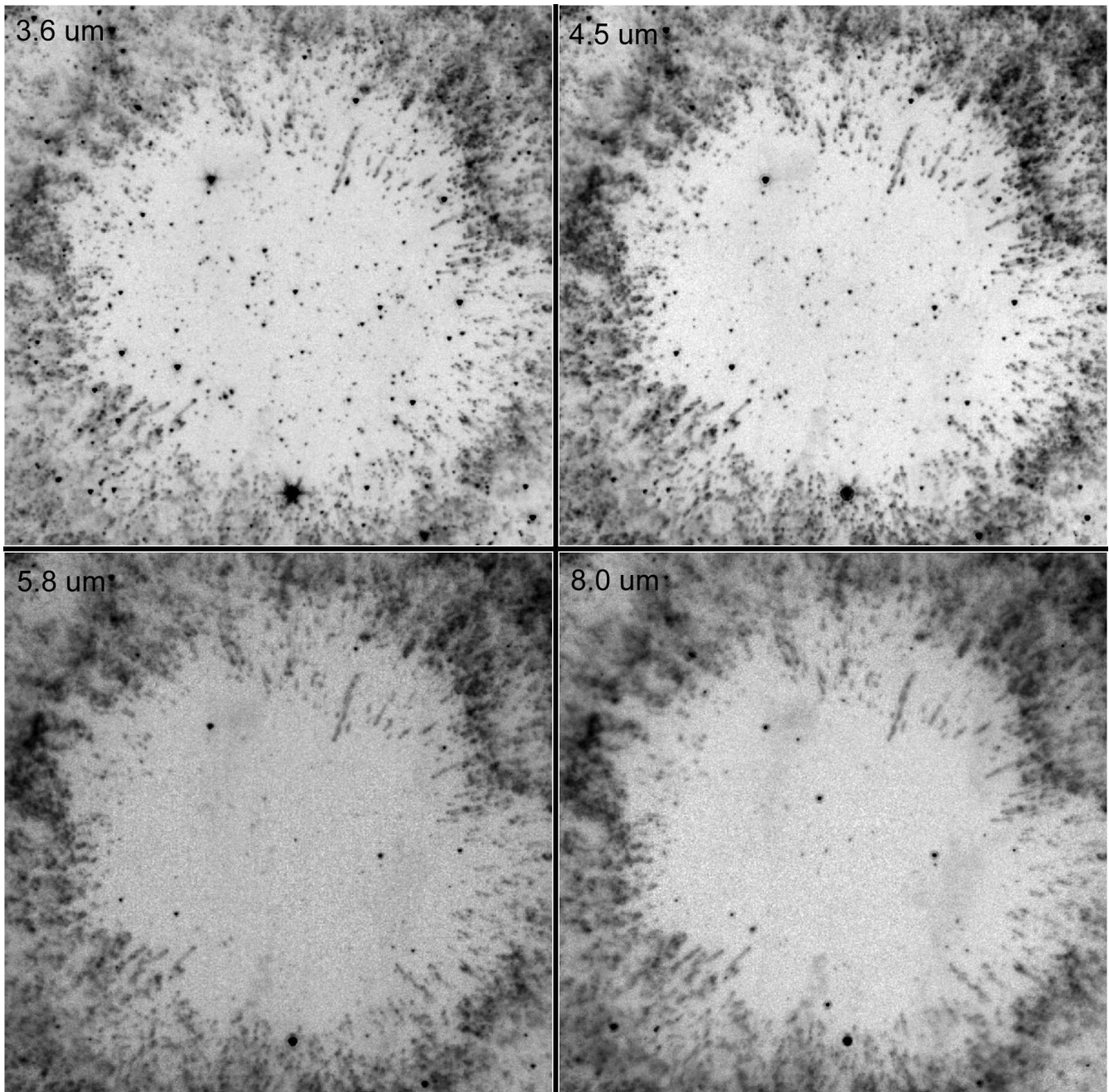
FIG. 4.— Same as Figure 3, except just the inner 6 \times 6 arcmin region displayed.
