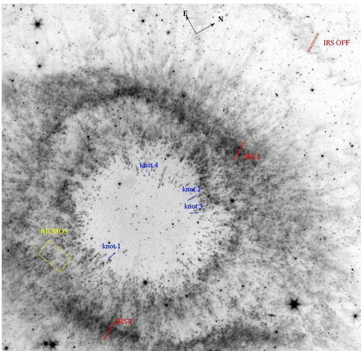
FIG. 10.— Location of the IRS slits and the knots that are discussed in the text, plotted on the IRAC 4.5 \mu\text{m} image.
