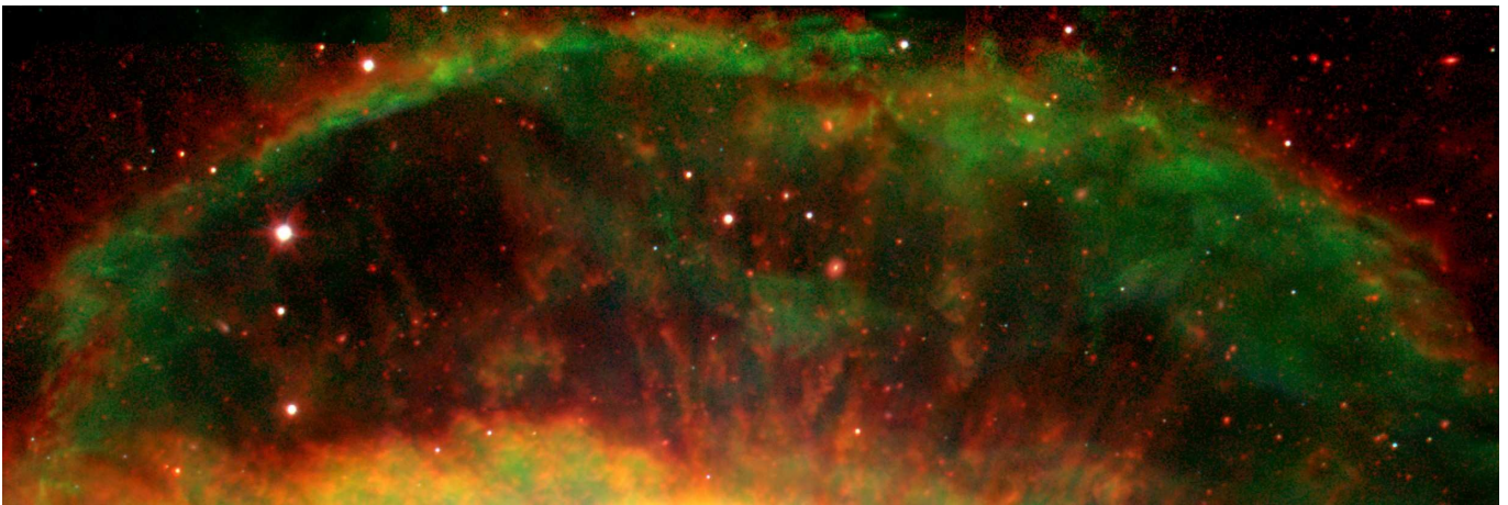
FIG. 19.— Combined Spitzer (4.5 and 8 μm) and HST H \alpha image & [O III] image shown as red-green-blue, respectively (full image available at http://www.spitzer.caltech.edu/Media/releases/ssc2006-01/ssc2006-01b.shtml ). North is 60.9 deg CW from up. The image shows clearly that the H 2 emission is located in a shell just outside of the H \alpha emission.
