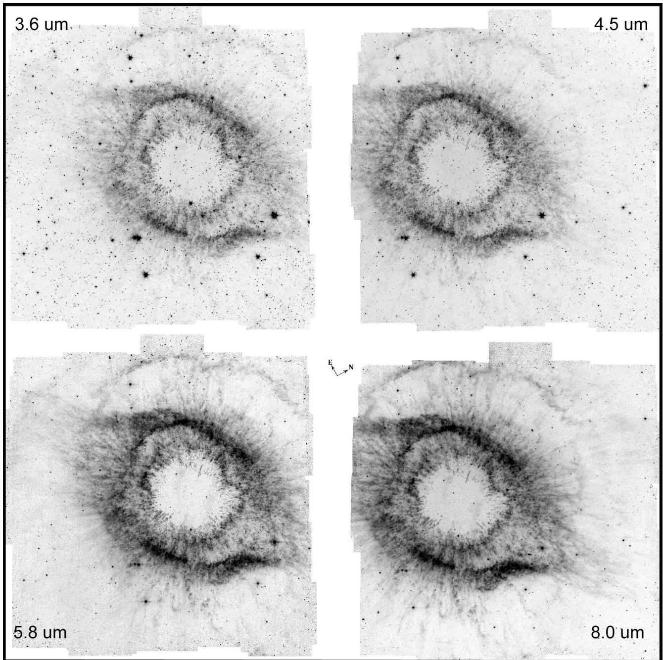
FIG. 3.— Grayscale images of each of the individual IRAC bands. The images are labeled with the name of the IRAC bands, and the orientation indicated by the arrows in the center of the image. The length of the arrows is 1 arcmin. The orientation of all the bands is the same, and each image is aligned vertically and horizontally with its neighbors.
