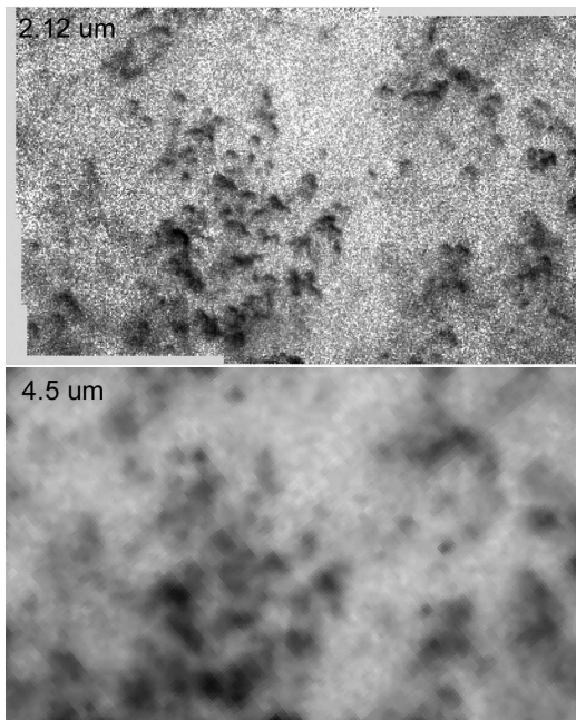
FIG. 6.— Top: The NICMOS 2.12 \mu\text{m} \text{H}_2 image (Meixner et al. (2005), “Position 2”). The total field is approximately 80 \times 50'' , and N is 21.89 \text{ CW} from vertical. Bottom: the same area of the IRAC 4.5 \mu\text{m} image.
