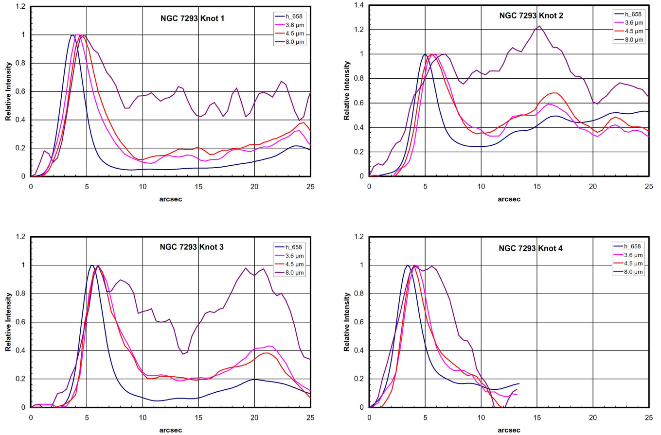
FIG. 18.— Plots showing the profiles of the emission through each of four separate knots. In each plot, the knot profiles from the 0.658, 3.6, 4.5, and 8 μm images are shown. The profile was extracted along a vector aligned in the radial direction, plotted in the inner to outer direction (see Figure 4 and Table 2 for the location of the knots). The width of the extracted region was 2".
