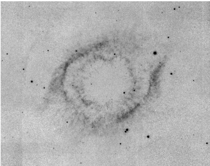
FIG. 8.— Narrowband \text{H}_2 image ( 2.12\ \mu\text{m} ) image of the Helix obtained with QUIST. North is up, and the image is approximately 29 \times 23 arcmin.
