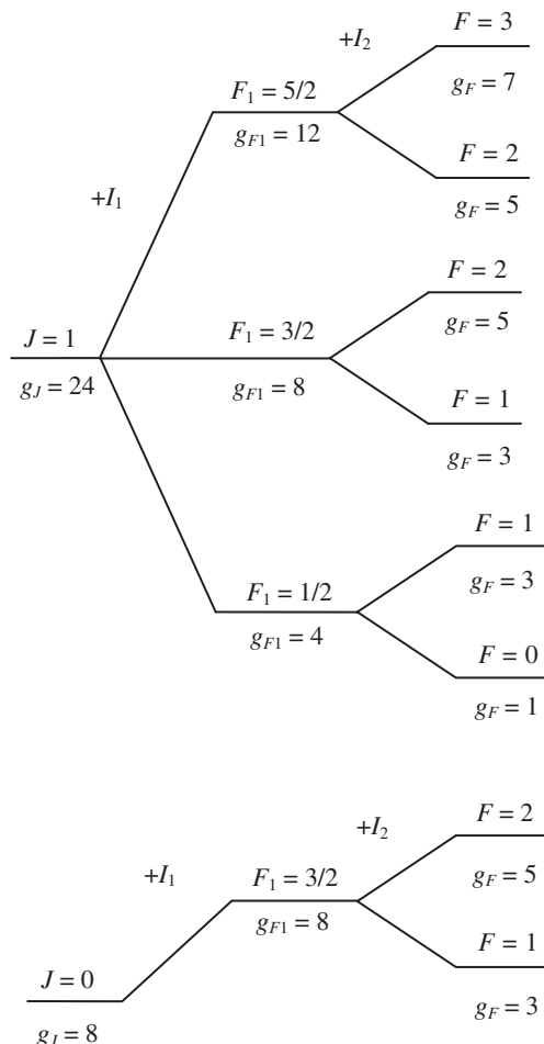
Fig. 1. Schematic example of the multiplets of HBr levels. Note: I(\text{Br}) = I_1 = 3/2 , I(\text{H}) = I_2 = 1/2 , g_i = (2I_i + 1)(2I_j + 1) = 8 , and g_s = 1 for all transitions of HBr.
