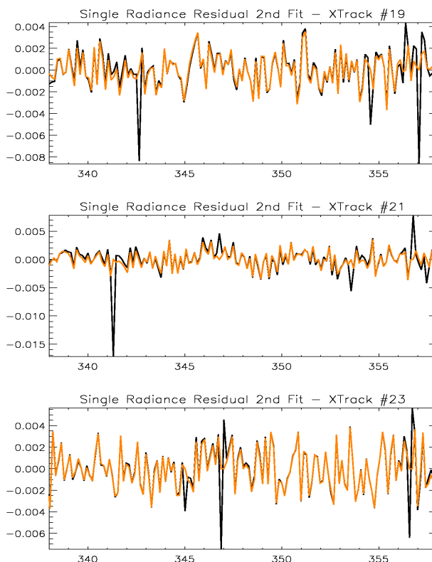
Figure 2: BrO fitting residuals for three selected cross-track positions (19, 21, 23) showing the original residual (black line) and the residual after exclusion of outliers (orange line).
