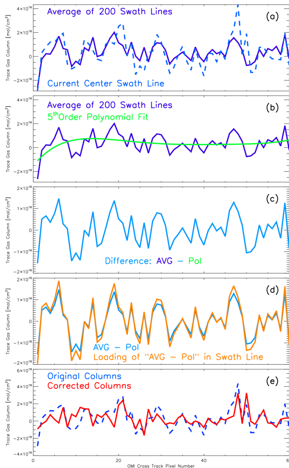
Figure 5: Cross-track smoothing of an individual HCHO swath line. (a) current swath line column values and 200 swath line average (compare Figure 3); (b) polynomial fit; (c) cross-track stripe pattern (difference between average and polynomial); (d) fitted loading of cross-track stripe pattern in current swath line; (e) original and corrected HCHO columns. X-axes in all plots are cross-track position 1 to 60.
