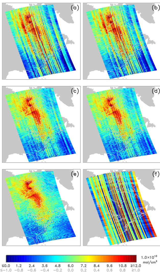
Figure 1: Destriping of BrO columns. (a): individual irradiance measurement, no outlier removal; (b): like "(a)" with outlier removal; (c): solar composite spectrum, no outlier removal; (d): like "(c)" with outlier removal; (e): post-processing destriping of "(d)"; (f): correction factor "(d) -> (e)". Black numbers on legend are for panels (a) to (e), gray numbers for the correction factor (f).
