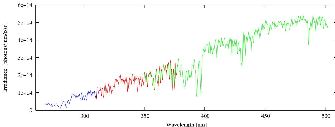
Figure 3: Example of an OMI composite solar spectrum for UV-1 (blue), UV-2 (red), and VIS (green) channels.
