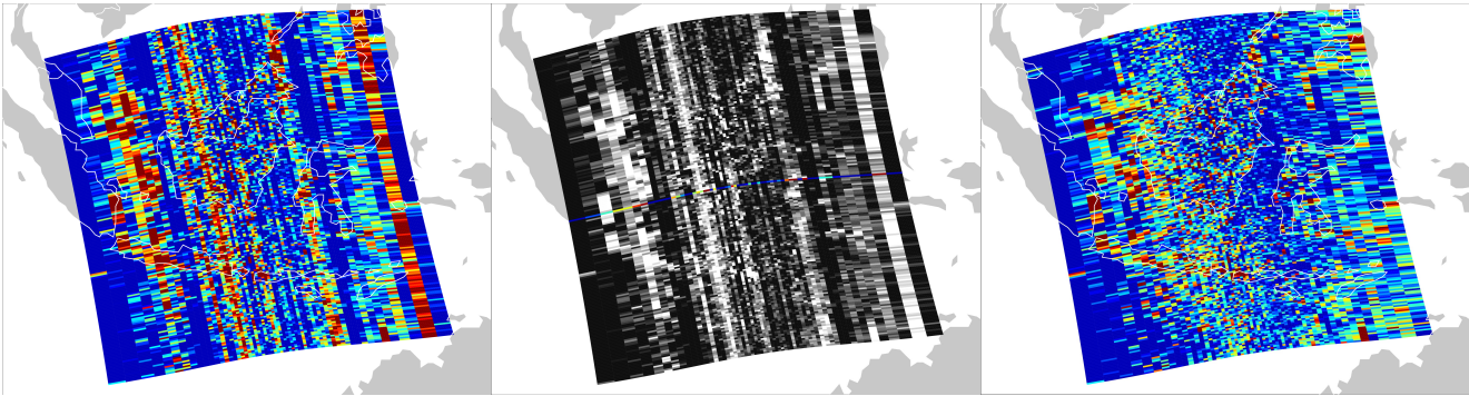
Figure 4: Cross-track smoothing of HCHO columns. Left: Columns as provided in the ColumnAmount data field. Center: The to-be-destriped center swath line (color) and the 200 surrounding swath lines (b&w) that are averaged; see Figure 5 for details on the smoothing. Right: smoothed columns as provided in the ColumnAmountDestriped data field.
